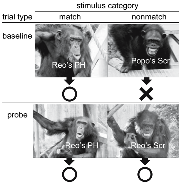
Fig. 3. Examples of the stimulus pairs in baseline and probe trials. Sample vocalization is Reo's pant hoot for both cases. In baseline trials, the vocal-individuality cues and/or the vocalization-type cues were valid for making correct responses. In probe trials, both the match and nonmatch stimuli depicted the sample individual, and responses to either were rewarded
