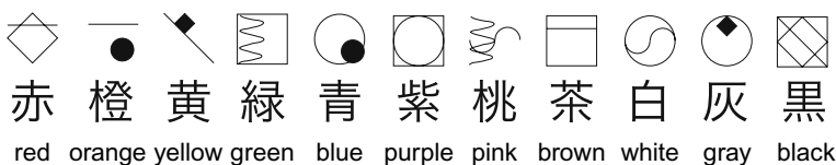
Fig. 1. Lexigrams ( top ) and kanji characters ( middle ) for 11 color names acquired by the chimpanzees
