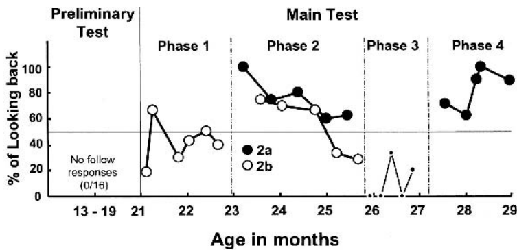
Fig. 6. The percentage of "looking back" responses in the distant-point condition as a function of session and the subject's age. (Okamoto et al. 2004)
