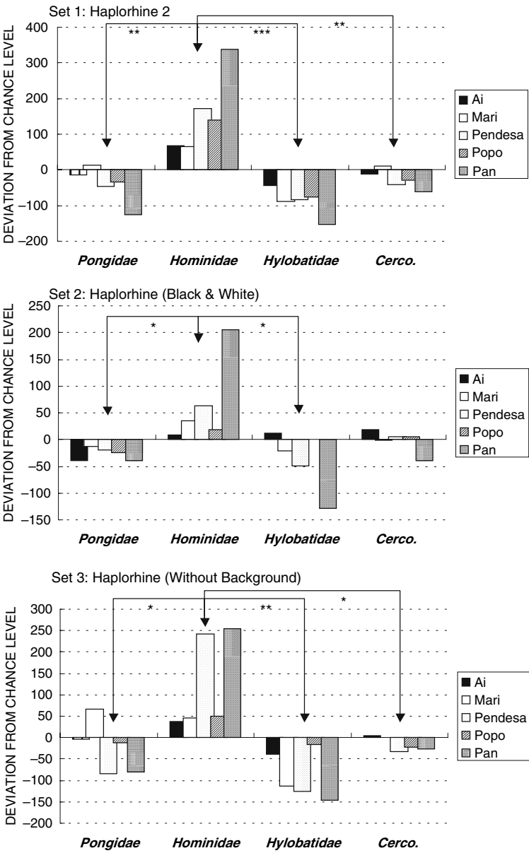
Fig. 6. Standardized score of each category in three stimulus sets. Each bar indicates the score after the subtraction of the chance level score (180) from the raw score. Cerco. on the x -axis indicates the Cercopithecoidea category. Asterisks indicate significant differences between the scores of two categories: *** P < 0.001 , ** P < 0.01 , * P < 0.05
