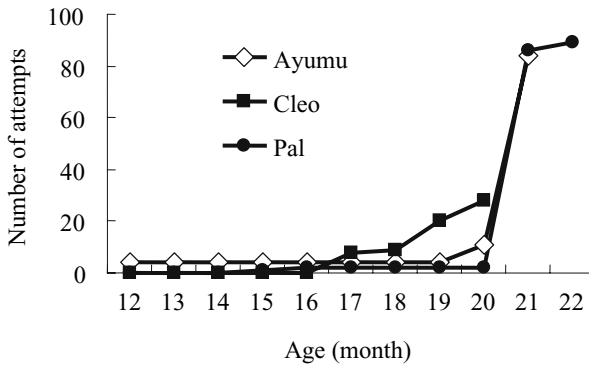
Fig. 6. Cumulative number of attempts before the infants' first success
