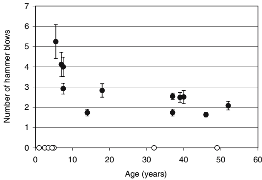
Fig. 9. Average number of hammer blows required to crack a single oil-palm nut as a function of age. Data were collected in 1999. Each filled circle represents the performance of a single individual who was able to crack nuts; open circles show age distribution of individuals who were never seen to succeed at cracking in 1999. Ages of oldest individuals are estimates. Error bars are standard errors of the mean
