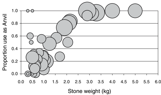
Fig. 6. Use of stones provided at the outdoor laboratory as hammer and anvil as a function of weight. Each circle represents a single stone, with the diameter of the circles corresponding to the relative frequencies with which the stones were used (the smallest circles indicate a single use; the largest represents 35 uses). Height on the y -axis corresponds to the ratio of use of the stone as anvil; i.e., 1 = exclusive use as anvil, 0 = exclusive use as hammer
