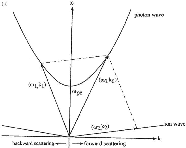
Figure 6.1. Schematic description in the \omega - k space of the conservation laws given in equations (6.5), taking into account the dispersion relations (6.1), (6.2) and (6.3) for (a) decay instability, (b) stimulated Raman instability and (c) stimulated Brillouin instability.
