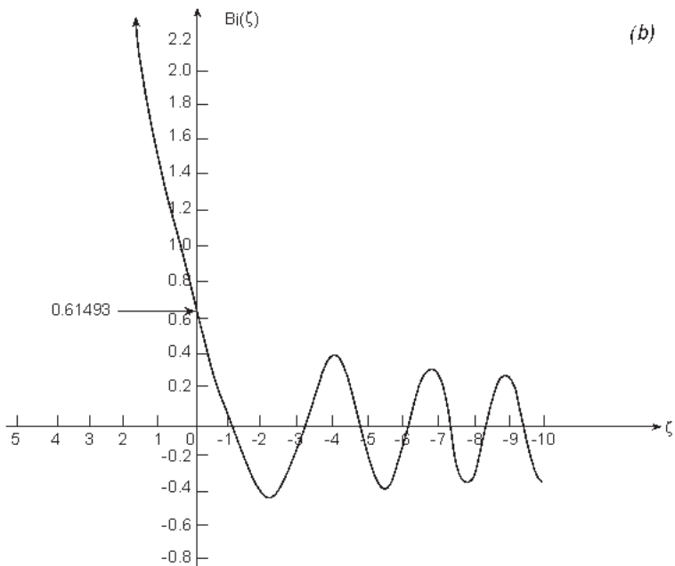
Figure 5.3. The Airy functions Ai , its derivative and Bi .
