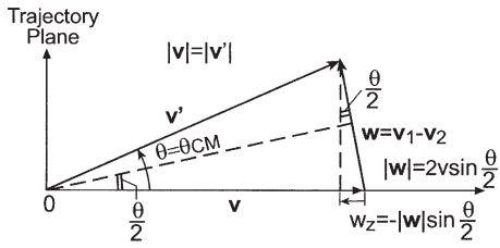
Centre of mass (CM) frame
