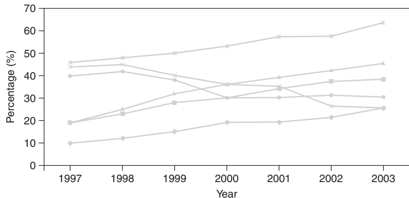
Figure 15.15 The percentage recycling of glass, aluminum and PET in the European Union and the United States (◆ PET in EU, ▲ aluminum in EU, * glass in EU, ■ PET in the USA, X aluminum in the USA and ● glass in the USA) (adapted from http://container-recycling.org/aluminrate/gaphs.thm , http://europa.eu.int/lib/ )
