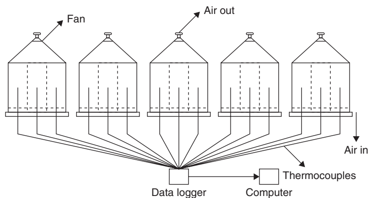
Figure 6.10 Vertical composting system consisting of five piles (adapted from Kulkul and Yaldiz, 2004)
