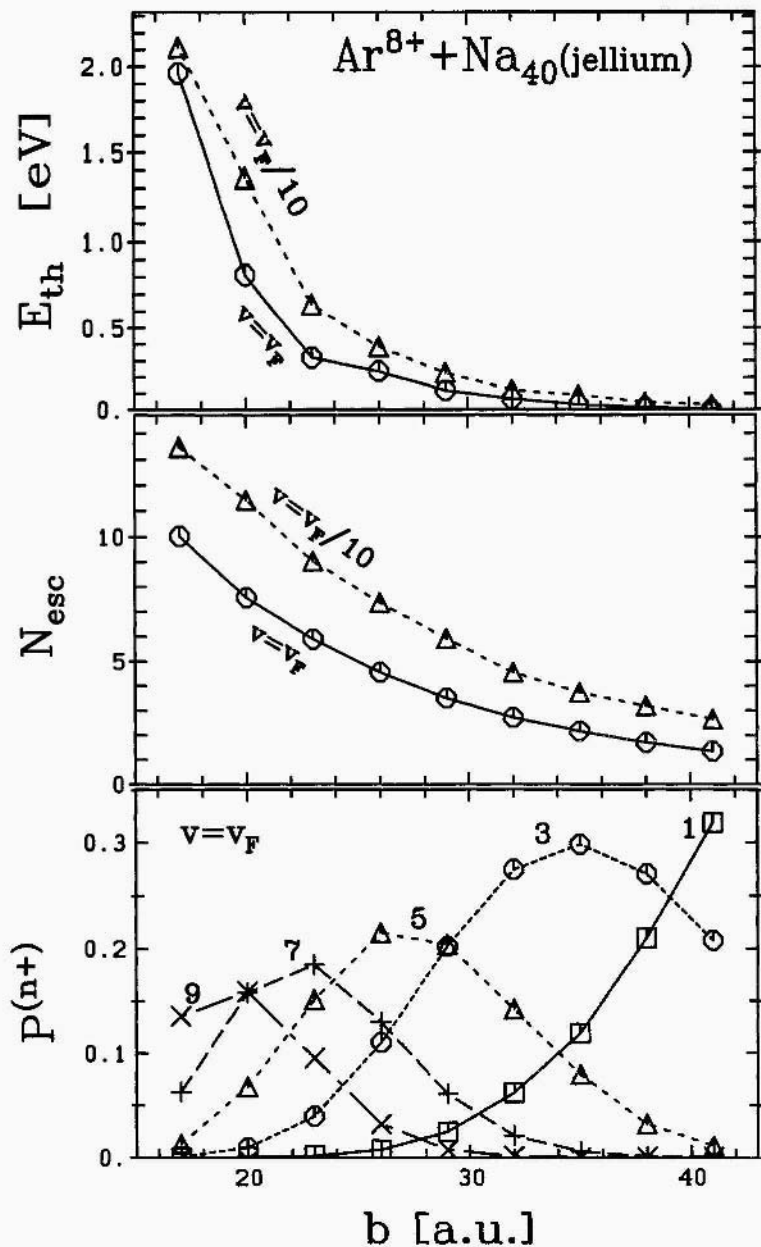
Figure 4. Trends with impact parameter for the asymptotic values of basic observables for a collision of an Ar^{8+} projectile on a Na_{40} cluster at two projectile velocities, as indicated. The upper panel shows the excitation energy, the middle panel the number of escaping electrons and the lower panel displays ionization probabilities in the case of v = v_F velocity. All quantities are plotted as a function of impact parameters. Ionic background is treated in the jellium approximation.
