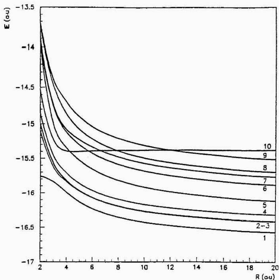
Figure 5 Adiabatic potential energy curves for the ^2\Sigma states of BHe^{4+} 1-2. \Sigma states dissociating to \{ B^{3+}(1s2s)^{13}S + He^+(1s) \} 3-4, \Sigma states dissociating to \{ B^{3+}(1s2p)^{13}P + He^+(1s) \} 5, \Sigma state dissociating to \{ B^{2+}(1s2s^2)S + He^{2+} \} ; 6-7, \Sigma states dissociating to \{ B^{2+}(1s2s2p)^2P + He^{2+} \} ; 8, \Sigma state dissociating to \{ B^{2+}(1s2p^2)D + He^{2+} \} ; 9, \Sigma state dissociating to \{ B^{2+}(1s2p^2)S + He^{2+} \} ; 10, \Sigma state dissociating to \{ B^{4+}(1s) + He(1s^2) \} .
