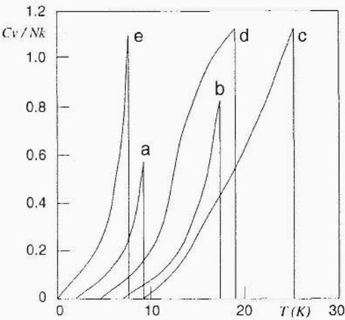
Figure 9. Theoretical heat capacity as a function of doping. (The p values are a = 0.98 , b = 0.97 , c = 0.95 , d = 0.92 , e = 0.9 ).
