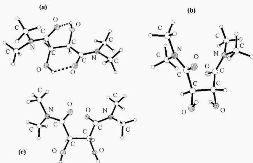
Figure 4 Structures of (R,R)-tartaric acid N,N,N',N' -tetramethyl diamide: (a) lowest-energy conformer for isolated molecule; (b) lowest-energy. conformer in aqueous solution; (c) cry stal structure. Fig. (a) adapted from ref. 22; fig. (c) adapted from ref. 29.
