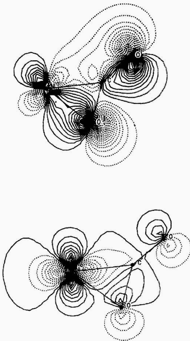
Figure 5. B3LYP 6a' (up) and 7a' (down) molecular orbitals of 1A'1^2C,0 of the NiCO 2 complex. Dark shadings represent positive coefficients (cutoff=0.425, step=0.025)
