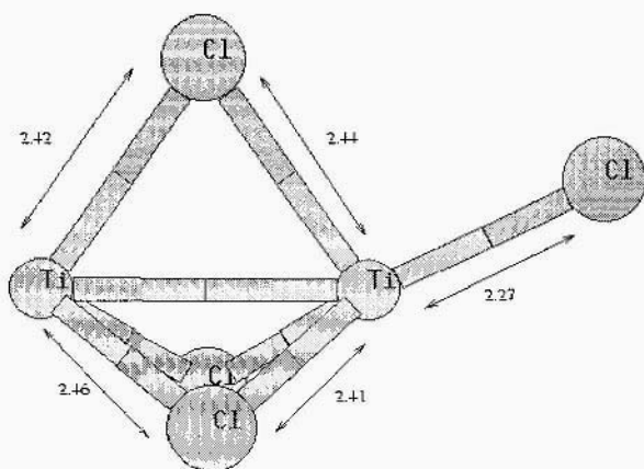
Figure 9a. Structure of (\text{TiCl}_2)_2 .
