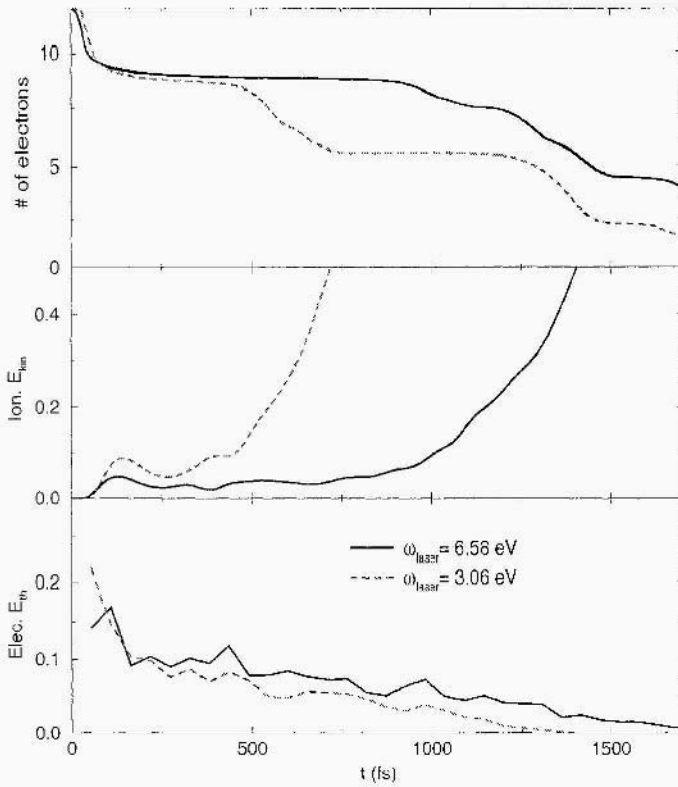
Figure 5. Time evolution of electron number N_{\text{el}} (upper panel), ionic kinetic energy E_{\text{kin,ion}} (middle, in Ry), and thermal energy of the electrons E_{\text{th,el}} (lower panel, in Ry). See [13] for the definition of the electronic excitation energy (lower panel) used in this calculation. From [13].
