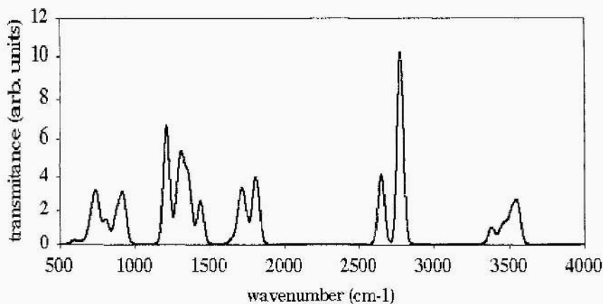
Figure 3. Calculated infrared spectrum of the monodentate [\text{Co(III)(NH}_3)_3\text{CO}_3]^{2+} complex .
