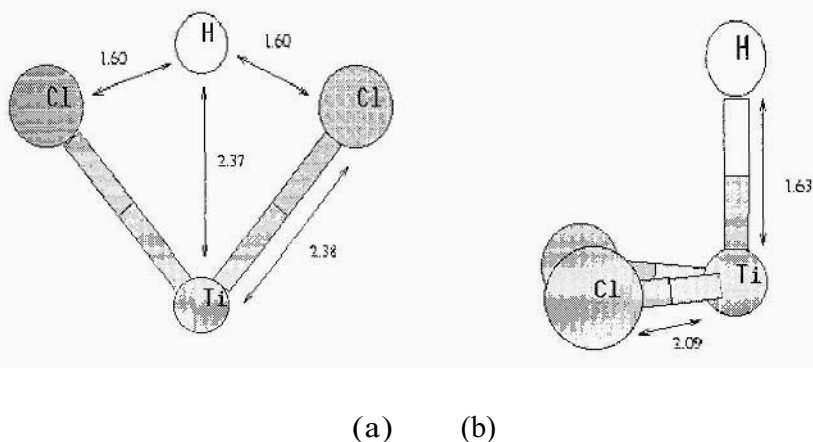
Figure 7. Structures of the protonated \text{TiCl}_2 . The triplet state (a) is more stable than the singlet state (b) by 39.7 kcal/mol.
