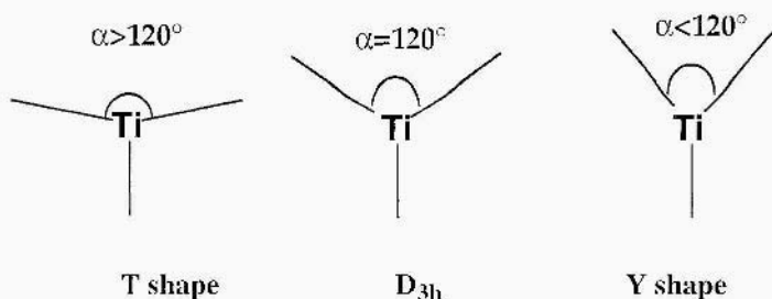
Figure 4. For \text{TiH}_3^- , the ^3B_1 state has a T geometry ( \alpha=123.4^\circ and one \text{TiH} bond is smaller than the other two, 2.020 Å vs 2.011 Å), the ^3A_2 state has a Y geometry ( \alpha=114.7^\circ and one \text{TiH} bond is longer than the other two, 2.059 Å vs 2.059 Å)
