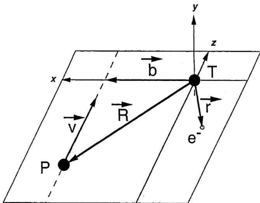
Figure 1. Collision system and coordinate frame: T and P represent respectively target and projectile centers; the impact velocity \vec{v} is parallel to the z -axis and the impact parameter \vec{b} to the x -axis. \vec{r} and \vec{R} are the respective positions of the electron and the projectile relatively to the target.
