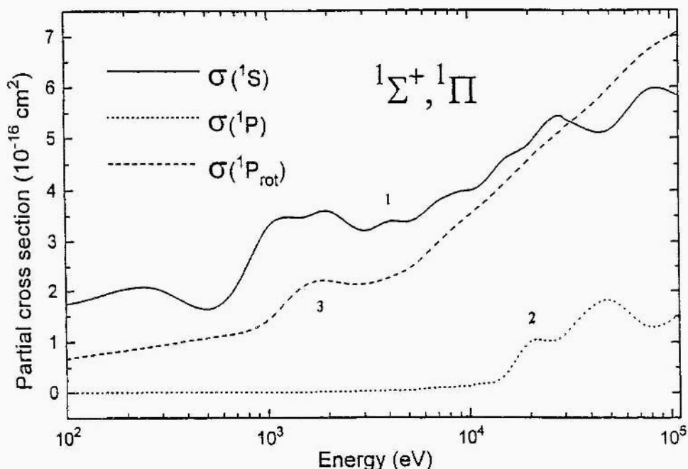
Figure 2. Partial charge-transfer cross sections for the ^1\Sigma^+ and ^1\Pi states of BH_2^+ as a function of incident-ion energy. The notations are the same as in the main text.
