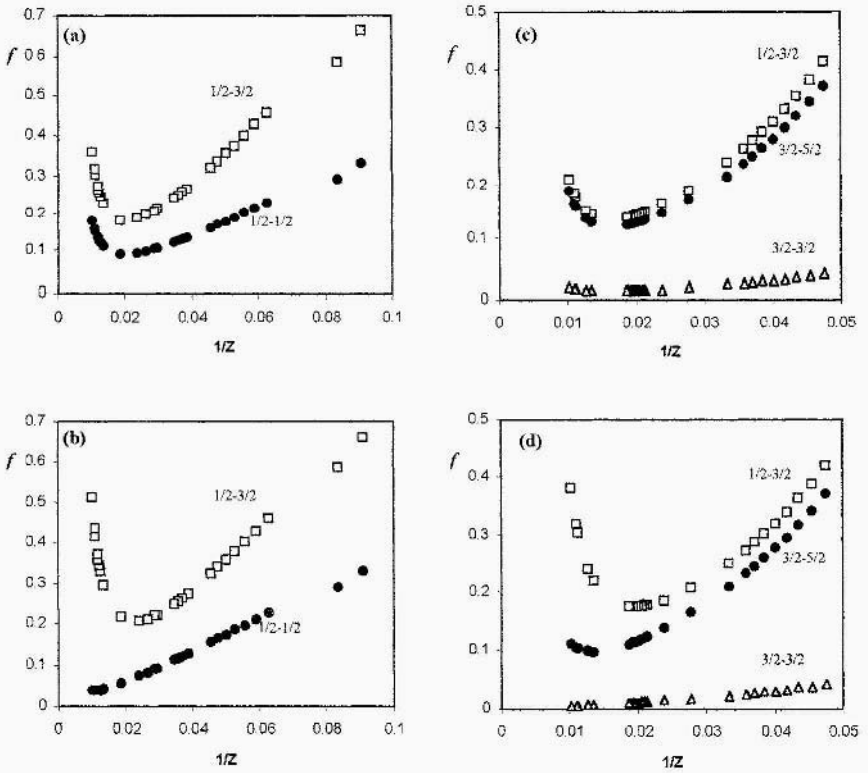
Figure 1. Systematic trends of the fine-structure QDO and RQDO. (a) and (b), respectively, oscillator strengths for the 3s\ 2S - 3p\ 2P^\circ transitions. Systematic trends of the fine-structure QDO and RQDO oscillator strengths for the 3p\ 2P^\circ - 3d\ 2D transitions, (c) and (d) respectively, in the sodium isoelectronic sequence [13].
