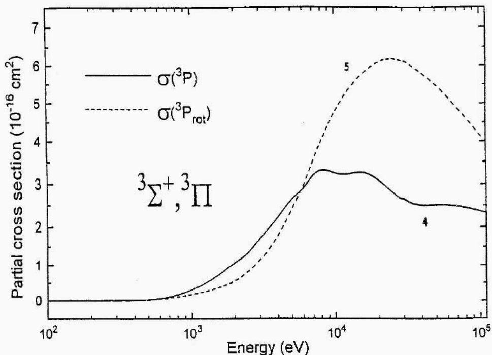
Figure 3. Partial charge-transfer cross sections for the ^3\Sigma^+ and ^3\Pi states of \text{BH}^{2+} as a function of incident-ion energy. The notations are the same as in the main text.
