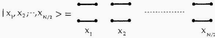
Figure 6. The all-resononstate |x_1, x_2, \dots, x_{N/2}\rangle in a two-leg ladder.
