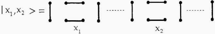
Figure 5. A generic two-resonon state |x_1, x_2\rangle in a two-leg ladder.
