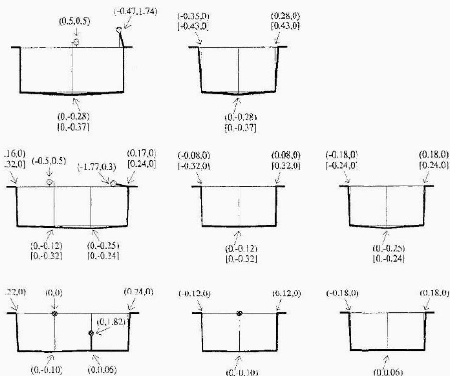
Figure 2. Equilibrium geometries for the three dissociated configurations. From top to bottom and from left to right, the following vertical sections are considered: H\alpha , in a plane through O(\alpha) and Mg(2) ; and another through Mg(1) and Mg(2) ; T\alpha , in a plane through O(\alpha) and Mg(2) ; and in two planes orthogonal to this one, through Mg(2) and O(\beta) ; respectively; T\beta , in the same planes as in the preceding case. Relaxations are given in Bohr with respect to the unperturbed lattice position: the two numbers in parentheses refer to the horizontal and vertical displacement. In square brackets, the corresponding data are provided for the bare defect prior to hydrogen adsorption. The position of H and H^+ is reported with reference to the missing oxygen site, and to the oxygen to which the proton is bound, respectively.
