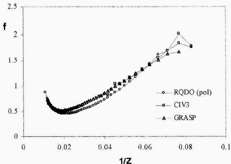
Figure 2 Systematic trends of the oscillator strengths of the 3s^2\ ^1S_0 - 3s3p\ ^1P^1_0 transitions in the magnesium isoelectronic sequence. RQDO (pol) are the core-polarisation-corrected RQDO f -values. Both CIV3 and GRASP f -values correspond to the length form of the transition integral
