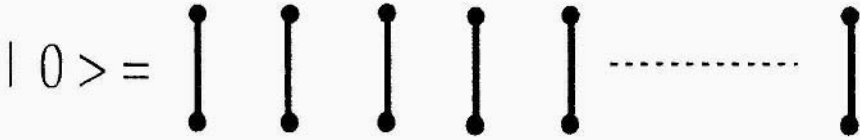
Figure 3. The zero-resonon state |0\rangle in a two-leg ladder. It is made of all vertical rung singlets. It is the reference state in the strong coupling limit J' \gg J .
