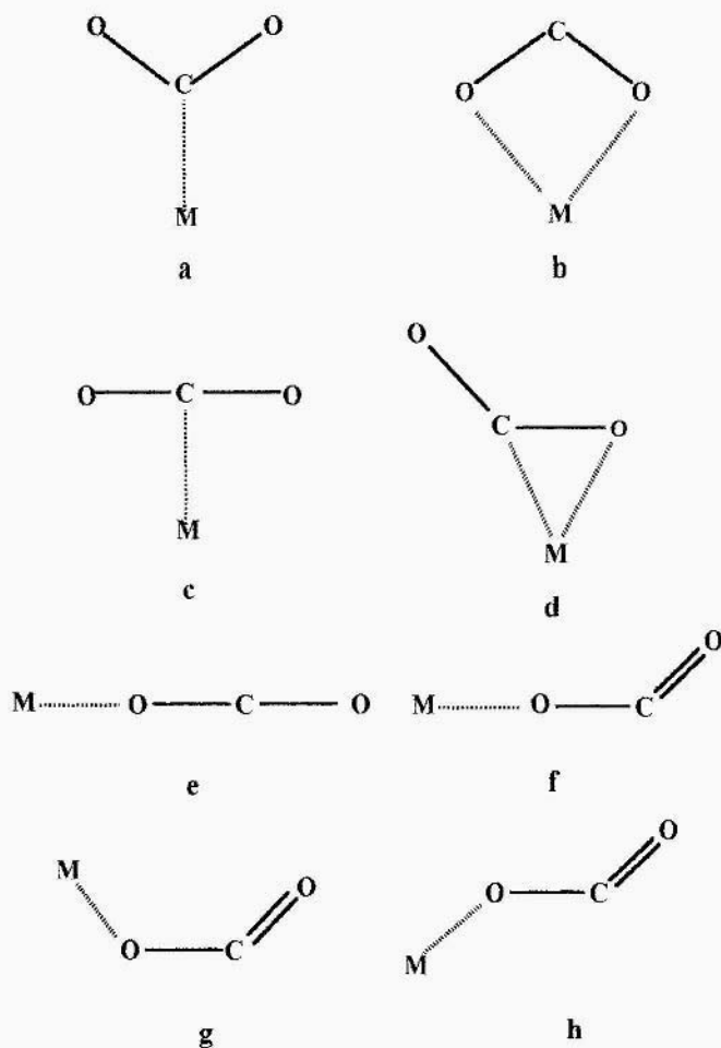
Figure 1. Possible metal-CO 2 coordination modes used as starting points in the geometry optimisation.
