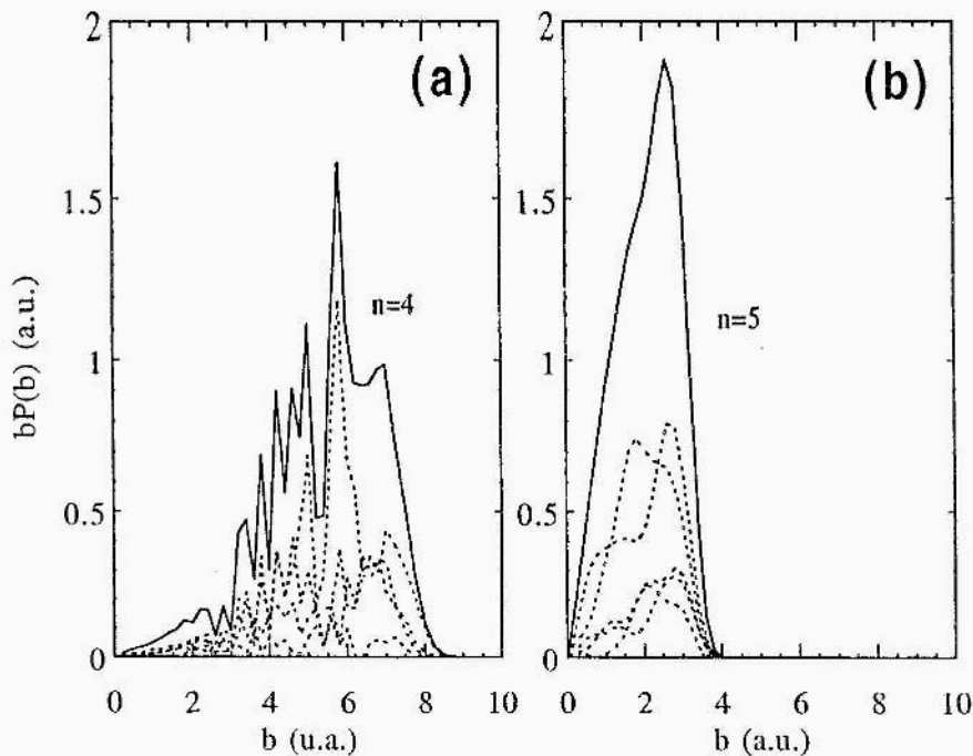
Figure 4. The reduced probability bP_{i \rightarrow f}^v(b) of electron capture in (a) n=4 and (b) n=5 C^{5+} atomic levels from H(1s), at collision energy of 0.1 keV/u ( v=0.06 a.u.). Full lines: total capture to n levels; dotted lines: nl sublevels capture details.
