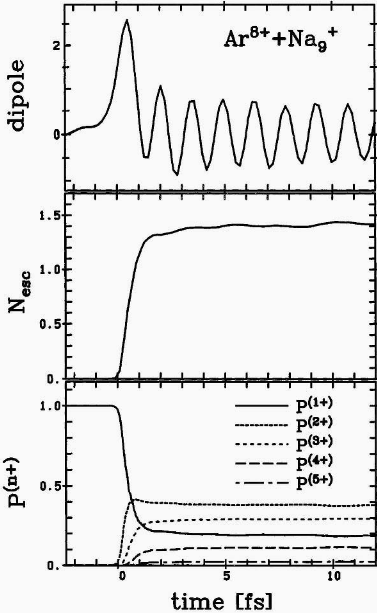
Figure 3. Example of a typical response of the electron cloud for the collision of \text{Ar}^{8+} with velocity v = 50 a_0/\text{fs} = 2 u_F on \text{Na}_9^+ at impact parameter b = 22 a_0 . We show the dipole moment (upper part), the total number of escaped electrons (middle part) and ionization probabilities P(n+) (lower part) as a function of time. Ionic background is treated in the soft jellium approximation. From [32].
