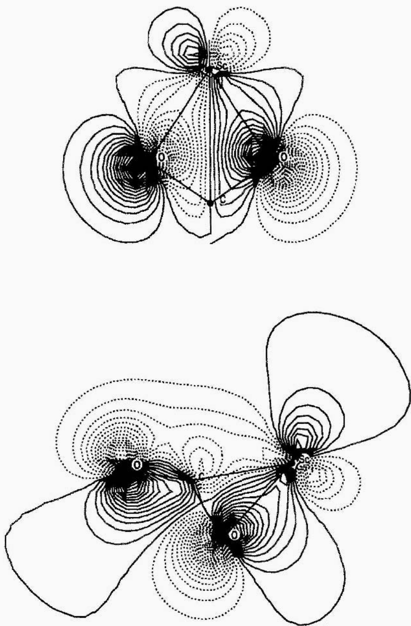
Figure 3. B3LYP 4b 2 and 9a 1 molecular orbitals of \eta^2\text{O}_2\text{O} and \eta^2\text{C}_3\text{O} ScCO 2 isomers, respectively. Dark shading represents positive coefficients (cutoff=0.425, step=0.025).
