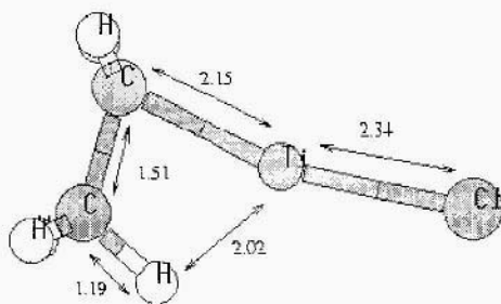
Figure 10. Structure of C1Ti-CH_2-CH_3 obtained from by optimisation of TiHCl-C_2H_4 with a \pi -bonding ethene
