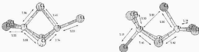
Figure 9, b and c. Structures of (\text{TiCl}_3)_2 and (\text{TiCl}_4)_2 .
