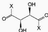
Figure 1. Zig-zag formula of ( R,R )-tartaric acid and its derivatives. X = NH 2 for the diamide and X = N(CH 3 ) 2 for the N,N,N',N' -tetramethyldiamide.
