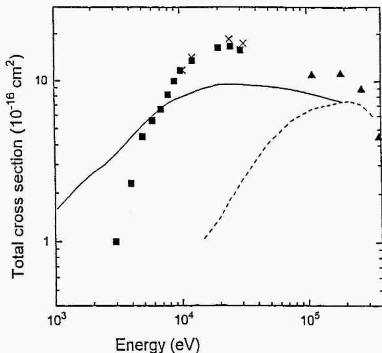
Figure 4. Comparison of our total charge-transfer cross section for B^{2+}/H with previous theoretical calculations and experimental measurements: - - - - \sigma_{tot} (this work); --- Crothers and Todd [8]; Y McCullough et al. [5]; x Crandall et al. [6]; \Delta Goffé et al. [7].
