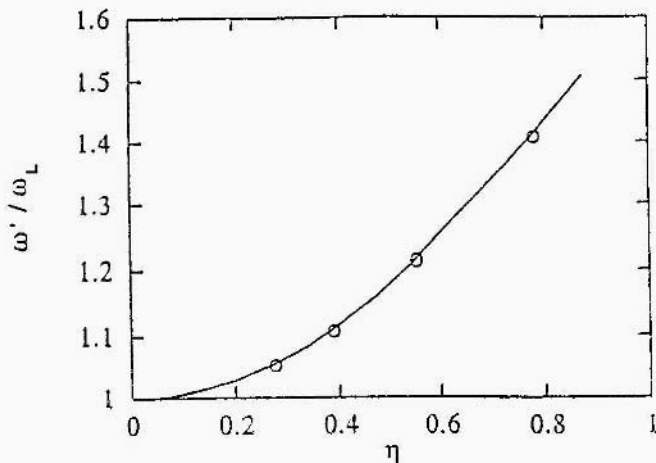
Figure 6. Frequency shift \omega'/\omega_L , Eq. (11), as a function of the relativistic parameter \bar{\pi} = (qF_0\hbar)/(mc\omega_H) , with \omega_H = 10a.u. . The circles indicate the shift deduced from the full time-dependent calculation.
