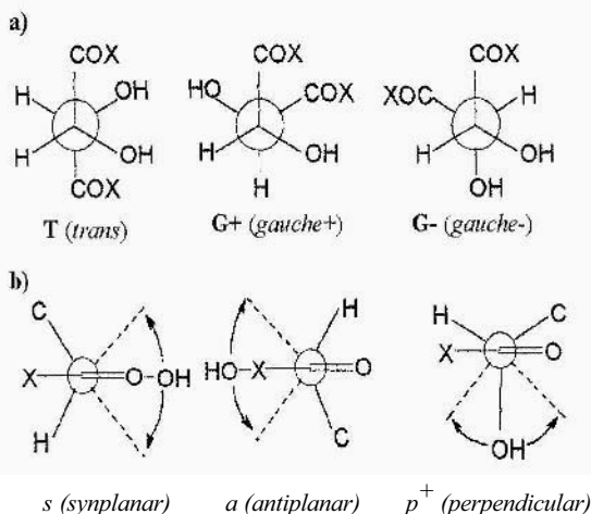
Figure 2. Rotational profiles of (R,R)-tartaric acid and its derivatives (a) Rotation around the C_{sp^3}-C_{sp^3} bond and (b) rotation around the C_{sp^3}-G_{sp^2} bond. X = NH_2 or N(CH_3)_2 .
