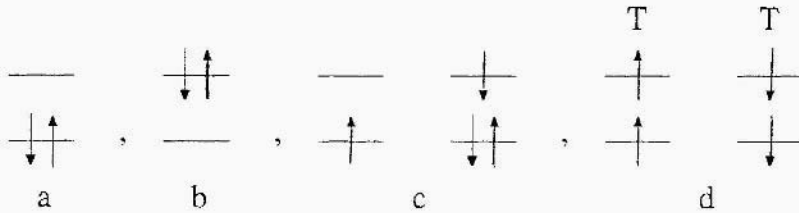
Figure 9. The set of local configurations considered in this work for the dimerized chain; a) the F -LC b) the D -LC c) the Ct1 -LC and d) the TT -LC made by combining two localized triplet symbolized by the T on the figure.
