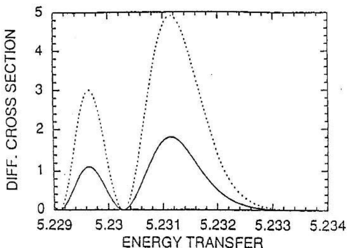
Figure 3. Envelope of the absorption edge part of the differential cross section d\sigma/d\omega scaled in 10^{-14} a.u. as a function of energy transfer scaled in units of 10^5\omega for an electrical field strength of E = 5.89 a.u. or vector potential A = 18769 a.u. . The solid line denotes the result for electrons and the dashed line sketches the result for spinless particles,
