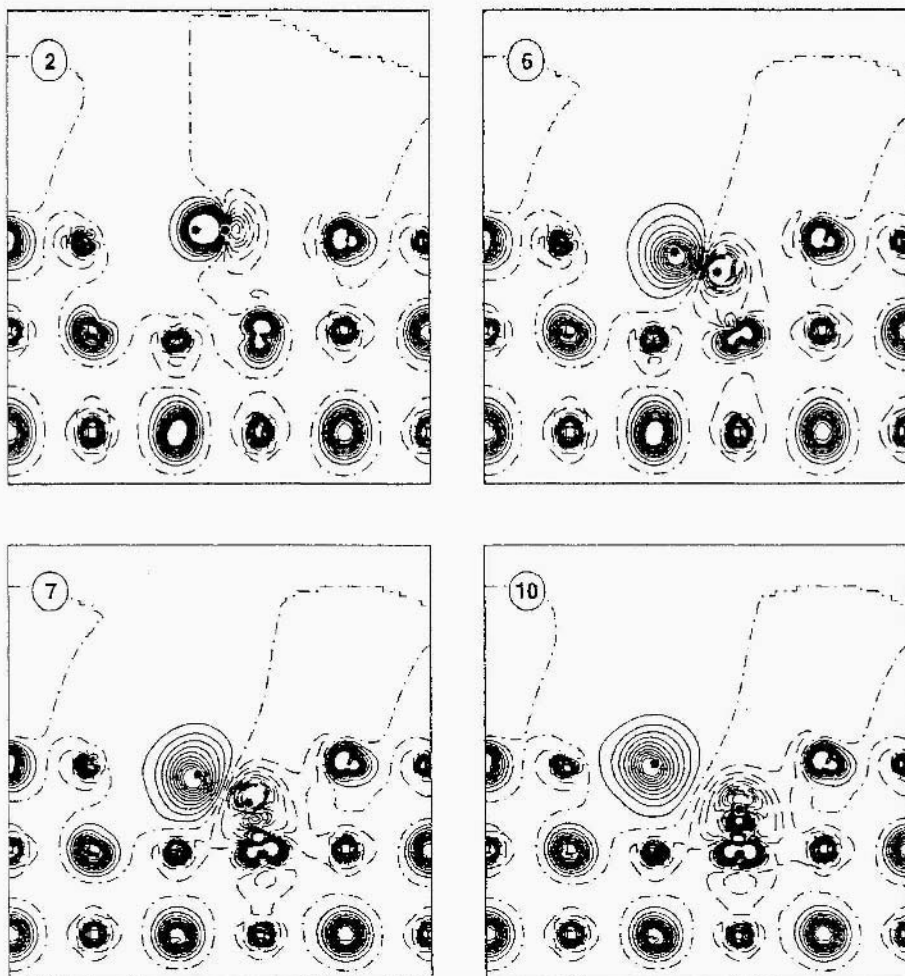
Figure 5. Difference density maps (total minus superposition of isolated species) for different configurations along the reaction path leading to the T\beta configuration. The numbers identifying each plot are as in figure 4. Consecutive iso-difference-density curves differ by 0.005 |e|/\text{Bohr}^3 . The black dots mark the position of the two hydrogen nuclei.
