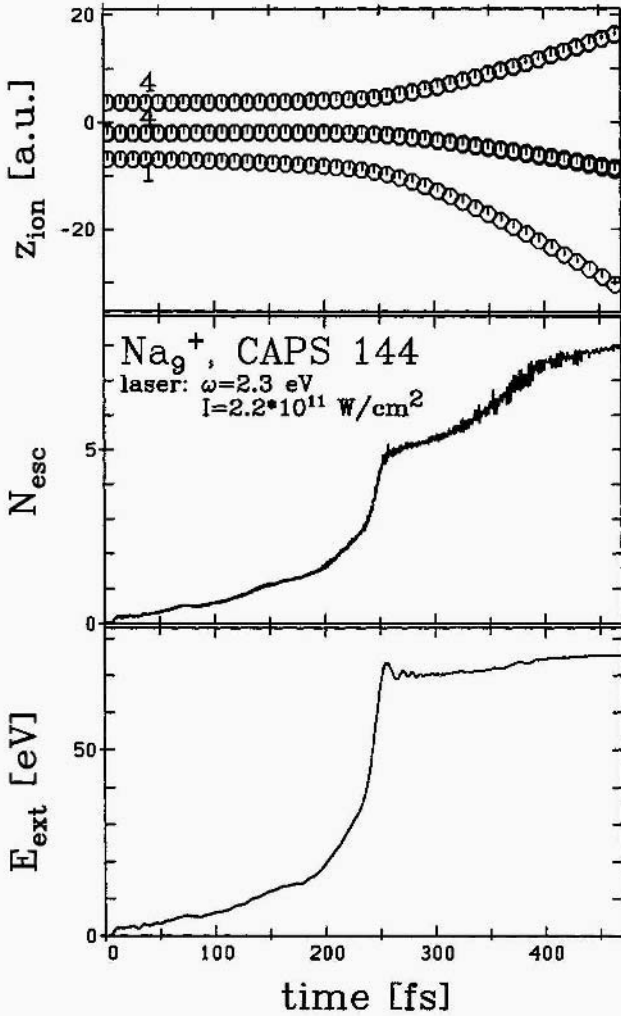
Figure 6. Time evolution of ionic structure and electronic key observables for \text{Na}_9^+ in a laser field with intensity I = 2.2 \times 10^{11} \text{ W/cm}^2 and frequency \omega = 2.3 \text{ eV} . Upper: The z -positions of the 9 ions with multiplicity (arrangement in rings according to CAPS) as indicated. Middle: Number of escaped electrons N_{\text{esc}} . Lower: Energy E_{\text{ext}} absorbed by the cluster from the external laser field. From [35].
