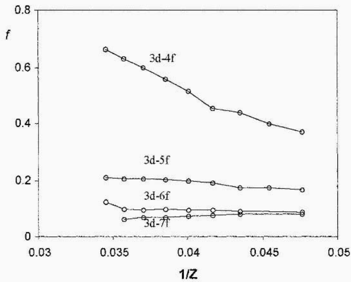
Figure 3. Systematic trends of the RQDO multiplet oscillator strengths of the 3d 2 D- nf 2 F° transitions in the “iron group” potassium-like ions.
