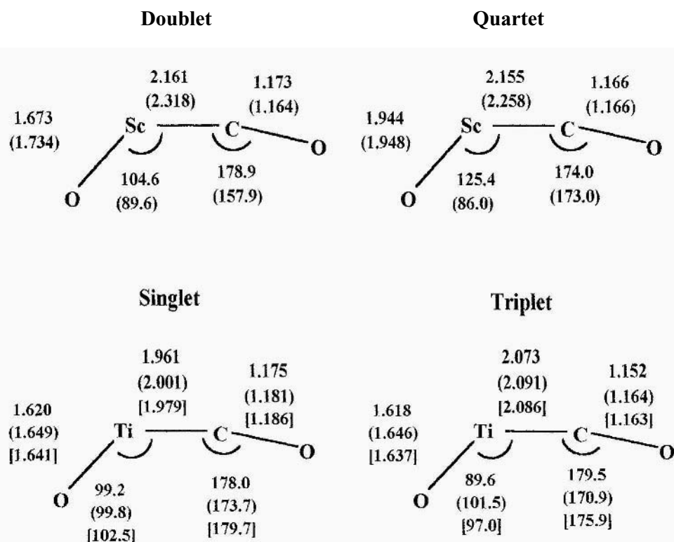
Figure 6. B3LYP, (PWP) and [BP] geometrical parameters for the OScCO and OTiCO systems. Distances are in Å and angles in degrees.
