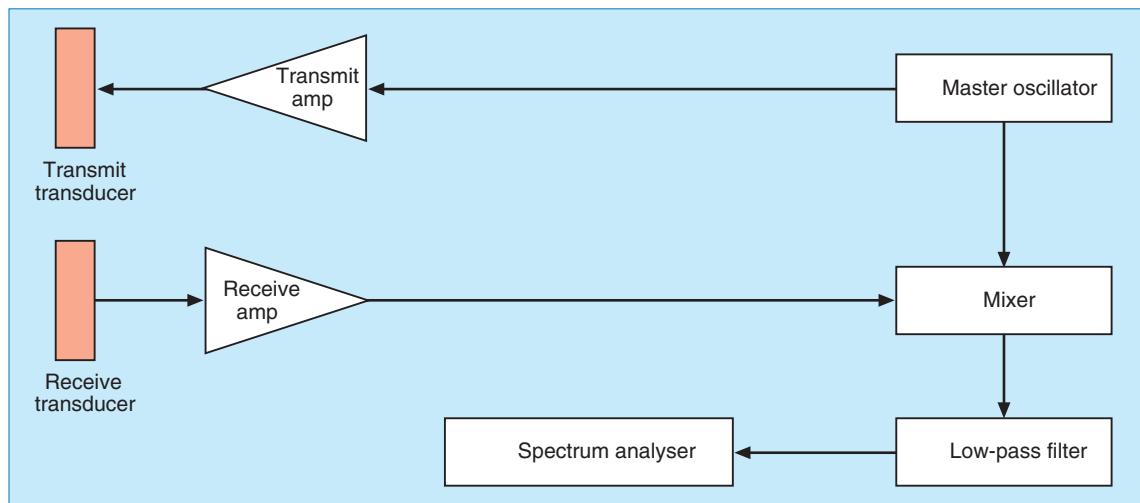
Figure 15.9 Block diagram of a simple continuous wave flowmeter
