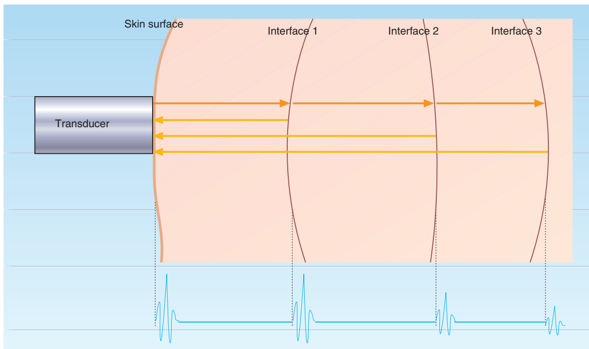
Figure 1.3 Pulse echo principle with multiple reflectors.
