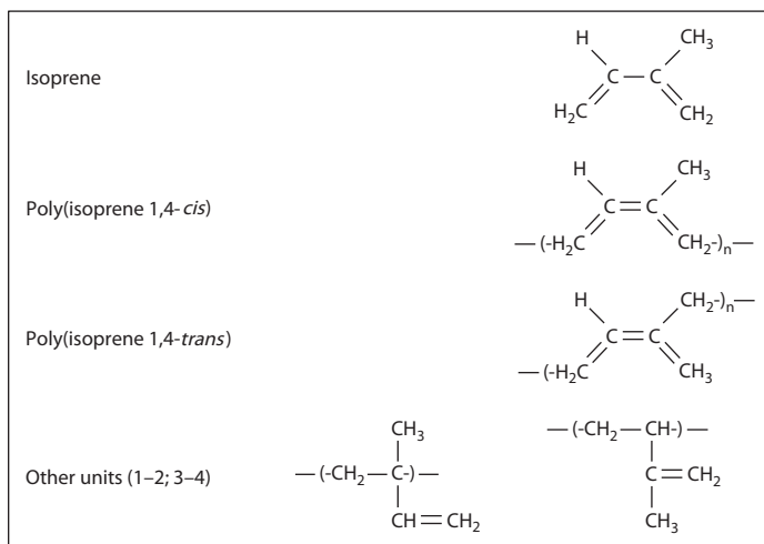
Figure 1.13 Cis-trans isomerism of polyisoprene. The systematic name of isoprene is 1,3-butadiene, 2-methyl. Poly(isoprene 1,4-cis) is the main constituent of natural rubber. Poly(isoprene 1,4-trans) is the main constituent of gutta percha. Vinylic units (1-2) and (3-4) are present in synthetic rubbers.
