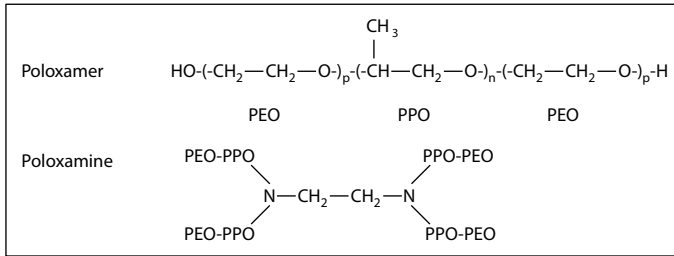
Figure 4.1 Repeating units in poloxamers and poloxamines.
