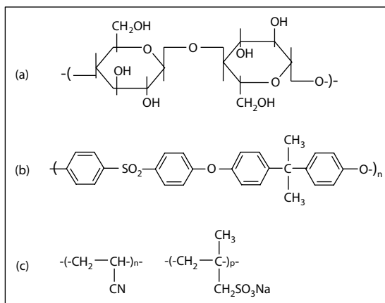
Figure 4.11 Polymeric materials used in haemodialysis membranes: (a) regenerated cellulose (cellophane, Cuprophan ® ) and modified cellulose derivatives in which some OH groups are modified by binding acetyl or diethylaminoethyl (DEAE) groups (in Hemophan ® ); (b) polysulfone; (c) poly (acrylonitrile-co-methallylsulphonate) copolymers (AN69S ® ).
