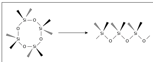
Figure 3.7 Synthesis of poly(dimethylsiloxane) (PDMS) by ring-opening polymerisation.
