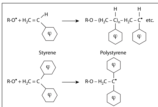
Figure 3.5 Limitation by steric hindrance of polymerisation of some styrene derivatives.
