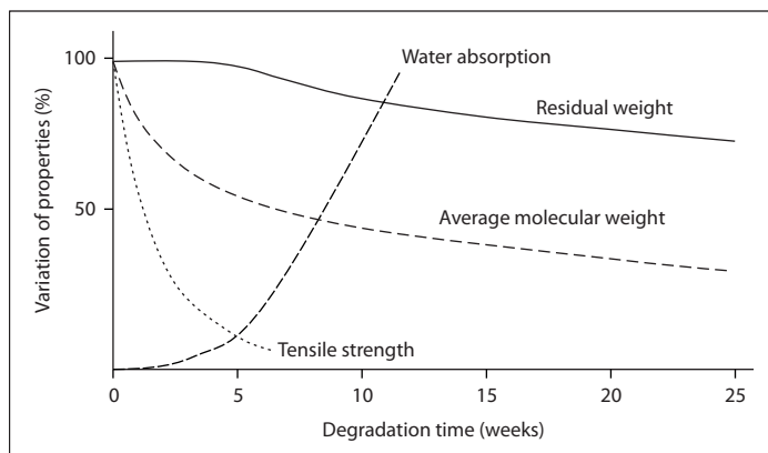
Figure 4.5 Degradation of poly(L,L-lactide) (PLLA) in aqueous medium: variation of several parameters with time.
