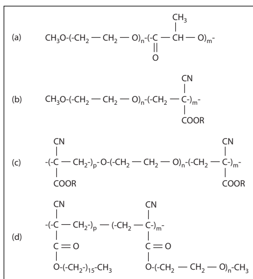
Figure 4.36 Block and graft amphiphilic copolymers leading to core-shell nanoparticles in aqueous solutions: (a) PEO-PLA diblock copolymer, (b) PEO-PACA diblock copolymer, (c) PACA-PEG-PACA triblock copolymer, and (d) Poly[hexadecyl cyanoacrylate-graft-(PEO)-] copolymer.
