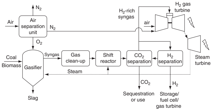
FIGURE 9.22 Layout for a gasification-based system for co-production of hydrogen and electrical power while sequestering CO 2 [51]. Reprinted with permission from Elsevier.
