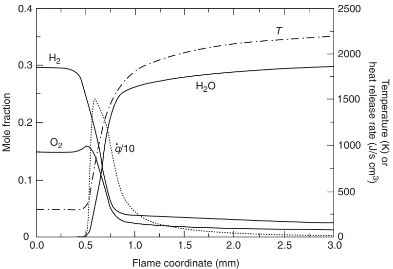
FIGURE 4.11 Composition, temperature, and heat release rate profiles for a stoichiometric \text{H}_2 -air laminar flame at 1 atm and T_0 = 298 \text{ K} .
