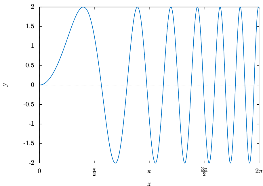
Figure 5.2.6 y = 2 \sin(x^2)
