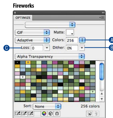
Figure 22-2. GIF optimization options in Photoshop and Fireworks.
