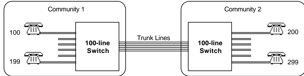
Figure 10.107 A network with two switches.
