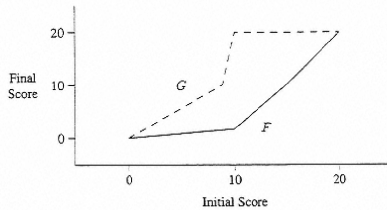
Figure B-1 Sample TAMP Curves
