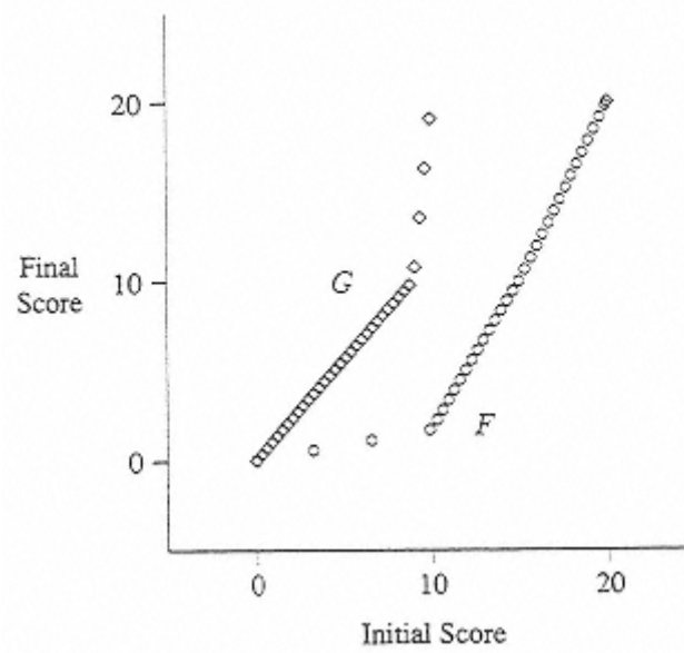
Figure B-2 Tamp Curves Illustrating Simpson's Paradox
