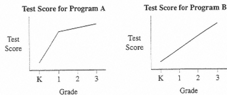
Figure 4-1 Hypothetical Student Growth Curves
