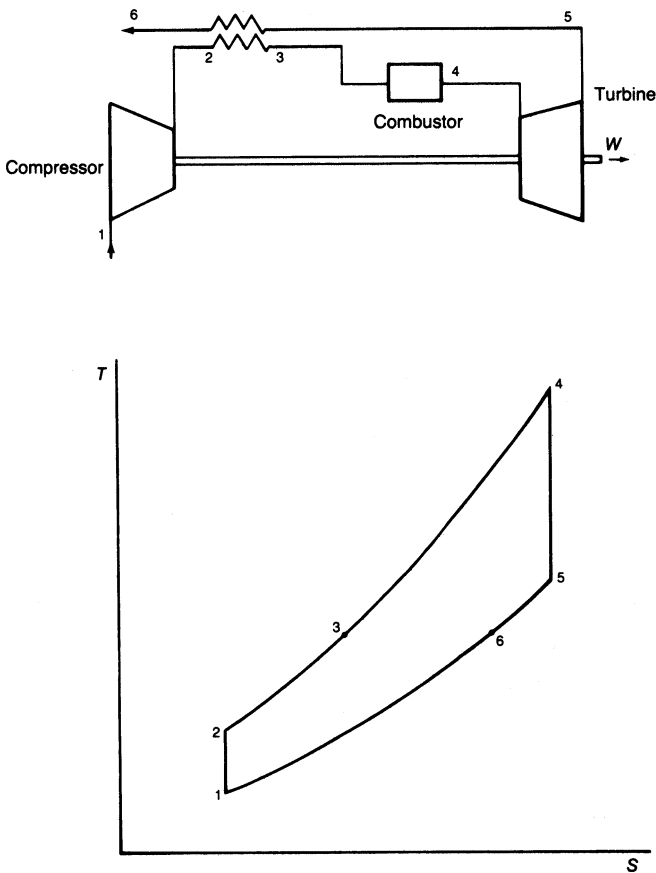
Figure 2-4. The regenerative gas turbine cycle.
