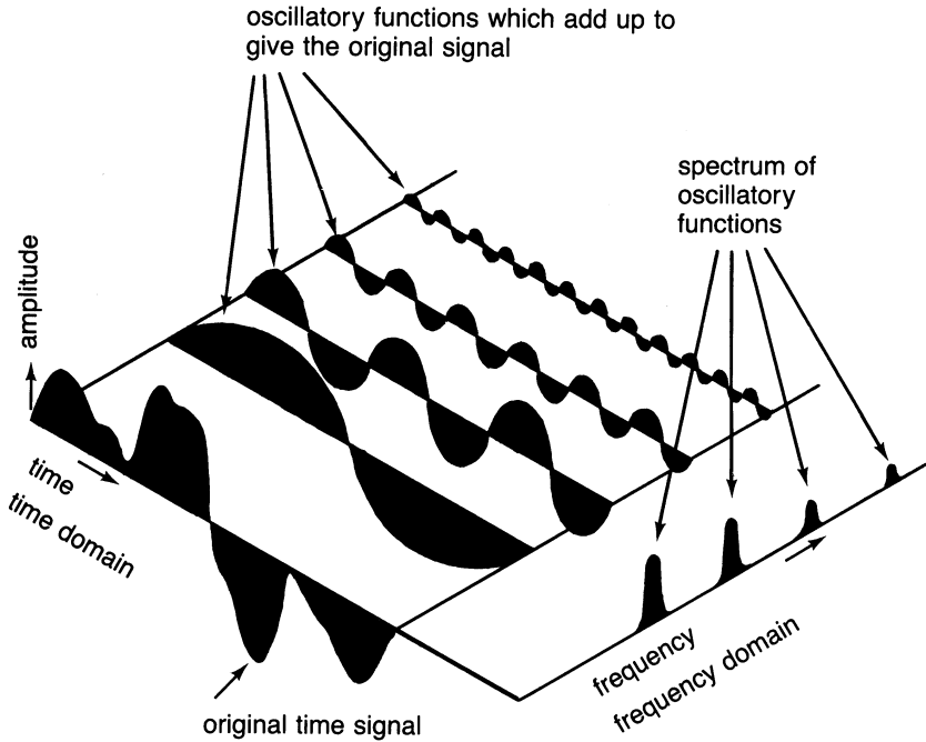
Figure 16-1. Decomposition of a time signal into a sum of oscillatory functions from which a spectrum can be obtained.
