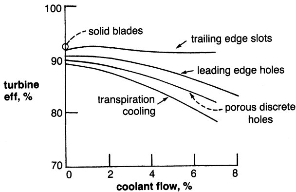
Figure 9-25. The effect of various types of cooling on turbine efficiency.
