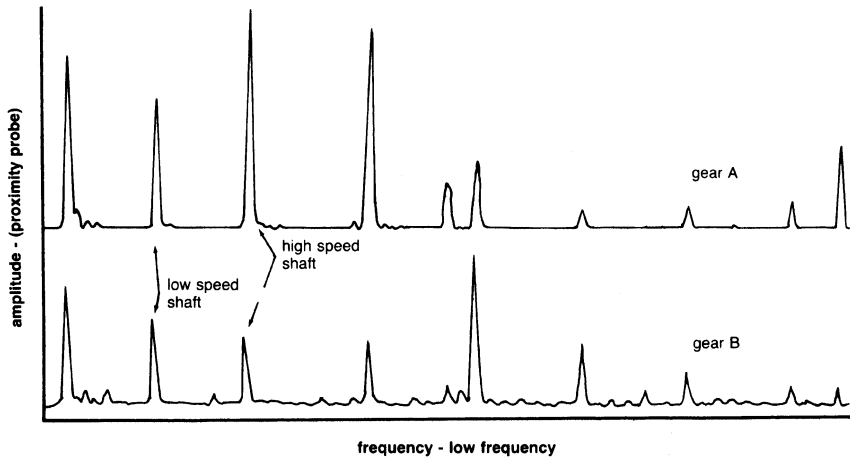
Figure 16-12. Gear box signature (low-frequency end).
