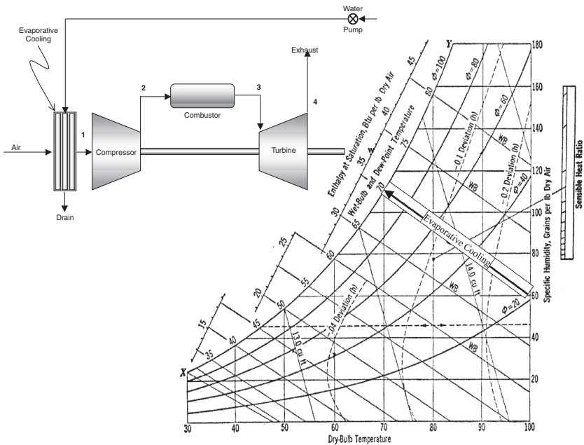
Figure 2-35. Schematic of evaporative cooling in a gas turbine.
