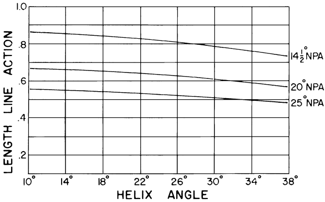
Figure 14-4. Length of line of action change with pressure angle and helix angle. (Courtesy of Lufkin Industries, Inc.)
