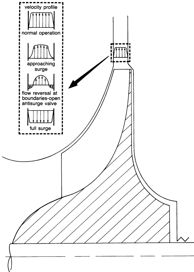
Figure 6-43. Boundary-layer surge prediction technique.
