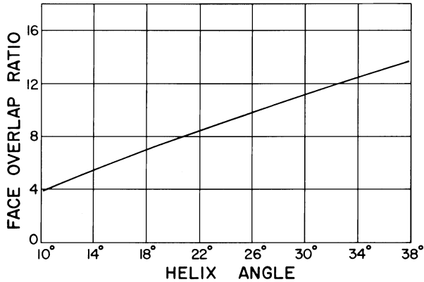
Figure 14-6. Face overlap (contact) ratio variation with helix angle. (Courtesy of Lufkin Industries, Inc.)
