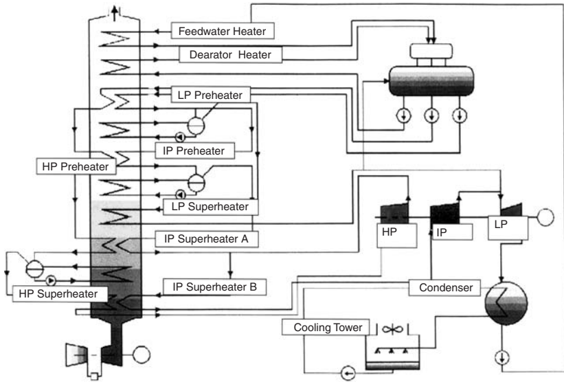
Figure 2-32. A typical large combined cycle power plant HRSG.
