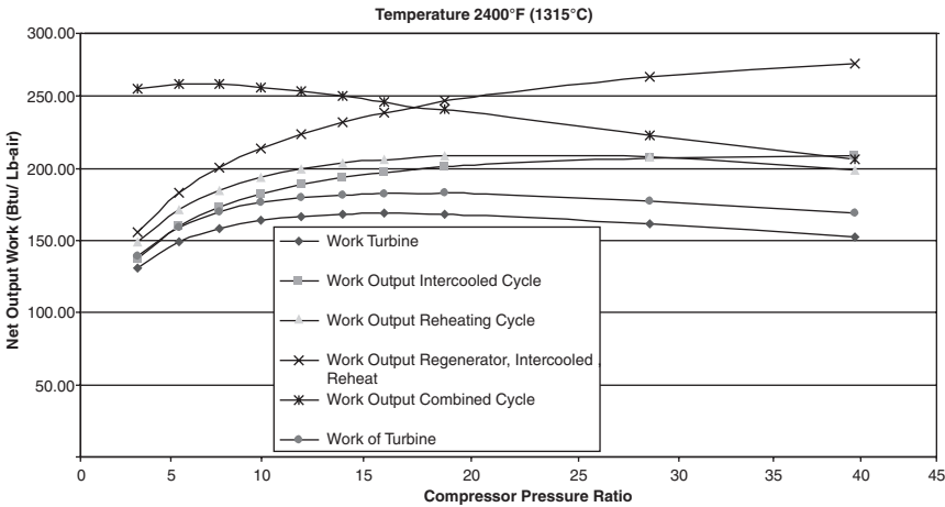
Figure 2-28. Comparison of net work output of various cycles temperature.
