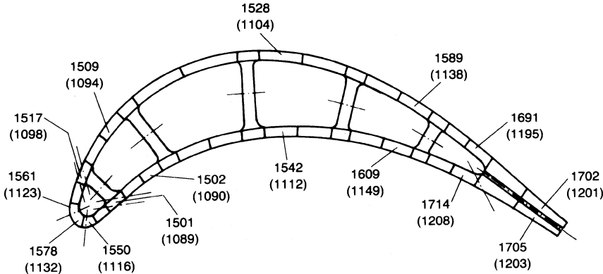
Figure 9-17. Temperature distribution for film convection-cooled design, °F (cooled).
