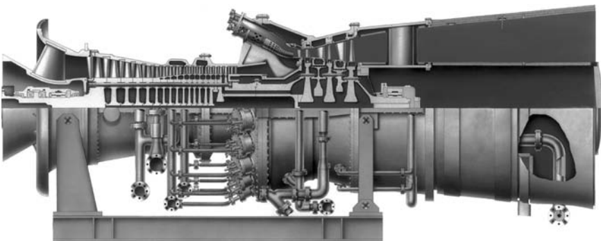
Figure 1-8. A frame-type gas turbine with can-annular combustors. (Courtesy GE Power Systems.)
