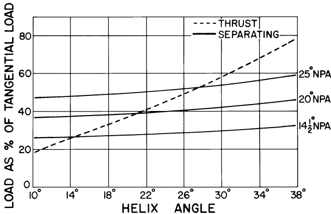
Figure 14-7. Thrust and separating load as a percentage of transmitted tangential load. (Courtesy of Lufkin Industries, Inc.)
