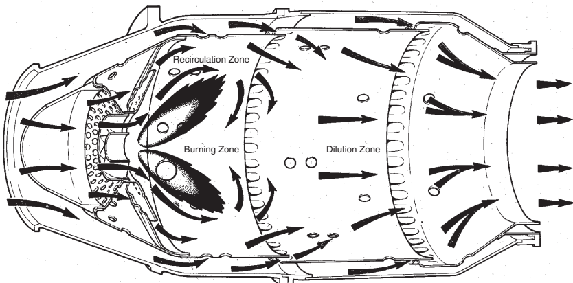
Figure 1-23. A typical combustor can with straight through flow.
