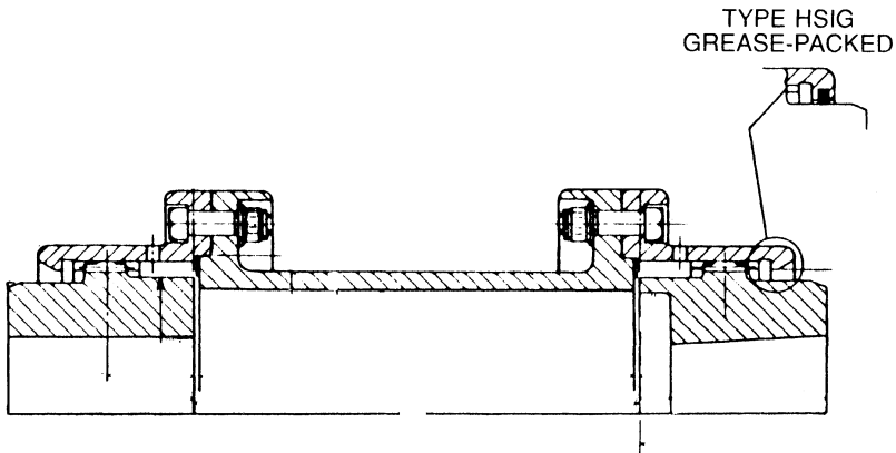
Figure 18-2. Gear coupling (male teeth integral with the hub).
