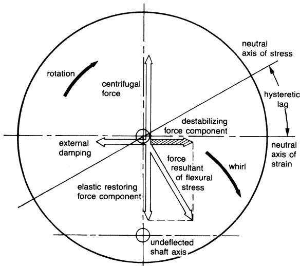
Figure 5-22a. Hysteretic whirl. (Ehrich, F.F., "Identification and Avoidance of Instabilities and Self-Excited Vibrations in Rotating Machinery," Adopted from ASME Paper 72-DE-21, General Electric Co., Aircraft Engine Group, Group Engineering Division, May 11, 1972.)
