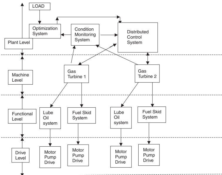
Figure 19-3. Hierarchic levels of automation.
