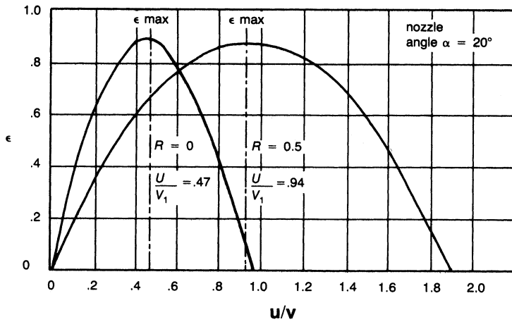
Figure 3-13. Variation of utilization factor with U/V_1 for R = 0 and R = 0.5 . (From Principles of Turbomachinery by Dennis G. Shepherd, © 1956 by Macmillan Publishing Co., Inc.)
