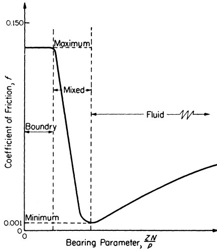
Figure 13-10. Classic ZN/P curve.
