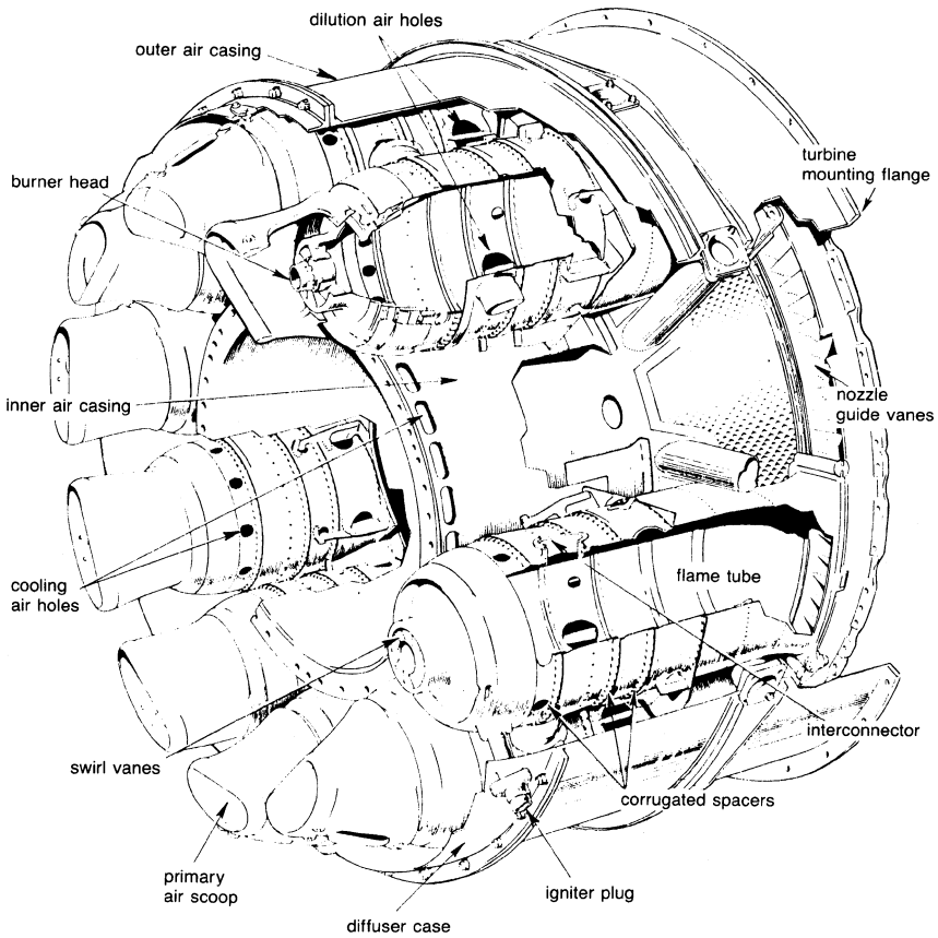
Figure 10-15. “Straight-through” flow-type can-annular combustors. (© Rolls-Royce Limited.)
