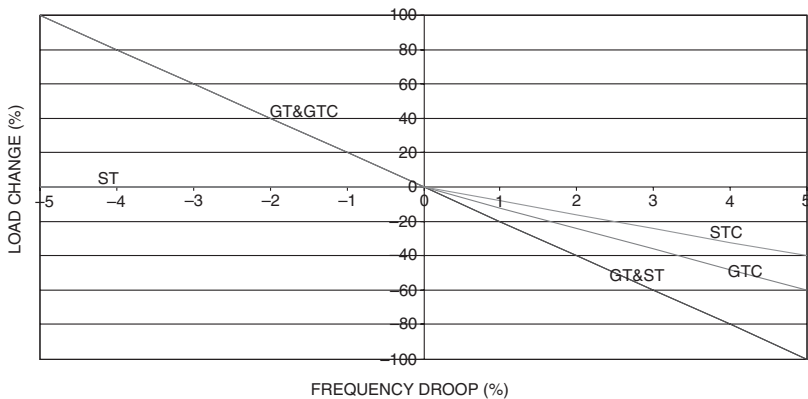
Figure 19-4. Droop curves for Combined Cycle Power Plants.
