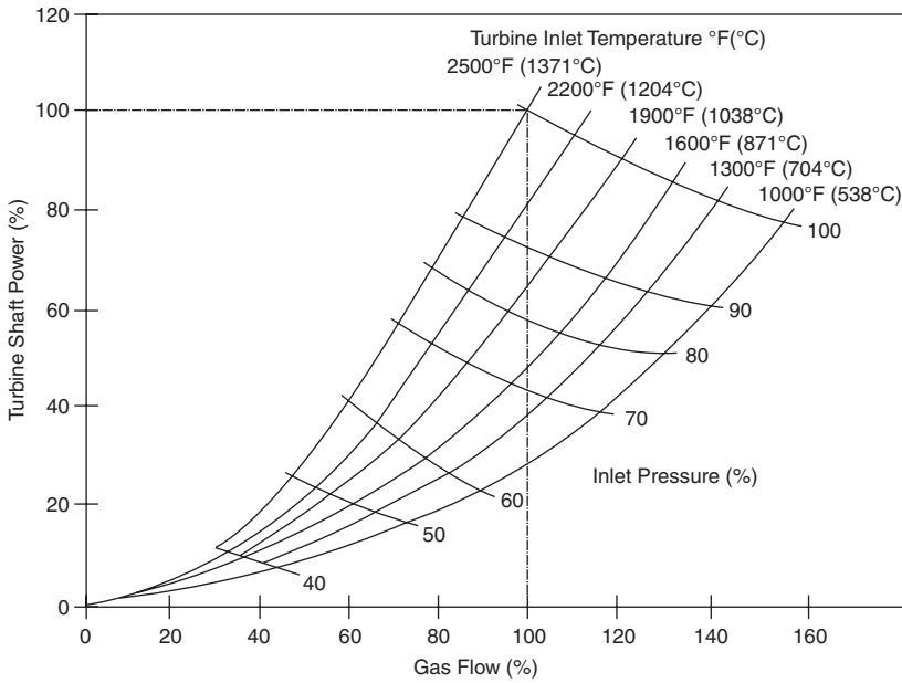
Figure 3-12. Turbine performance map.
