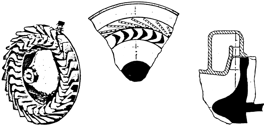
Figure 8-3. Cantilever-type radial-inflow turbine.
