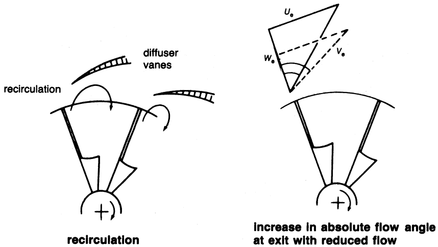
Figure 6-34. Recirculating loss.
