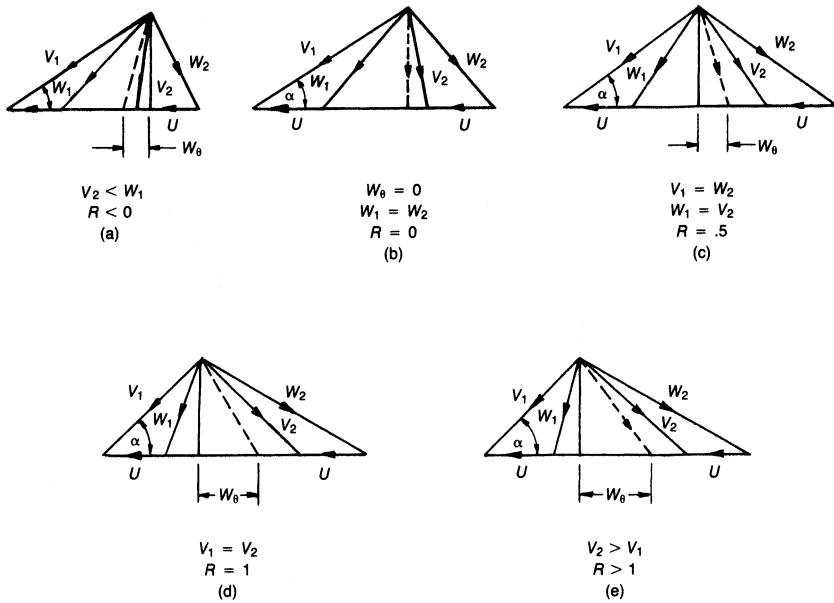
Figure 9-4. Turbine velocity triangles showing the effect of various degrees of reaction.
