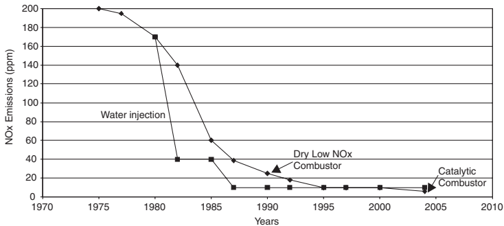
Figure 10-18. Control of gas turbine NO x emissions over the years.
