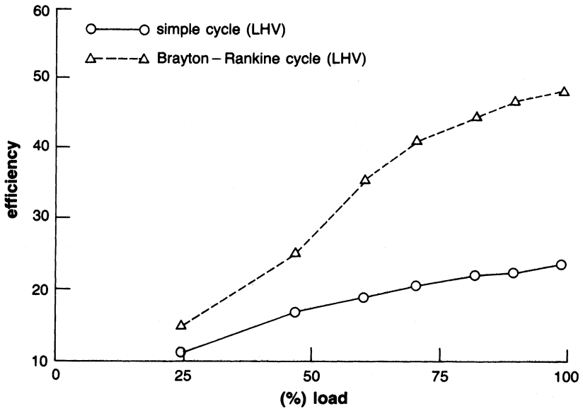
Figure 3-19. Combined cycle and simple cycle efficiency as a function of gas turbine load.
