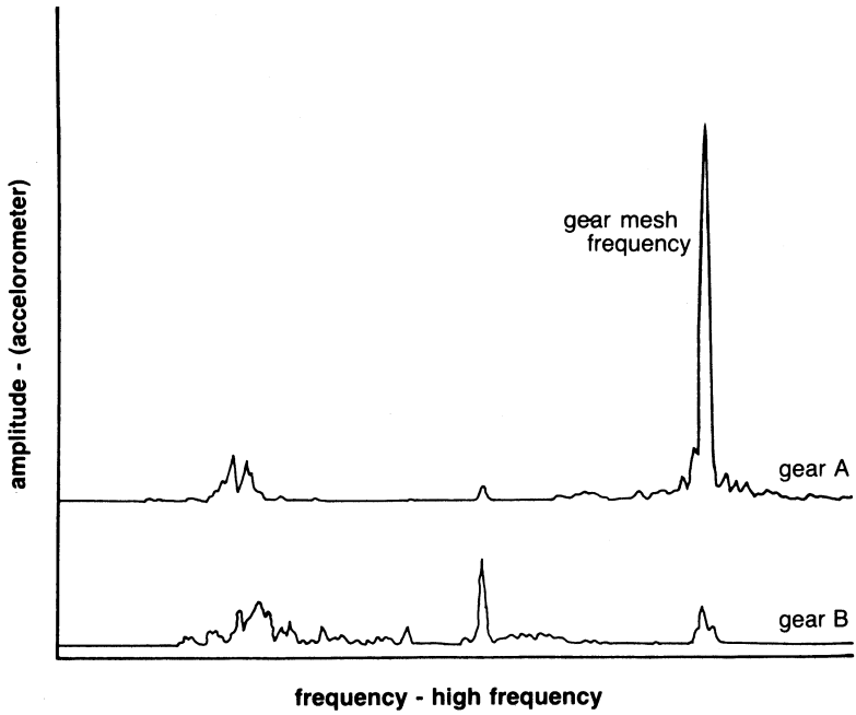
Figure 16-13. Gear box signature (high-frequency end).
