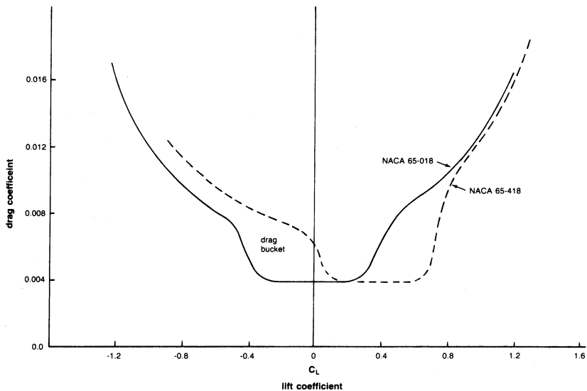
Figure 7-7. NACA measurements of drag coefficients for two laminar airfoils.
