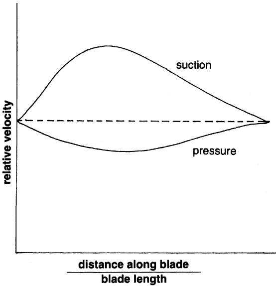
Figure 8-15. Relative velocity distribution of suction and pressure side along the blade length.
