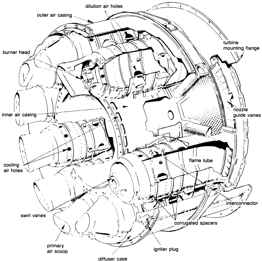
Figure 1-26. Turbo-annular combustion chamber for aircraft-type gas turbines.
