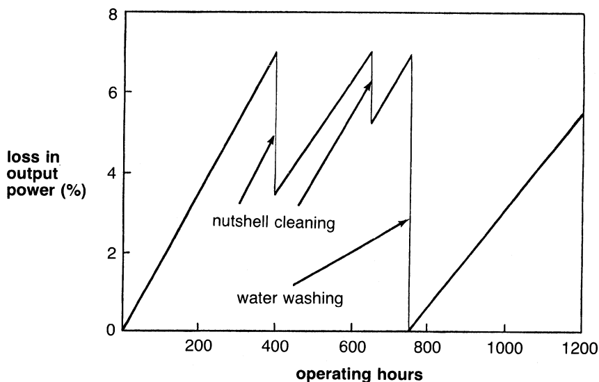
Figure 21-8. Effect of cleaning on power output.
