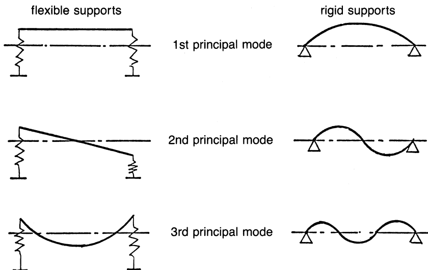
Figure 17-8. Typical principal modes for a symmetric and uniform shaft.
