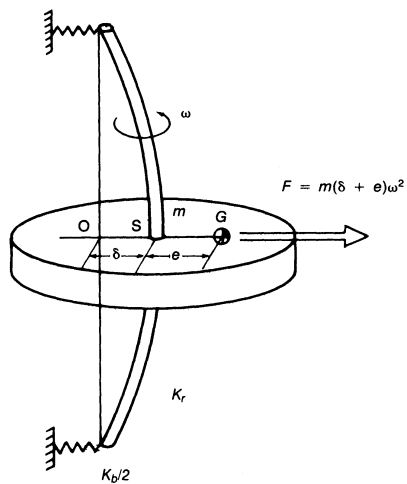
Figure 5-14b. Flexible supports.
