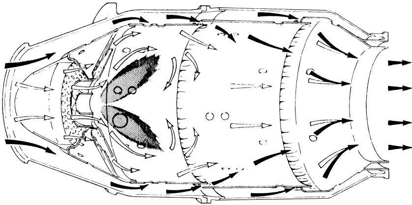
Figure 10-4. Flame stabilization created by impinging jets and general airflow pattern. (©Rolls-Royce Limited.)
