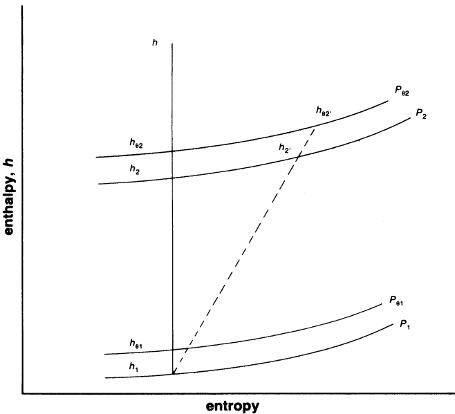
Figure 3-4. Entropy-enthalpy diagram of a compressor.
