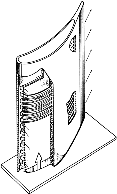
Figure 9-14. Strut insert blade.
