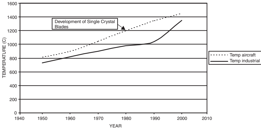
Figure 1-4. Trend in improvement in firing temperature.
