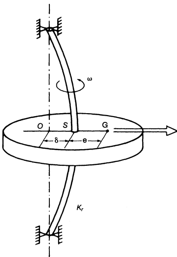
Figure 5-14a. Rigid supports.
