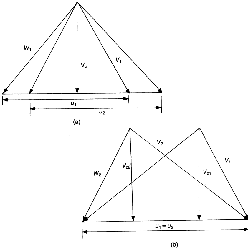
Figure 7-18. Velocity triangles.
