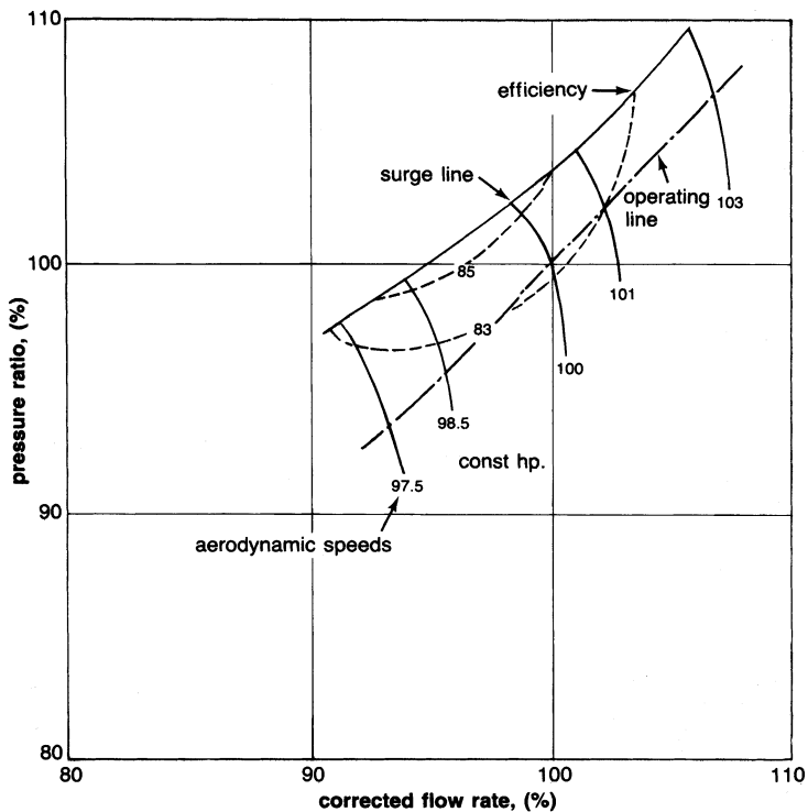
Figure 3-10. Typical flow map for an axial-flow compressor.
