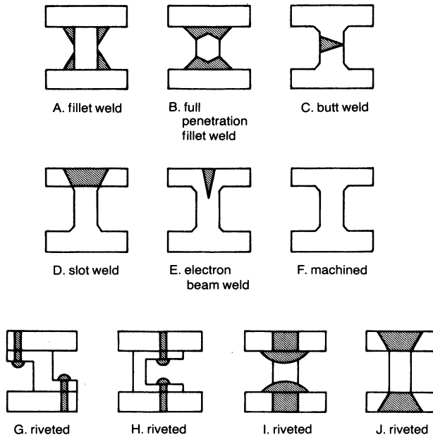
Figure 6-48. Several fabrication techniques for centrifugal impellers.
