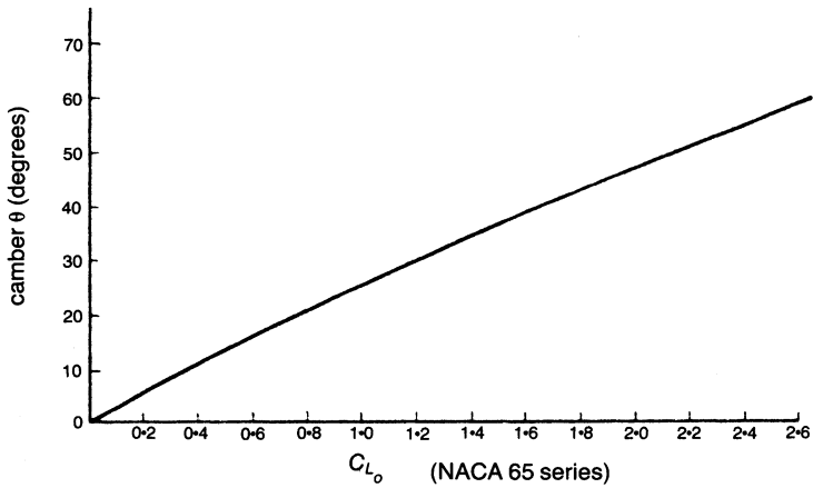
Figure 7-29. Approximate relation between camber ( \theta ) and C_{L0} of NACA 65 series.
