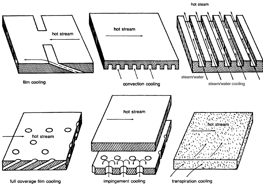
Figure 9-13. Various suggested cooling schemes.
