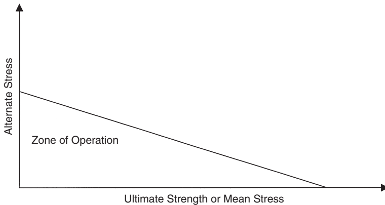
Figure 11-5. Goodman Diagram.
