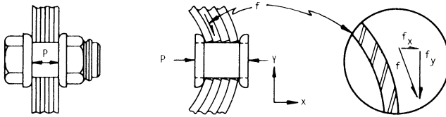
Figure 18-11. Frictional damping in a metal-disc coupling.
