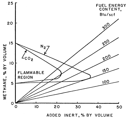
Figure 12-2. Flammable fuel mixtures of \text{CH}_4\text{-N}_2 and \text{CH}_4\text{-CO}_2 at one atm showing various energy levels.
