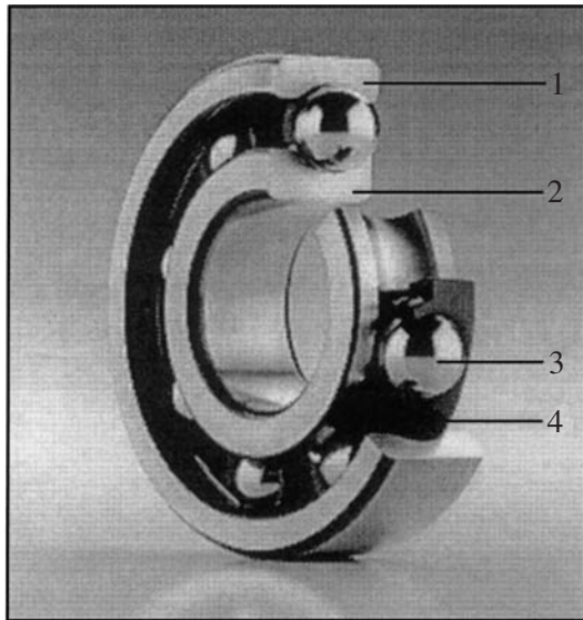
1 Outer ring, 2 Inner ring, 3 Rolling element, 4 Cage
