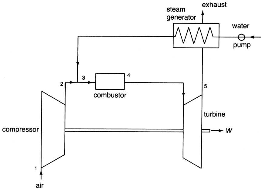
Figure 2-20. The steam injection cycle.
