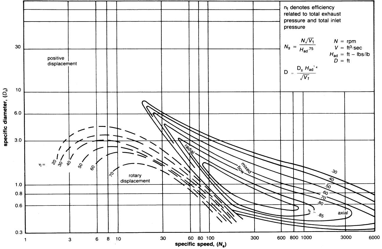
Figure 3-8a. Compressor map.
