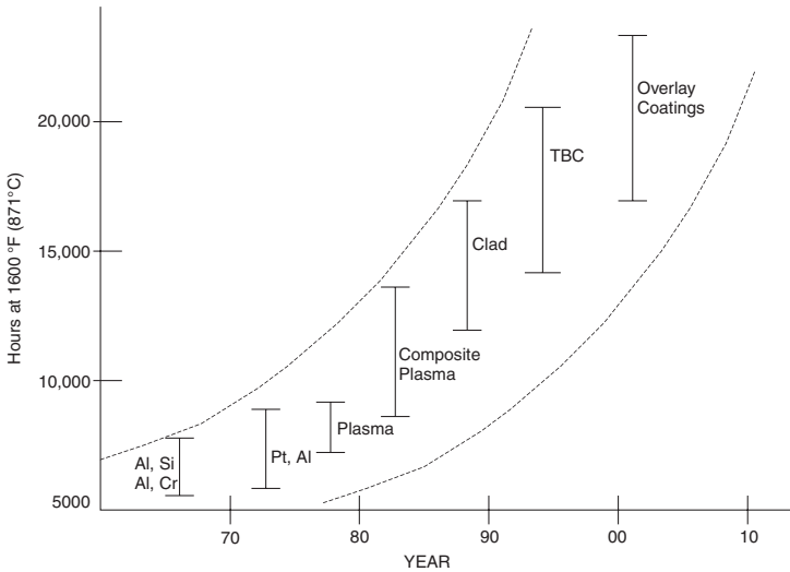
Figure 11-10. Developments of coatings.
