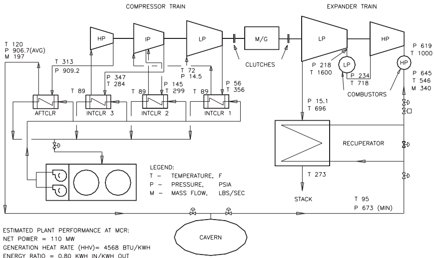
Figure 2-34. Schematic of a compressed air energy storage plant. (ASME Technical Paper 2000-GT-0595).
