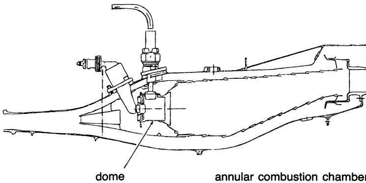
Figure 12-9. Cross section of an annular combustor showing high dome flow configuration. (Courtesy of General Electric Company.)
