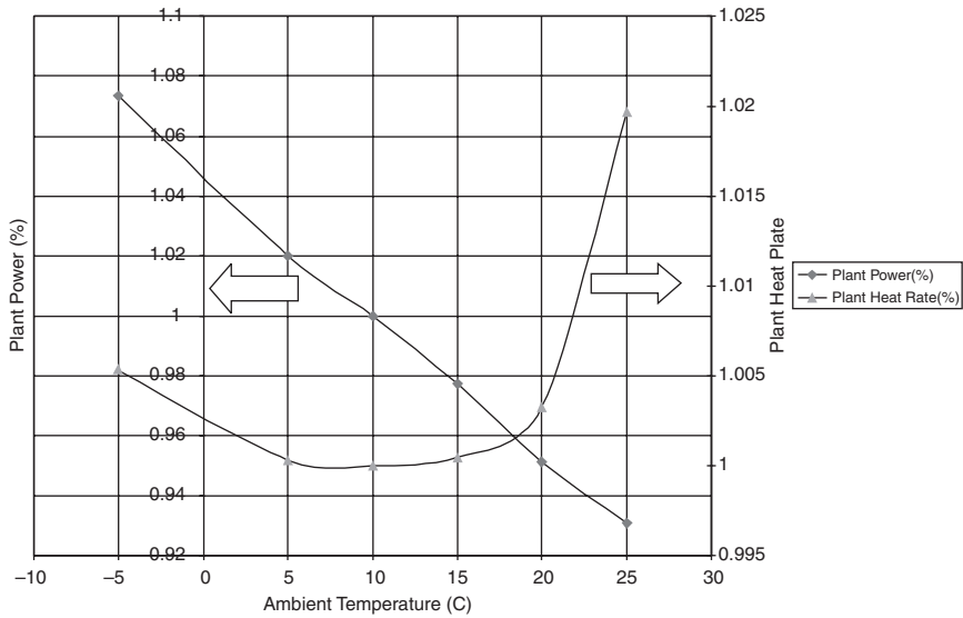
Figure 20-8. Plant conditions as a function of inlet ambient temperature.
