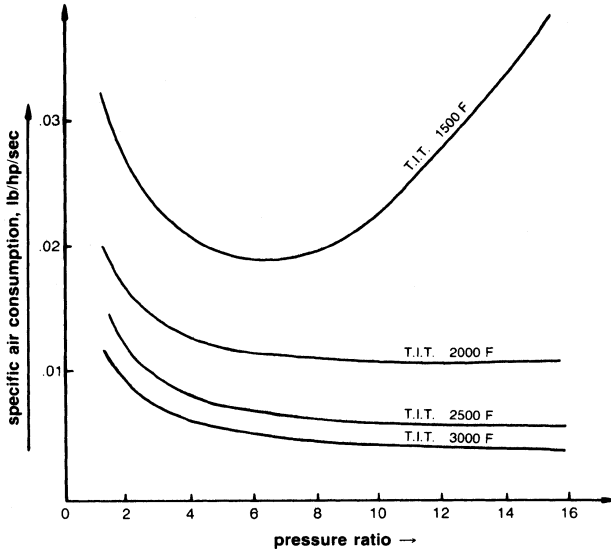
Figure 11-1a. Specific air versus pressure ratio and turbine inlet temperatures.
