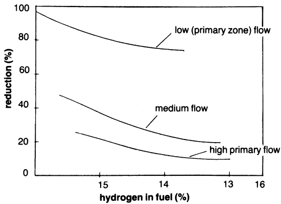
Figure 12-8. Effect of hydrogen saturation in primary flow on smoke.
