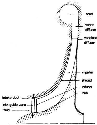
Figure 6-4. Schematic of a centrifugal compressor.
