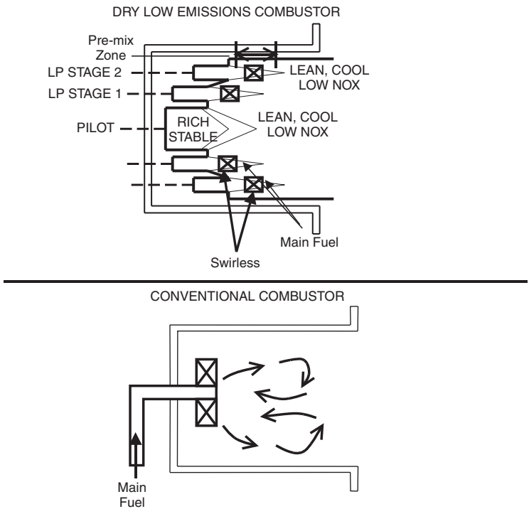
Figure 10-23. A schematic comparison of a typical dry low emission \text{NO}_x combustor and a conventional combustors.
