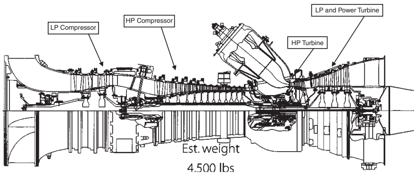
Figure 1-10. A cross section of an aeroderivative gas turbine engine.
