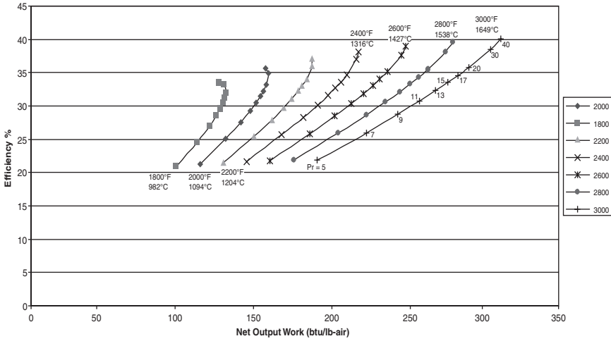
Figure 2-15. The performance map of an intercooled gas turbine cycle.
