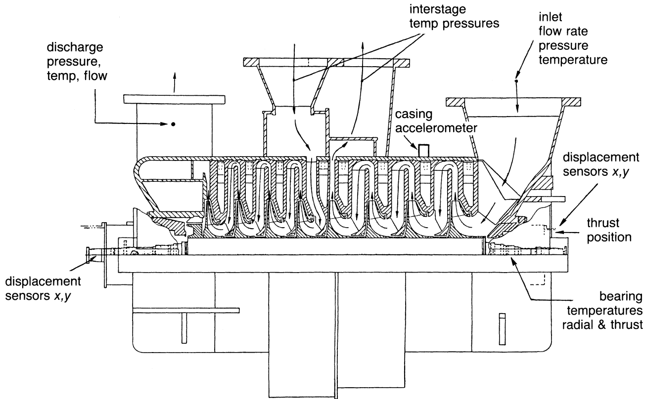
Figure 19-11. Instrumentation for monitoring and diagnostics on a centrifugal compressor.
