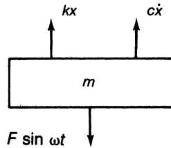
Figure 5-11. Free body diagram of mass ( M ).
