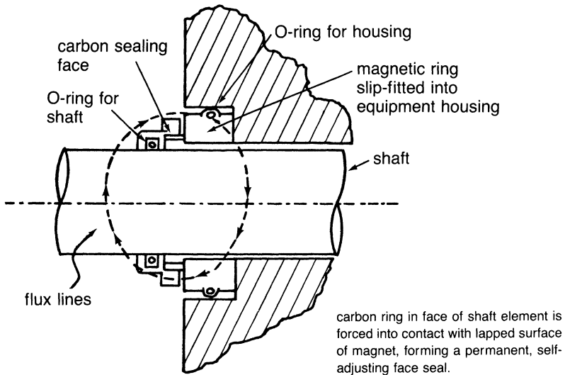
Figure 13-28. Simple magnetic-type seal.
