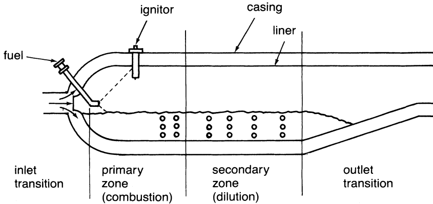
Figure 10-7. A can-annular combustor.
