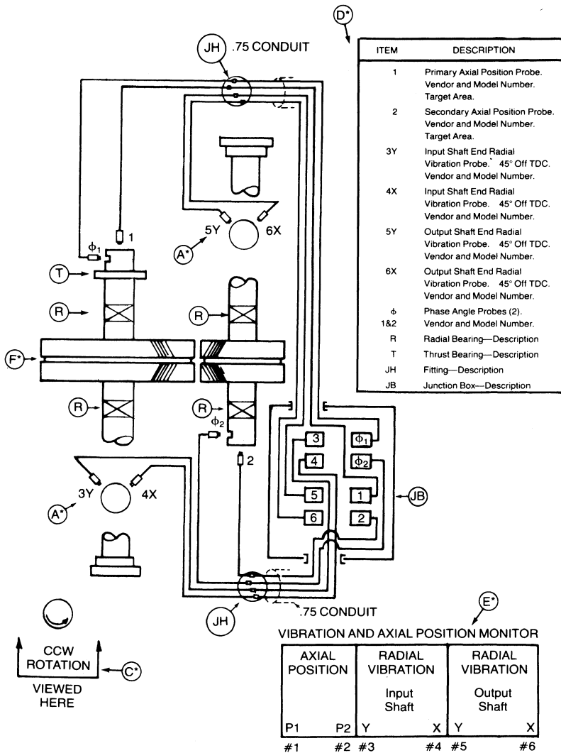
Figure 4-11. Typical protection system for a gearbox.
