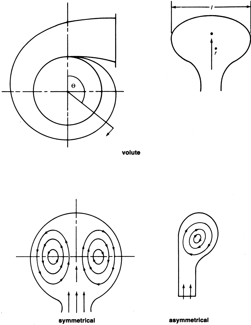
Figure 6-30. Flow patterns in volute.
