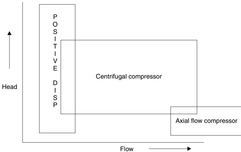
Figure 1-17. Performance characteristics of different types of compressors.
