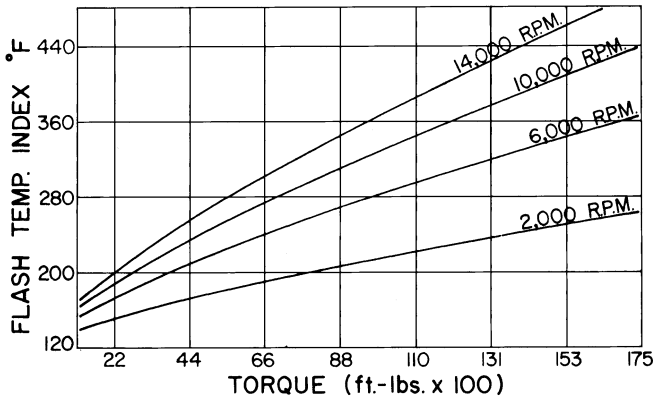
Figure 14-8. Scoring based on flash temperature index related to speed and torque. (Courtesy of Lufkin Industries, Inc.)
