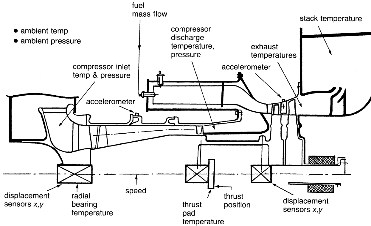
Figure 19-10. Instrumentation for monitoring and diagnostics on a gas turbine engine.
