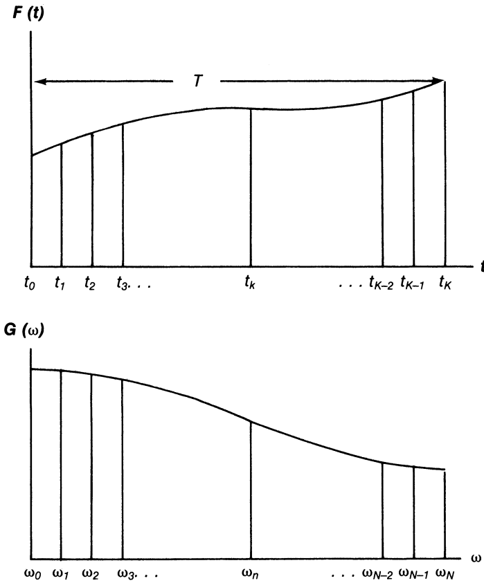
Figure 16-2. Discrete Fourier transform representation.
