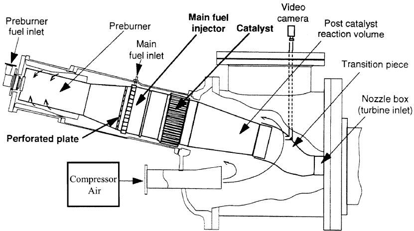
Figure 10-28. Schematic of a full scale catalytic combustor. Courtesy GE Power Systems and Catalytica Combustion Systems Inc.
