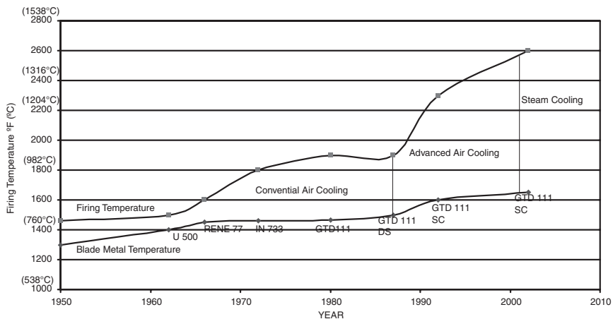
Figure 1-38. Firing temperature increase with blade material improvement.
