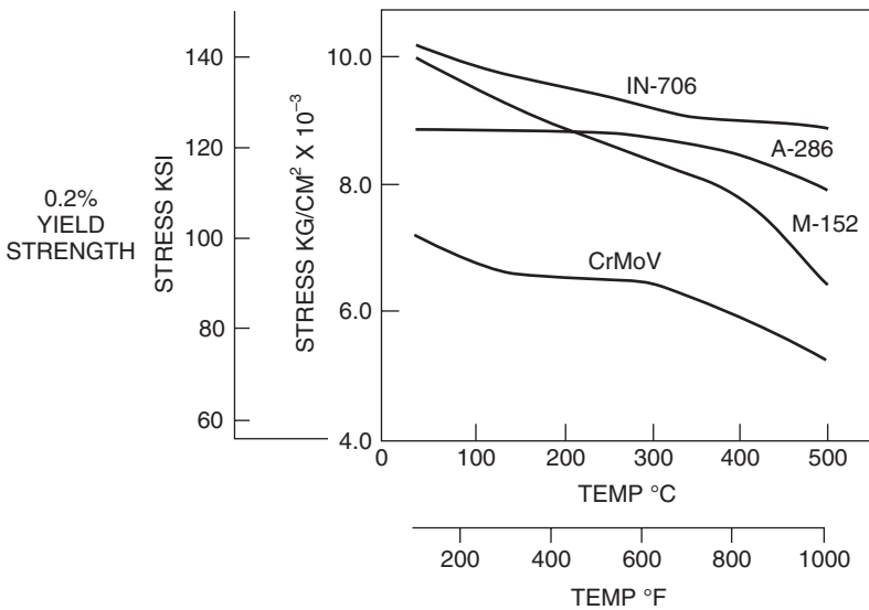
Figure 11-7. Turbine Wheel Alloys tensile yield strength comparison.
