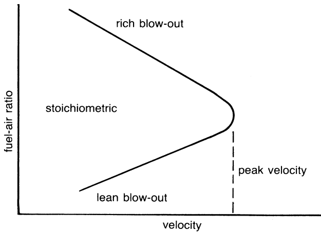
Figure 10-5. Range of burnable fuel-air ratios versus combustor gas velocity.
