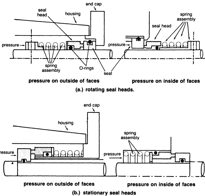
Figure 13-26. Rotating and stationary seal heads.
