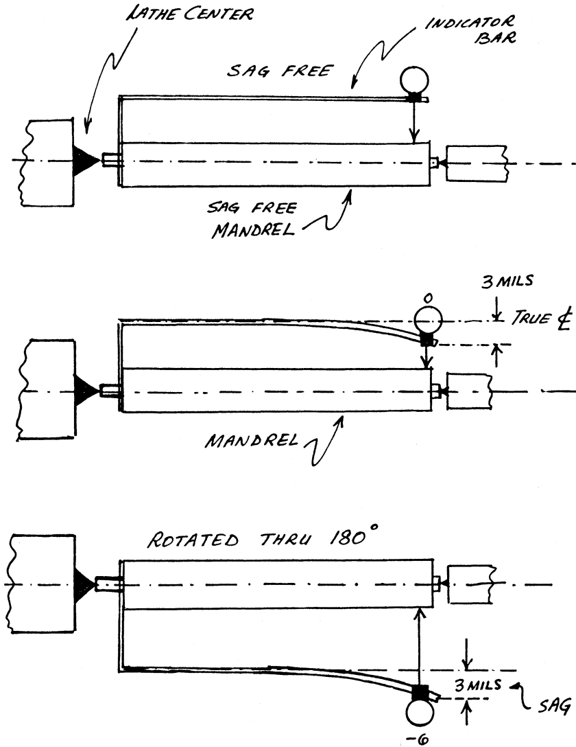
Figure 18-16. Method for determining sag.
