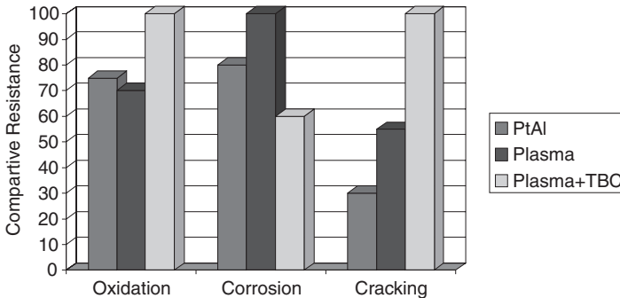
Figure 11-11. Comparative resistance in various types of coatings.
