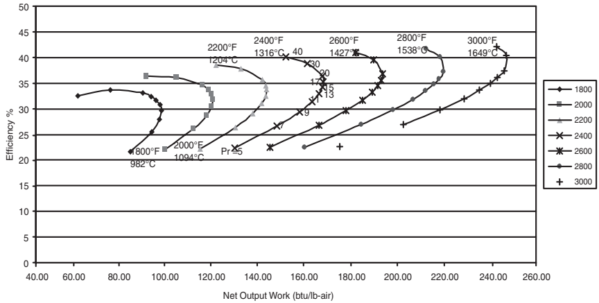
Figure 1-6. Performance map of a simple cycle gas turbine.
