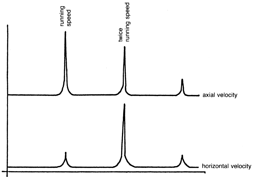
Figure 16-10. A typical misalignment signature plot.
