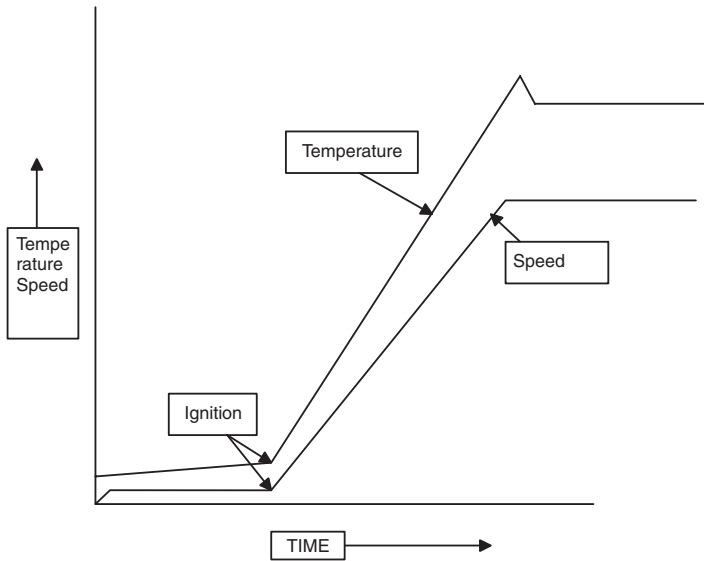
Figure 19-2. Startup characteristics of a gas turbine.
