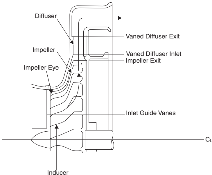
Figure 1-21. Schematic of a centrifugal compressor stage.
