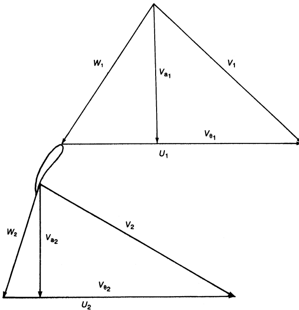
Figure 3-3. Velocity triangles for an axial-flow compressor.
