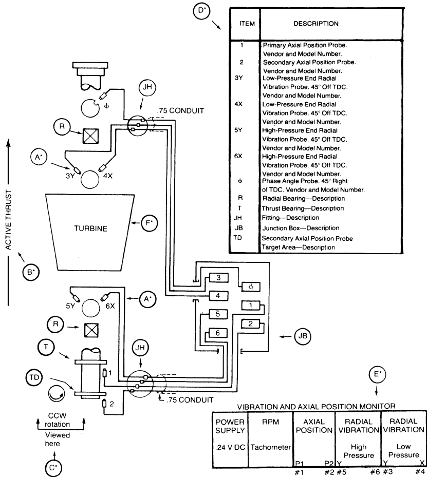
Figure 4-10. Typical protection system for a turbine.
