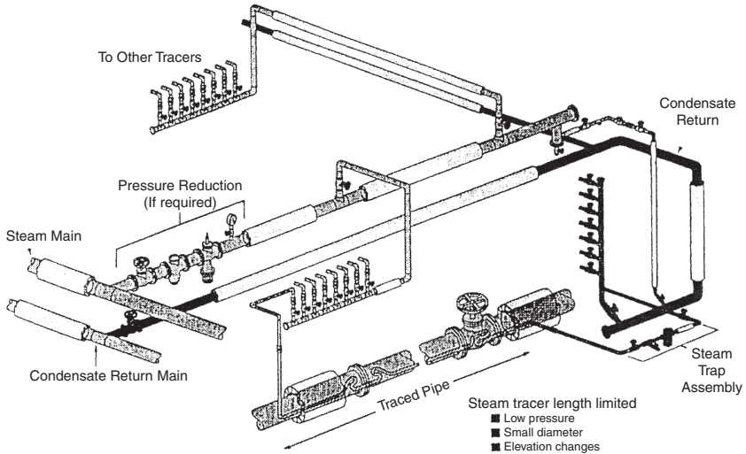
Figure 12-12. Steam tracing system.
