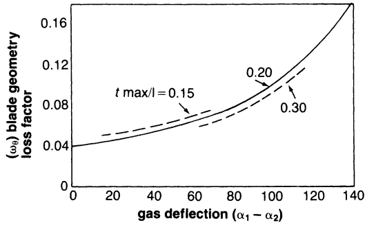
Figure 9-27. Blade geometry loss.
