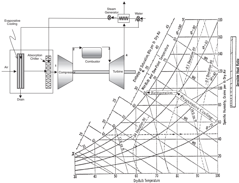
Figure 2-38. Evaporative and refrigerated inlet systems.
