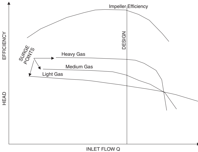
Figure 6-40. Effect of gas composition.
