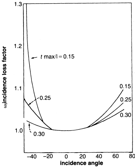
Figure 9-28. Incidence angle loss.
