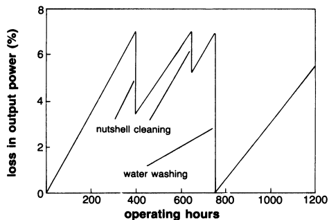
Figure 12-10. Effect of cleaning on power output.
