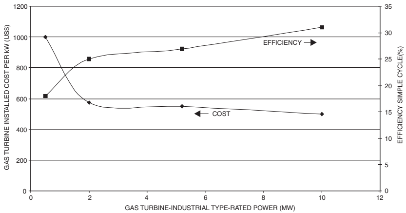
Figure 4-3. Installed cost and efficiency of industrial type turbines.
