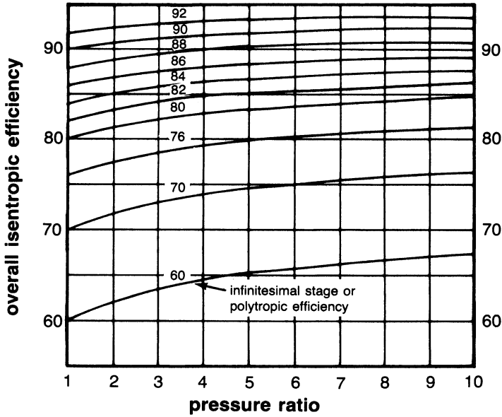
Figure 3-7. Overall and polytropic efficiency expansion.
