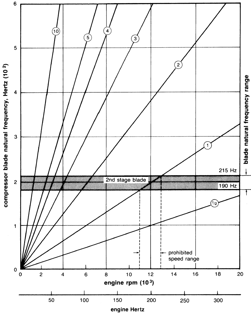
Figure 5-25. Campbell diagram.
