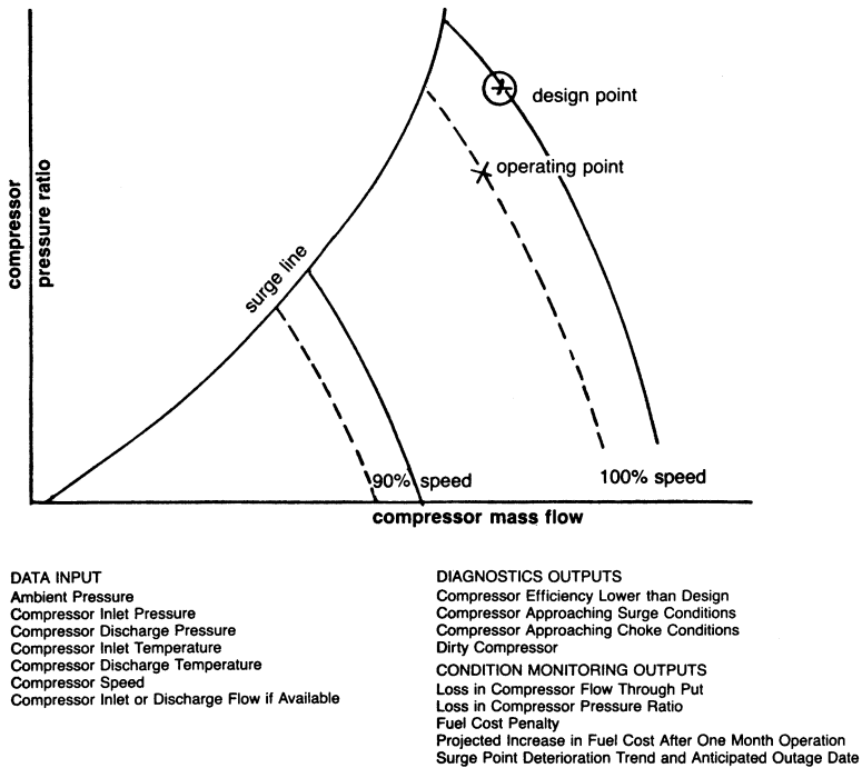
Figure 19-15. Aerothermal condition monitoring for compressors.
