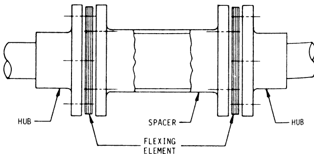
Figure 18-10. Typical metal-flexing disc coupling.
