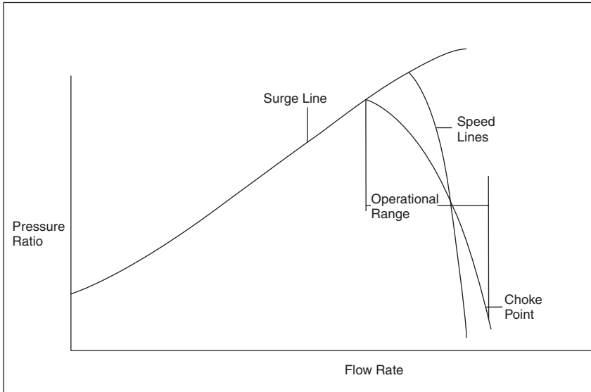
Figure 1-18. Schematic of a compressor performance map.
