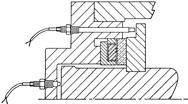
Figure 21-11. Actual probes for thrust-bearing monitoring.
