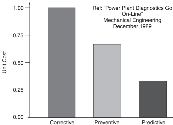
Figure 19-7. Comparison between various maintenance techniques.
