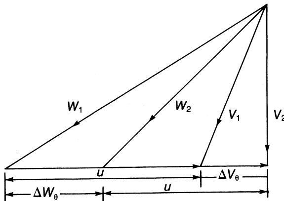
Figure 7-21. Axial-outflow stage velocity diagram.
