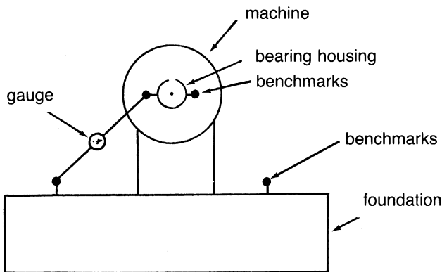
Figure 18-18. Hot alignment system with dial indicator.
