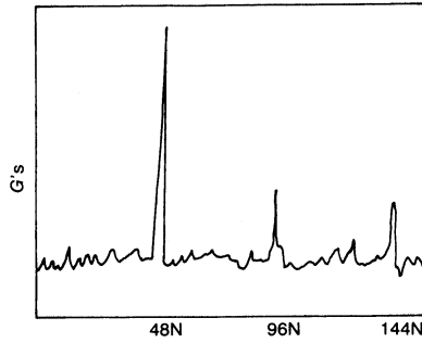
Figure 7-38. High-pressure bleed chamber—9400 rpm.
