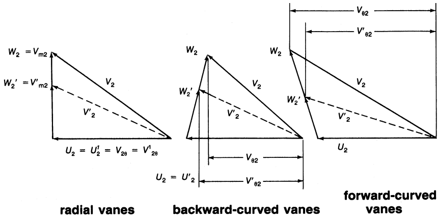
Figure 6-10. Velocity triangles.
