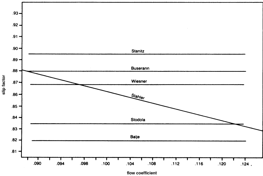
Figure 6-26. Various slip factors as a function of the flow coefficient.
