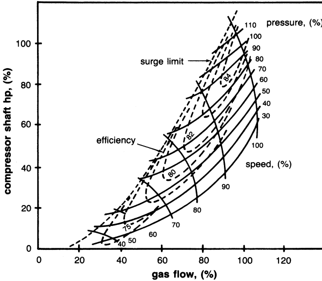
Figure 3-11. Typical compressor map where speedlines are a function of horsepower and flow rate.
