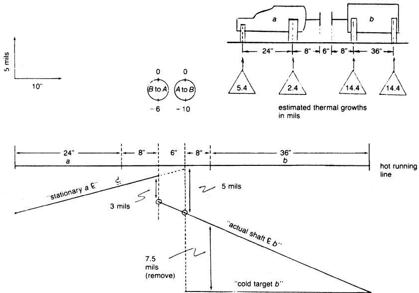
Figure 18-17. Graphic plotting for reverse-dial indicator method.
