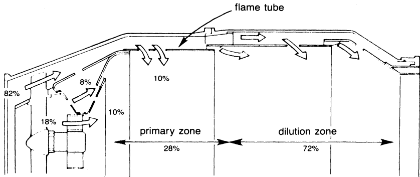
Figure 10-6. Addition of flame tube distributes flow between primary and dilution zone.
