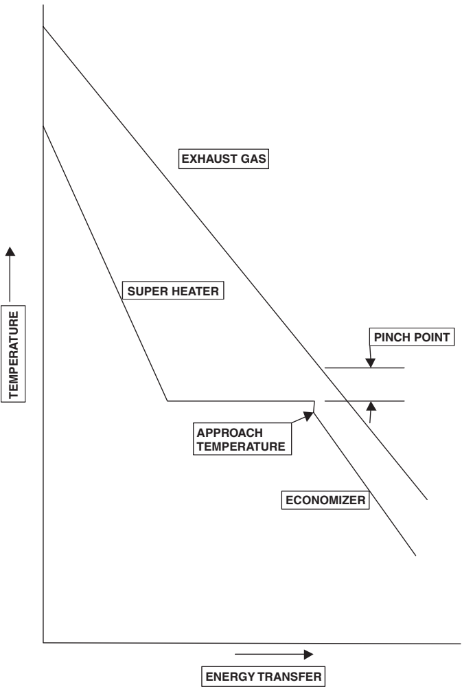
Figure 1-40. Energy transfer diagram in an HRSG of a combined cycle power plant.
