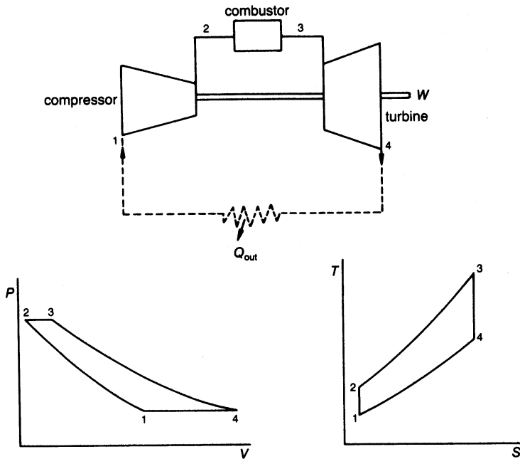
Figure 2-1. The air-standard Brayton cycle.
