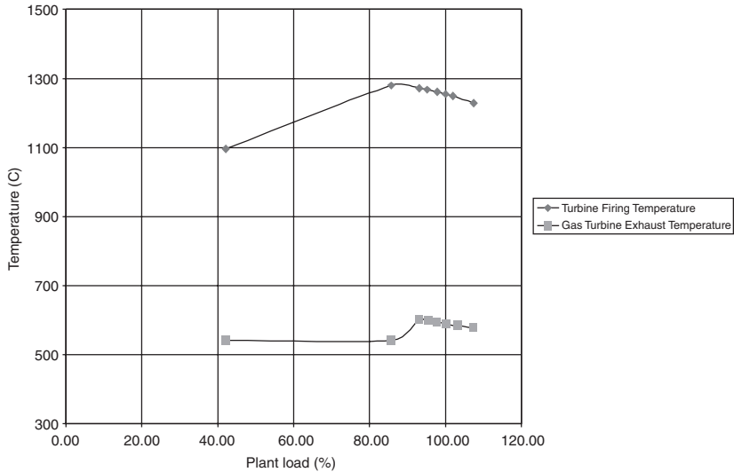
Figure 20-13. Effect of the plant load on turbine firing temperature and the turbine exhaust.
