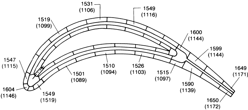
Figure 9-15. Temperature distribution for strut insert design, °F (cooled).
