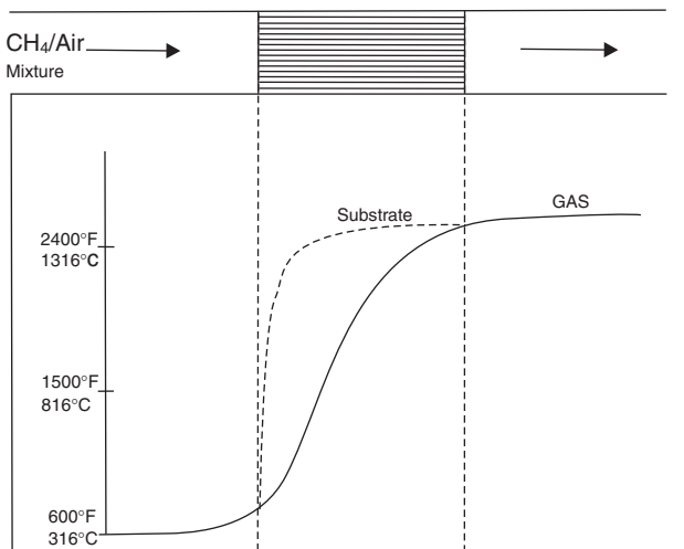
Figure 10-26. Schematic temperature profiles for catalyst (substrate) and bulk gas in a traditional catalytic combustor.
