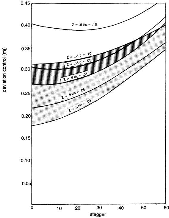
Figure 7-27. Position of maximum thickness effect on deviation.
