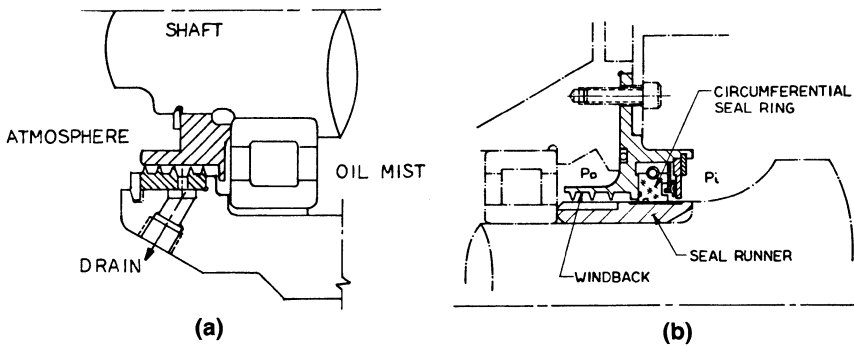
Figure 13-23. Windback seal.
