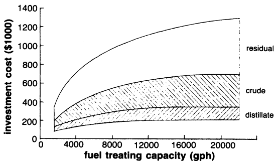
Figure 12-11. Gas turbine fuel treatment plant investment costs. (Courtesy of General Electric Company.)
