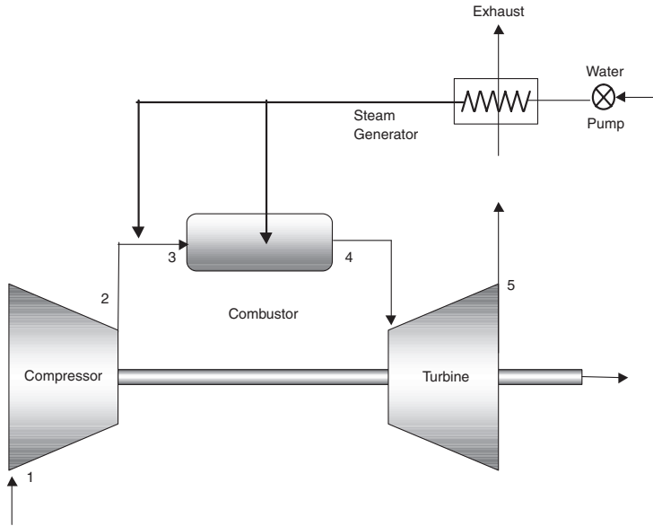
Figure 2-42. Steam injection at exit of compressor and in the combustor of the gas turbine.
