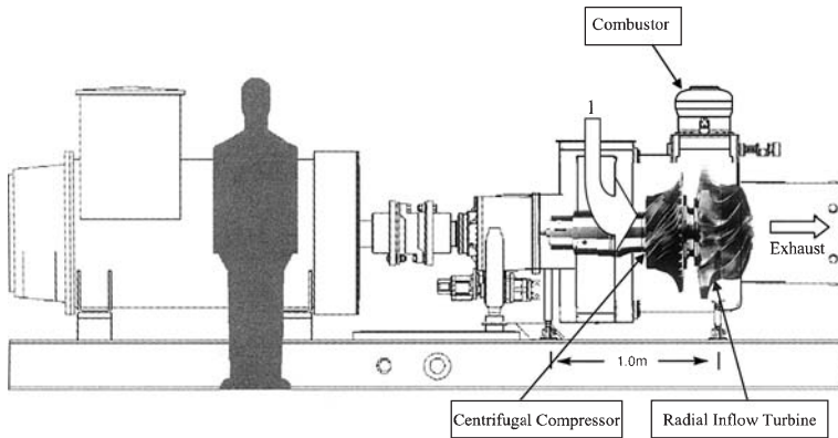
Figure 1-13. A small radial flow gas turbine cutaway showing the turbine rotor.
