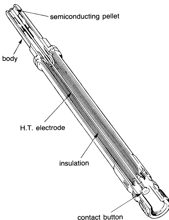
Figure 10-11. An ignitor plug. (©Rolls-Royce Limited.)
