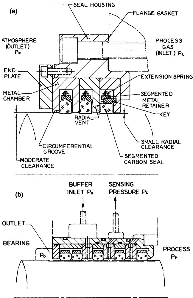
Figure 13-24. Floating-type restrictive ring seal.
