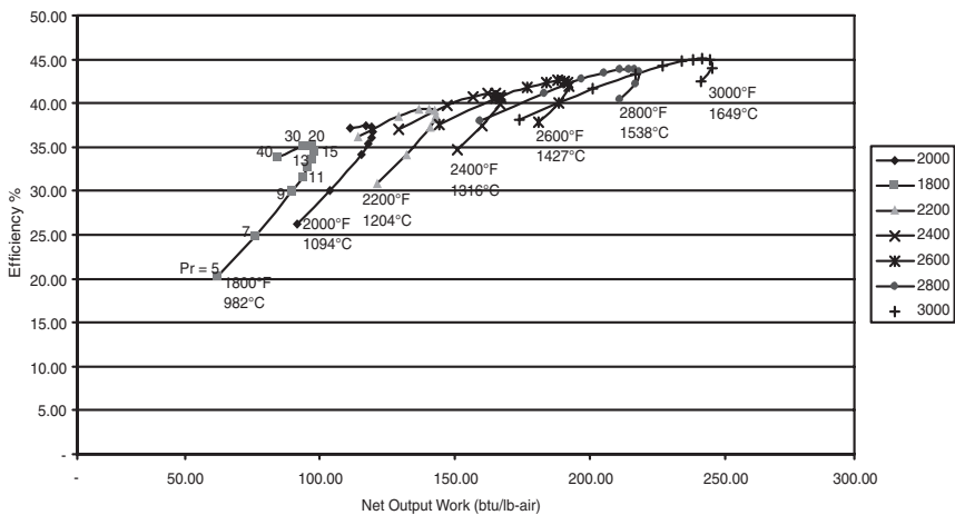
Figure 1-7. Performance map of a regenerative gas turbine.
