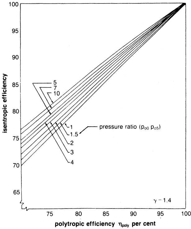
Figure 8-8. Relationship between polytropic and isentropic efficiency during expansion.
