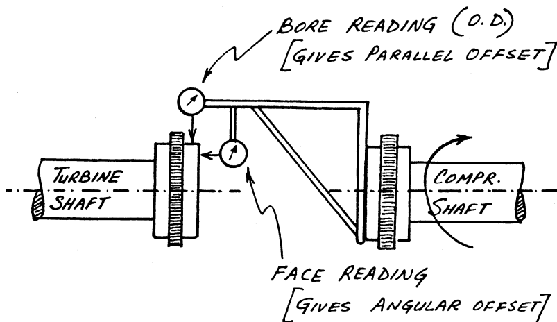
Figure 18-14. Face-OD indicator setup.
