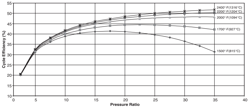
Figure 2-2. Overall cycle efficiency as a function of the firing temperature and pressure ratio. Based on a compressor efficiency of 87% and a turbine efficiency of 92%.
