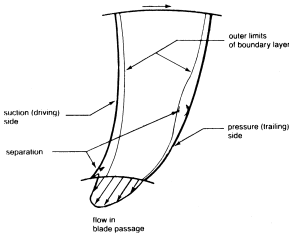
Figure 8-16. Boundary-layer formation in a radial-flow impeller.
