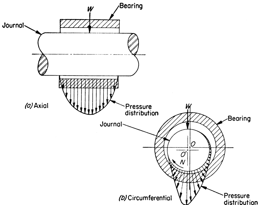
Figure 13-8. Pressure distribution in a full journal bearing.
