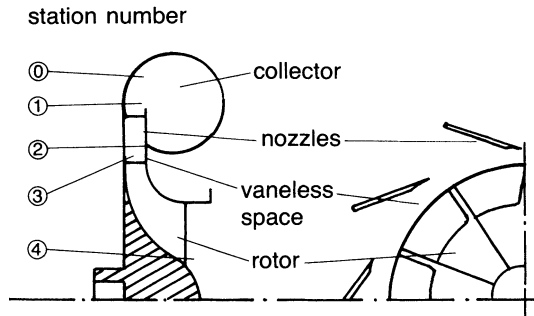
Figure 8-5. Components of a radial-inflow turbine.
