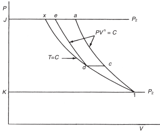
Figure 2-6. Multistages compression with intercooling.
