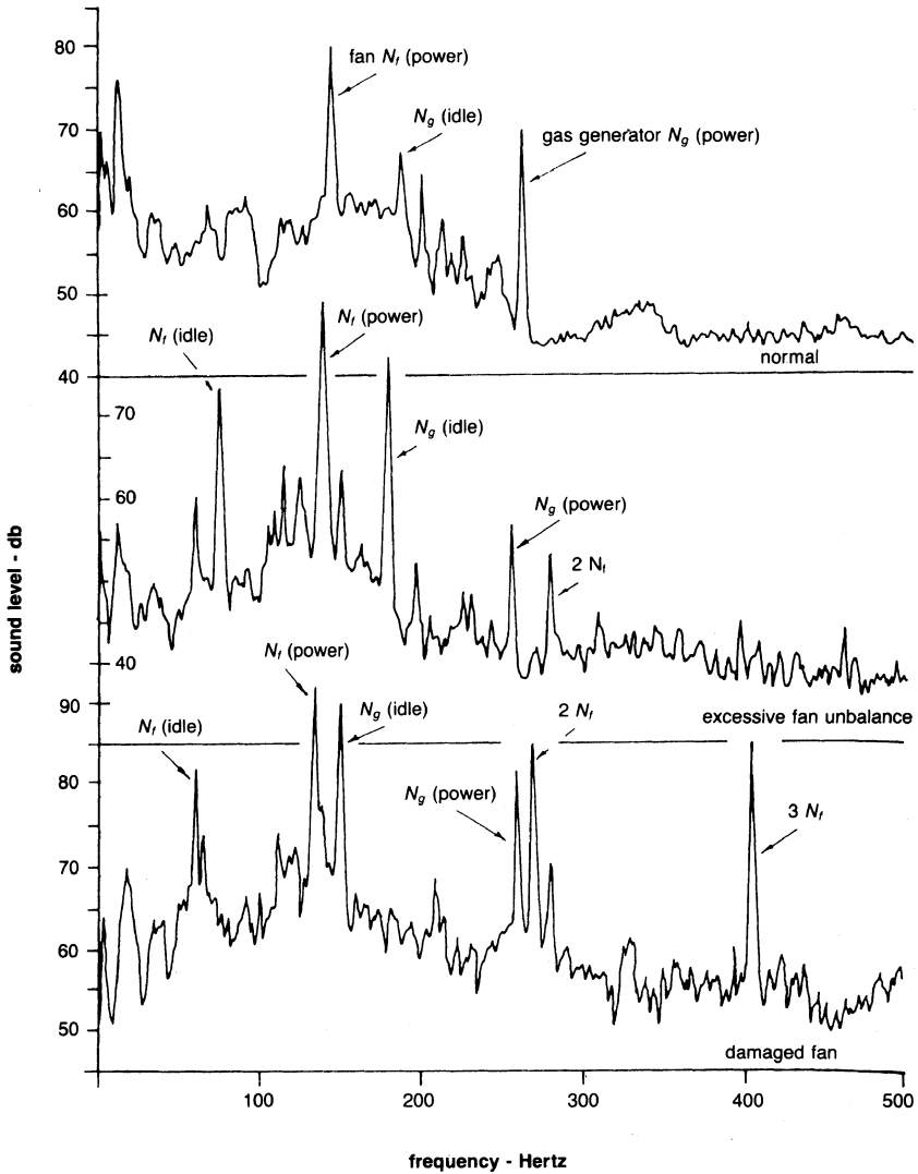
Figure 16-15. Jet engine acoustic signature.
