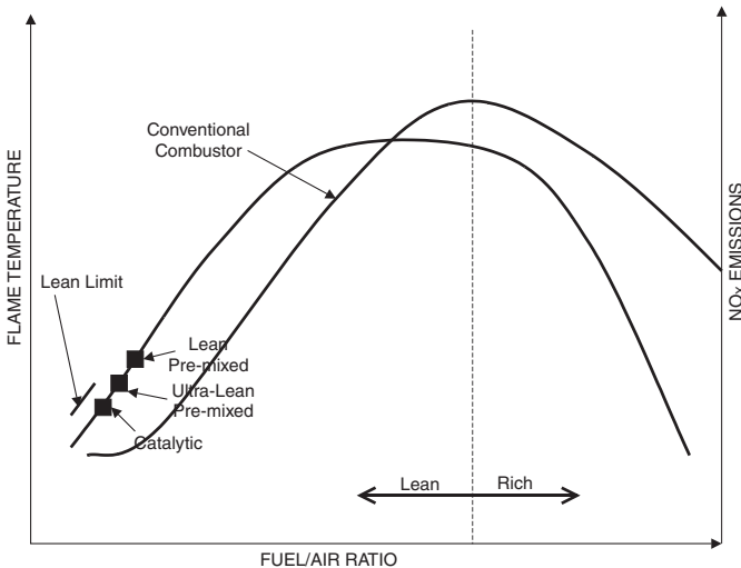
Figure 10-22. Effect of fuel /air ratio on flame temperature and NO x emissions.
