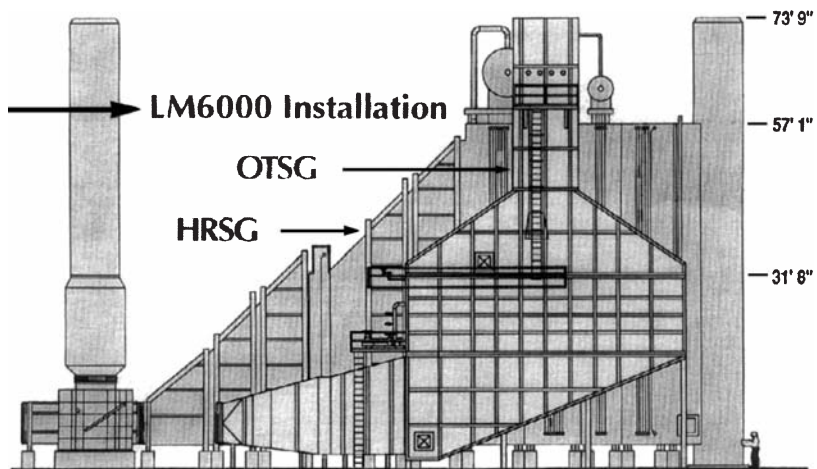
Figure 1-39. Comparison of a drum type HRSG to a once through steam generator. (Courtesy Innovative Steam Technologies.)
