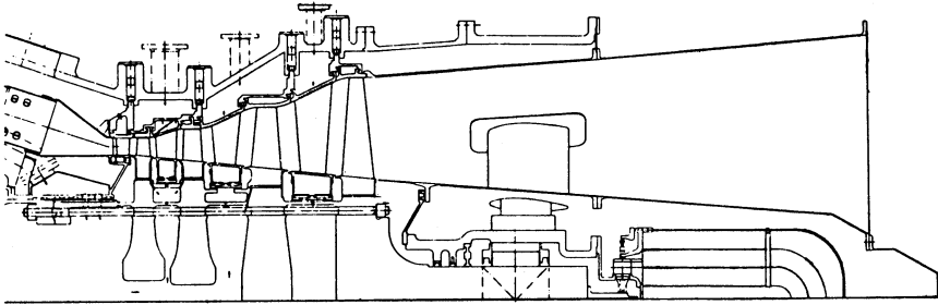
Figure 1-37. Schematic of an axial flow turbine.
