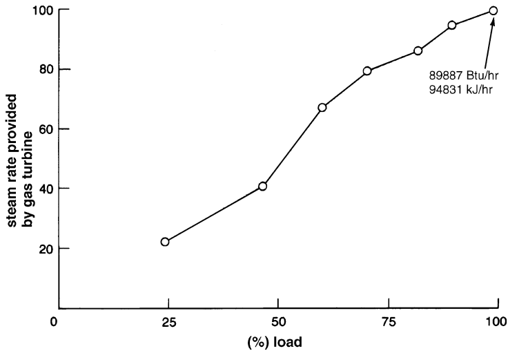
Figure 3-21. Steam generated by exhaust gases of gas turbine as a function of gas turbine load.
