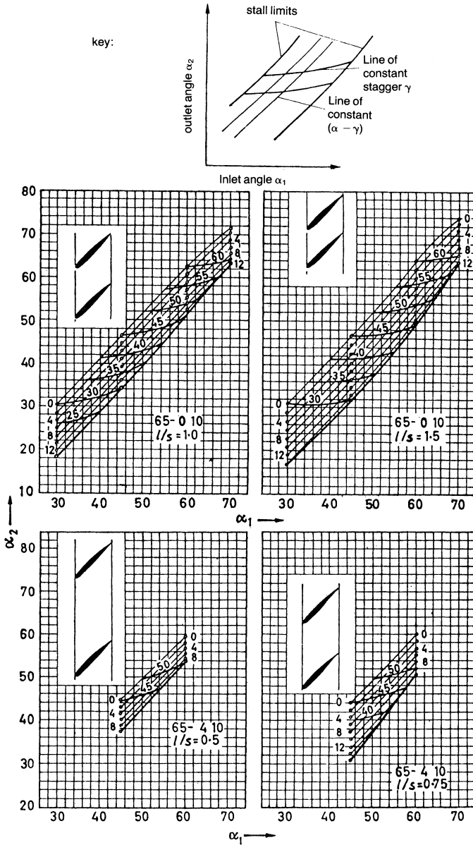
Figure 7-30. The NACA 65 series cascade data. (Courtesy of G. Mellor, Massachusetts Institute of Technology, Gas Turbine Laboratory Publication.)
