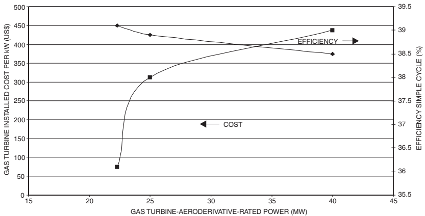
Figure 4-4. Installed cost and efficiency of aero-derivative type turbines.
