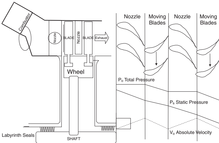
Figure 9-10. Schematic of a reaction-type turbine showing the distribution of the thermodynamic and fluid mechanic properties.
