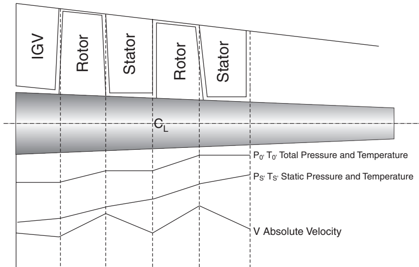
Figure 7-3. Variation of enthalpy, velocity, and pressure through an axial-flow compressor.
