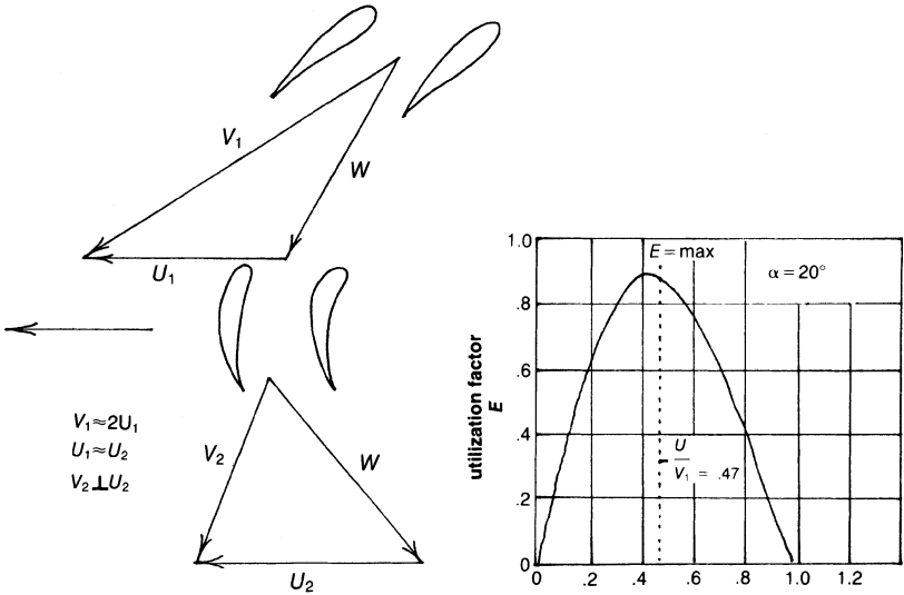
Figure 9-9. Effect of velocity and air angle on utilization factor.
