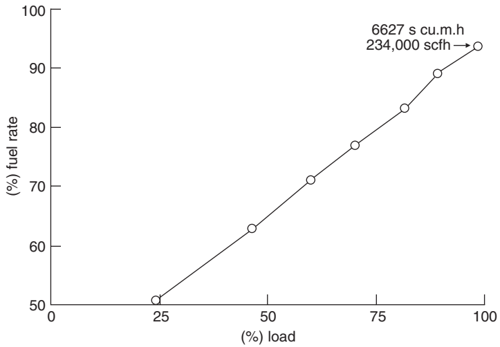
Figure 3-20. Fuel consumption as a function of gas turbine load.
