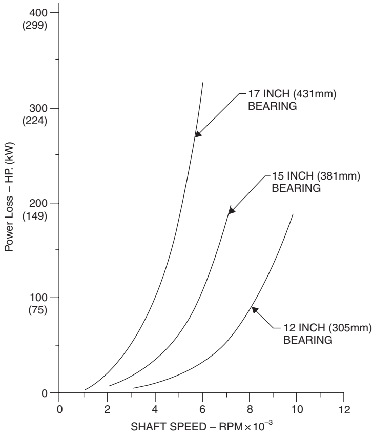
Figure 13-20. Total power loss in thrust bearings.
