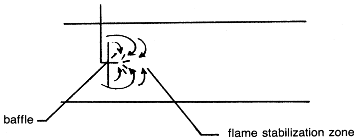
Figure 10-2. Baffle added to straight-walled duct to create flame stabilization zone.
