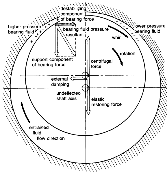
Figure 5-23a. Oil whirl. (Ehrich, F.F., "Identification and Avoidance of Instabilities and Self-Excited Vibrations in Rotating Machinery," Adopted from ASME Paper 72-DE-21, General Electric Co., Aircraft Engine Group, Group Engineering Division, May 11, 1972.)
