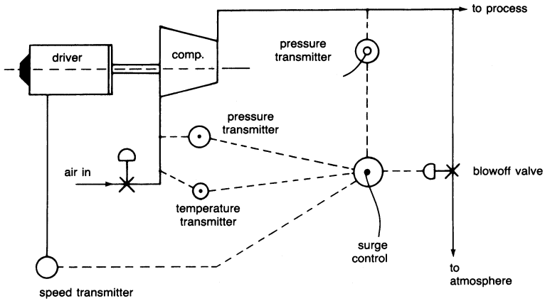
Figure 6-41. Pressure-oriented anti-surge control system.
