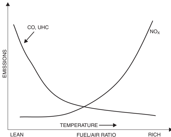
Figure 10-20. The effect of flame temperature on emissions.
