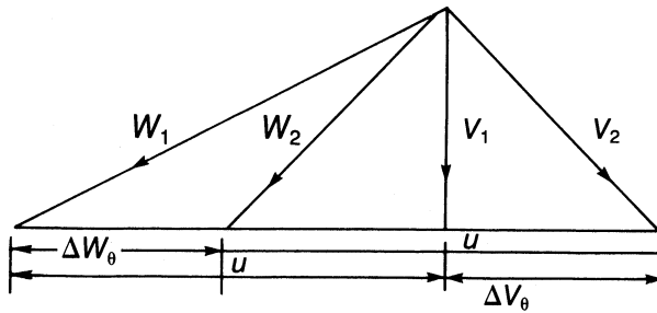
Figure 7-20. Axial-entry stage velocity diagram.
