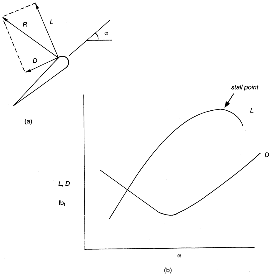
Figure 7-6. Characteristics of the lift and drag forces on an airfoil.
