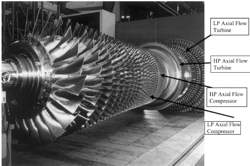
Figure 1-20. A high-pressure ratio turbine rotor. (Courtesy ALSTOM.)
