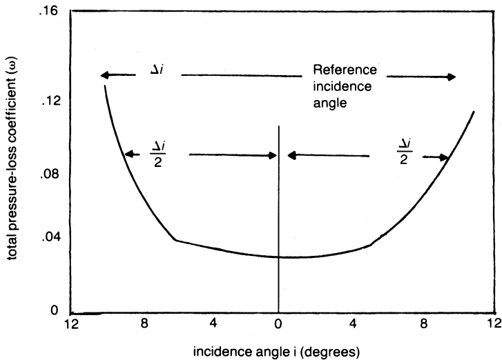
Figure 7-22. Loss as a function of incidence angle.
