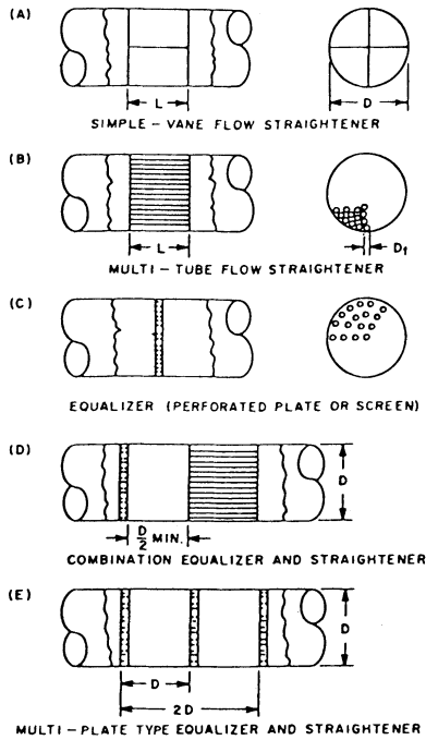
Figure 20-1. Flow equalizers and straighteners. (Power Test Code 10, Compressors and Exhausters , American Society of Mechanical Engineers, 1965.)
