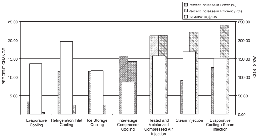
Figure 2-45. Comparison of various cycles based on percent change in power and efficiency and cost $/KW.
