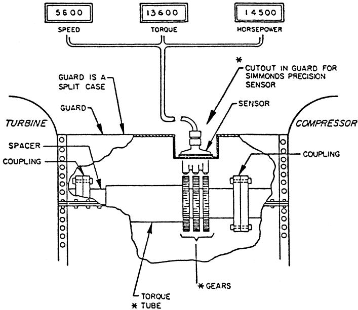
Figure 19-14. Torque meter for a gas turbine.
