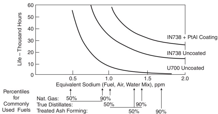
Figure 11-8. Effect of sodium corrosion on blade life.
