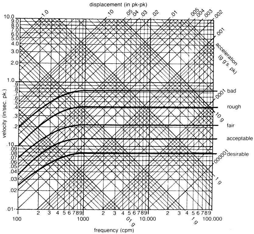
Figure 19-13. Vibration nomograph and severity chart. (Courtesy of IRD Mechanical Analysis, Inc.)
