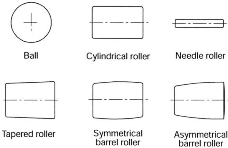
Figure 13-4. Various types of rollers used in a rolling bearing. (Courtesy FAG bearings.)
