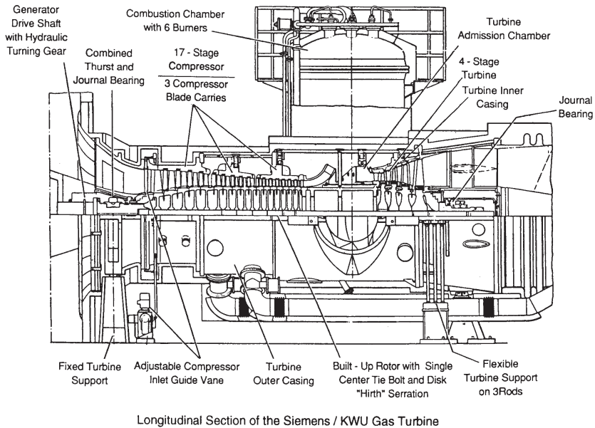
Figure 1-9. Frame-type gas turbine with silo type combustors. (Courtesy Siemens Power Generation.)
