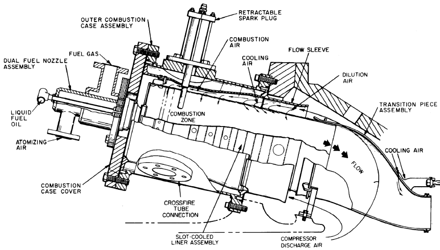
Figure 1-25. A typical reverse flow can-annular combustor.
