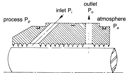
f. buffered-vented straight labyrinth
