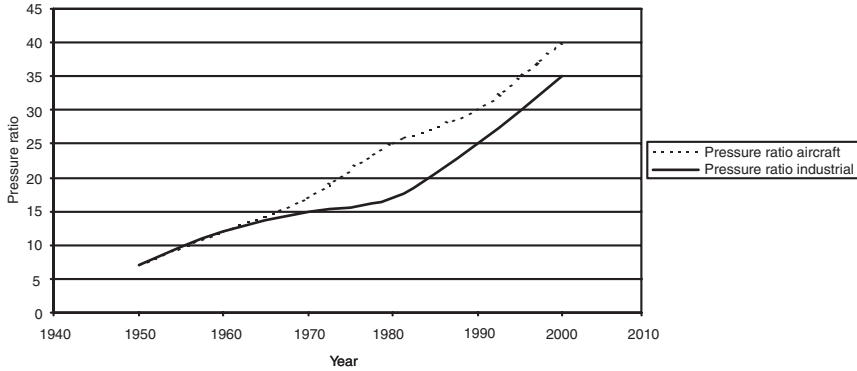
Figure 1-3. Development of engine pressure ratio over the years.
