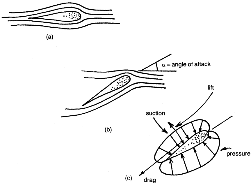
Figure 7-5. Flow around an airfoil at various angles of attack.
