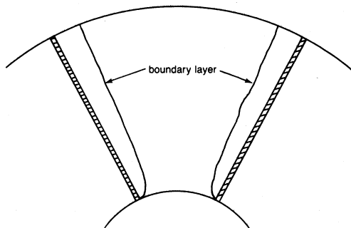
Figure 6-23. Boundary-layer development.
