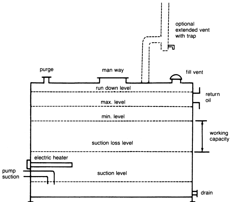
Figure 15-2. Lube oil reservoir.
