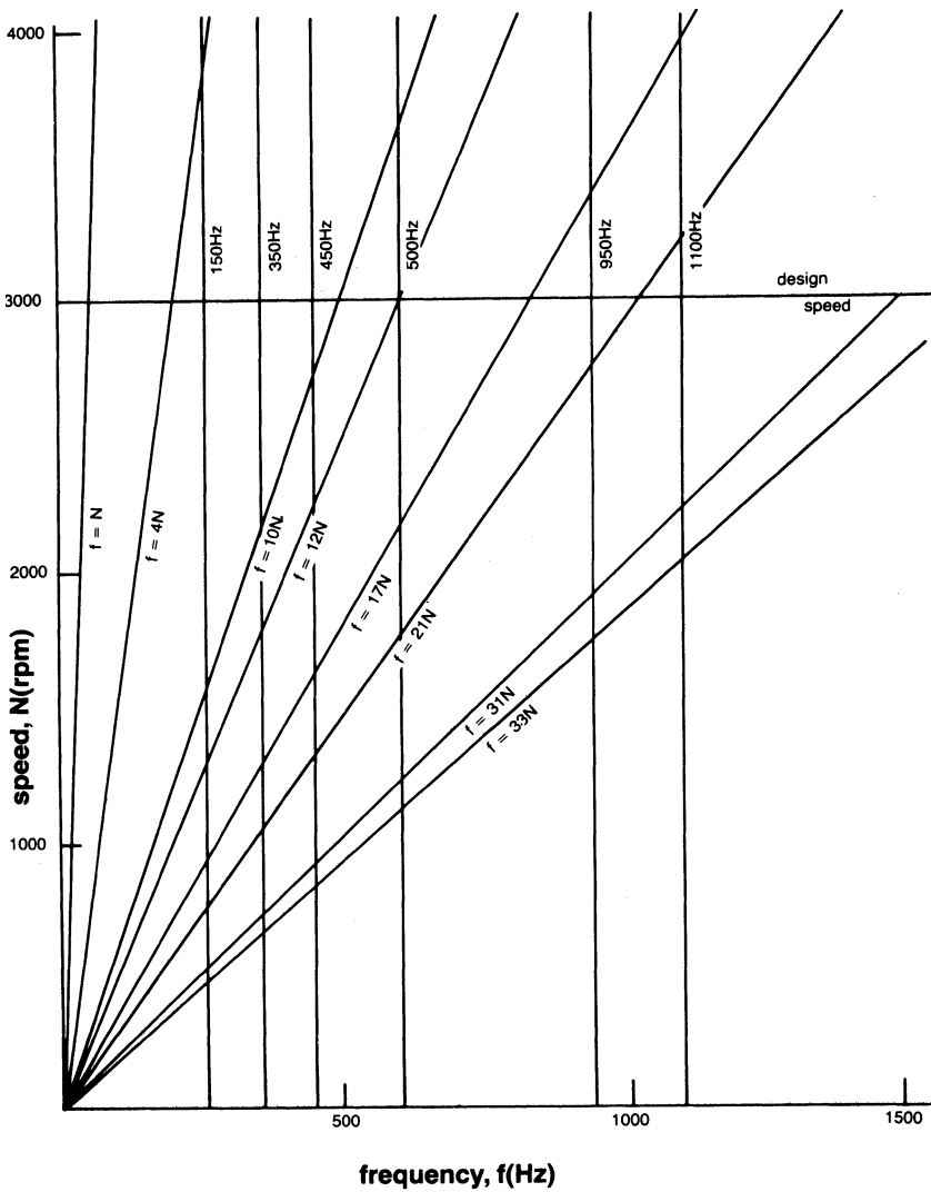
Figure 5-28. Campbell diagram of tested impeller.
