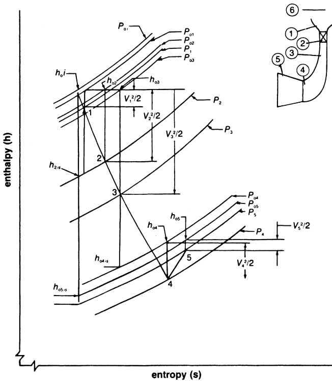
Figure 8-7. h-s diagram for turbine stage process.
