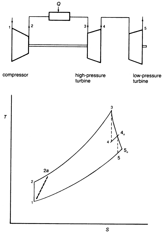
Figure 2-11. The split-shaft gas turbine cycle.
