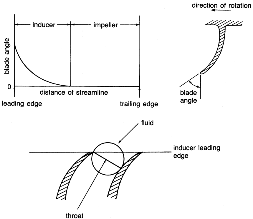
Figure 6-19. Inducer centrifugal compressor.
