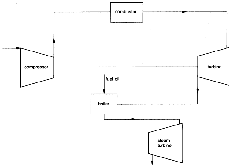
Figure 3-15. Schematic of combined cycle gas turbine.
