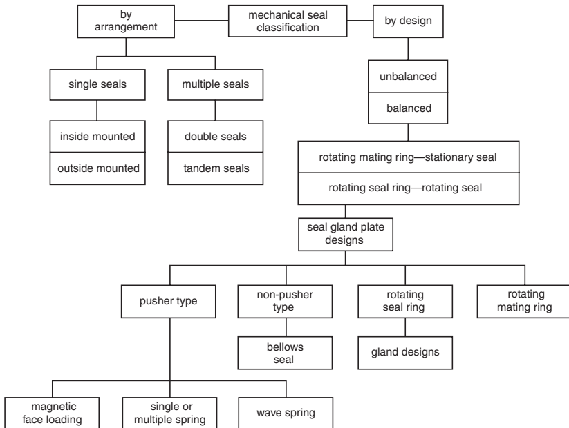
Figure 13-33. Mechanical seal classifications.
