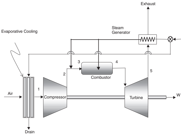
Figure 2-44. Evaporative cooling and steam injection in a gas turbine.
