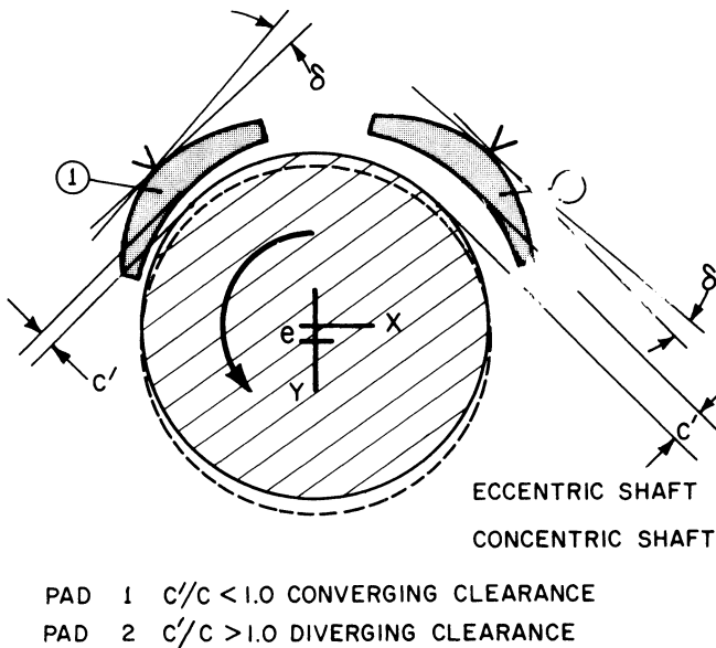
Figure 13-12. Tilting-pad bearing pre-load.
