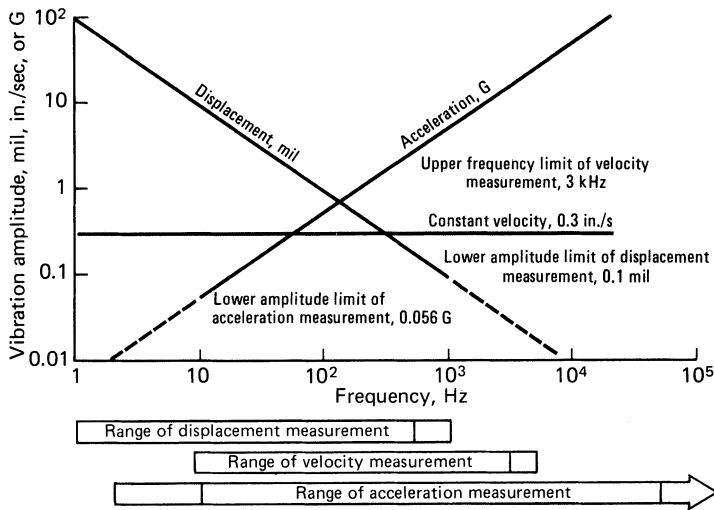
Figure 16-3. Limitations on machinery vibrations analysis systems and transducers.
