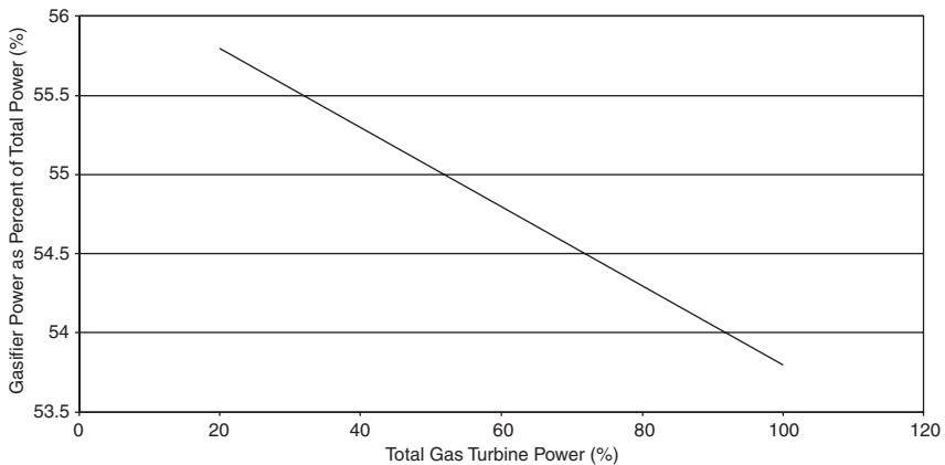
Figure 20-10. Gasifier power as a function of total gas turbine power.
