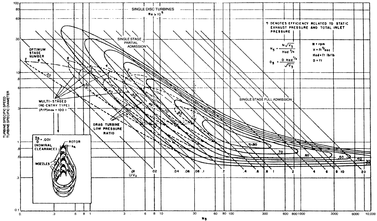
Figure 3-8b. Turbine map. (Balje, O.E., "A Study of Reynolds Number Effects in Turbomachinery," Journal of Engineering for Power , ASME Trans., Vol. 86, Series A, p. 227.)
