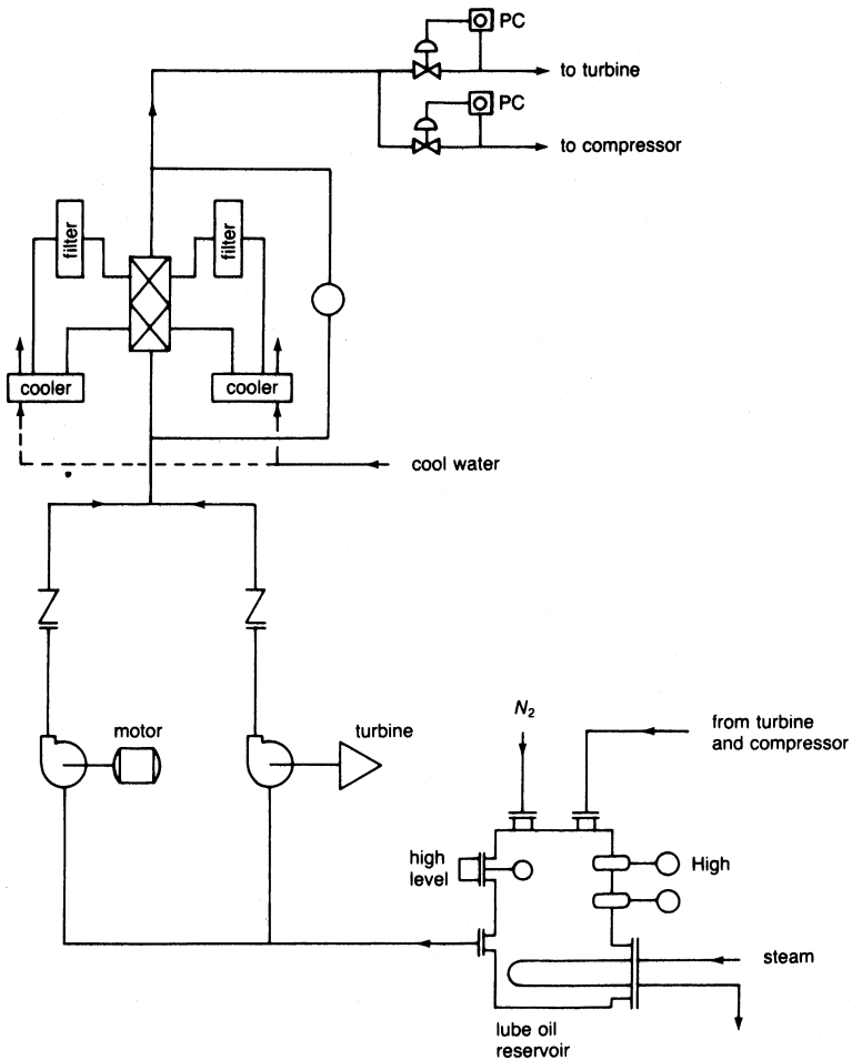
Figure 15-1. A typical lube oil system.
