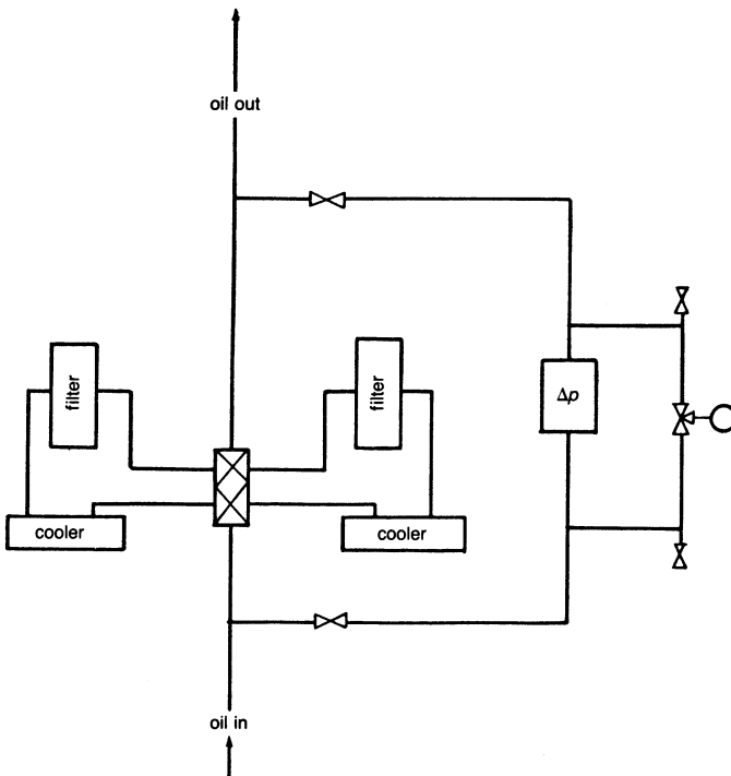
Figure 15-3. Cooler-filter arrangement.
