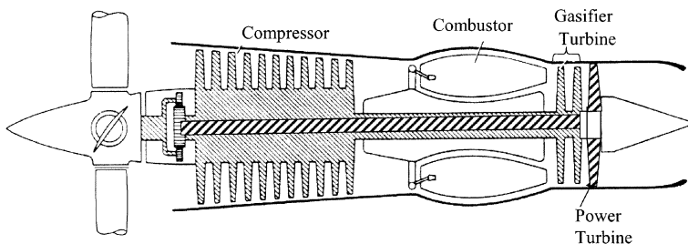
Figure 4-2. Schematic of a turboprop engine.
