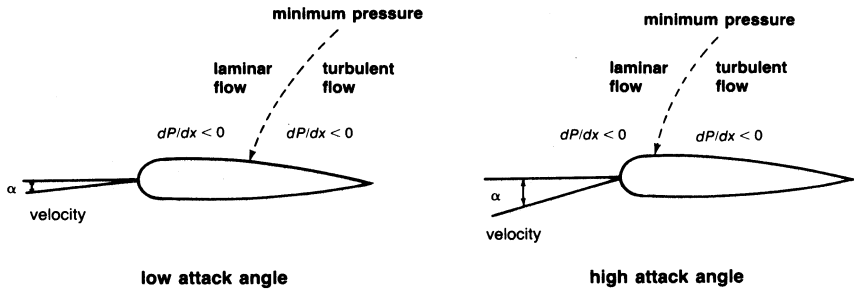
Figure 7-8. Laminar flow airfoils.
