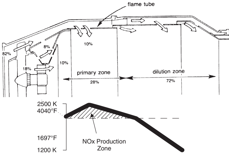
Figure 10-19. A typical combustor showing the \text{NO}_x production zone.
