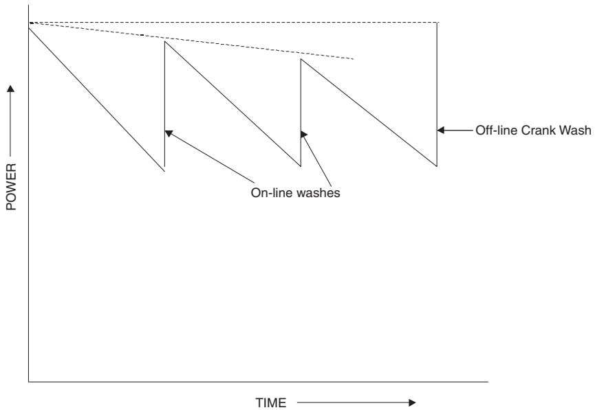
Figure 20-7. Compressor water wash characteristics.
