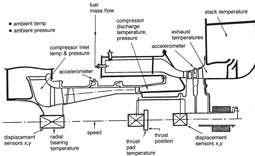
Figure 20-6. Gas turbine suggested measurement points.
