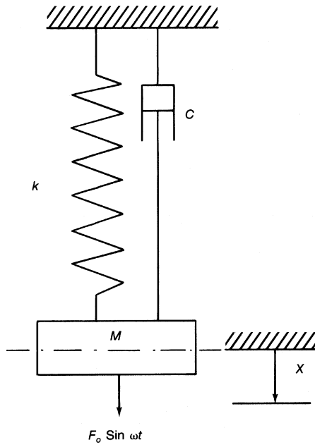
Figure 5-17. Forced vibration with viscous damping.
