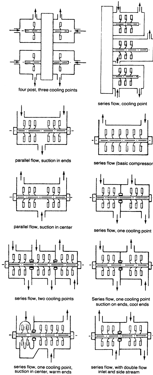
Figure 6-47. Various configurations of centrifugal compressors.
