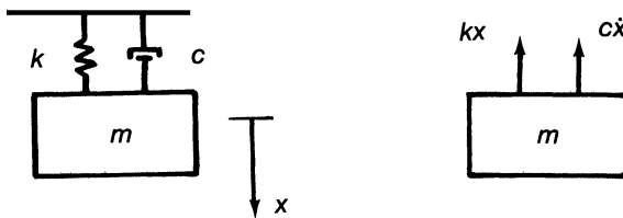
Figure 5-6. Free vibration with viscous damping.
