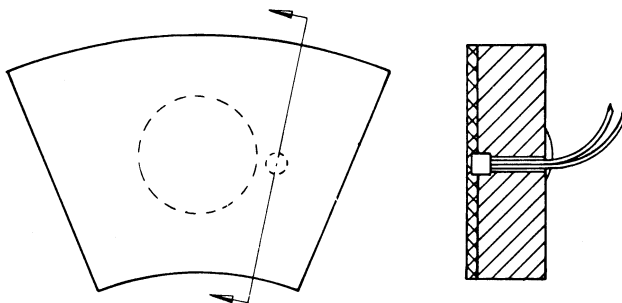
Figure 21-9. RTD embedded in bearing surface.
