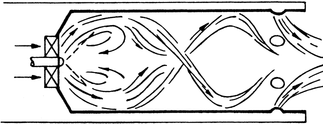
Figure 10-3. Flame stabilization region created by swirl vanes.
