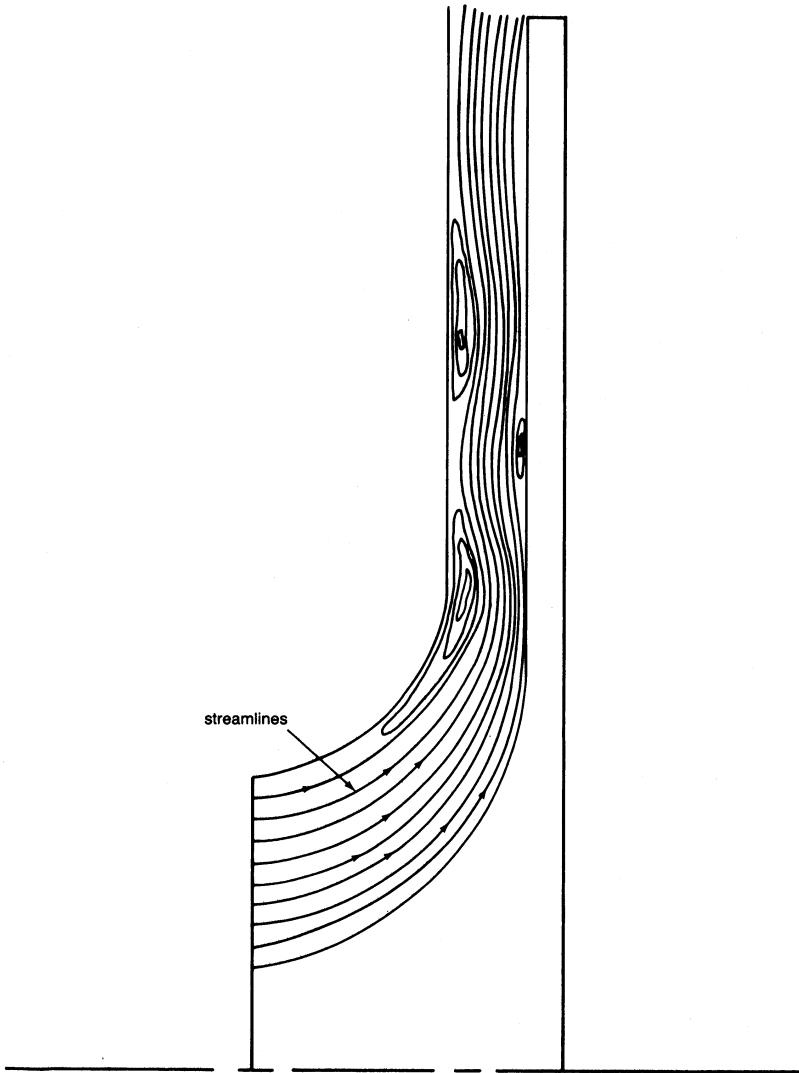
Figure 6-17. Flow map as seen in meridional plane.
