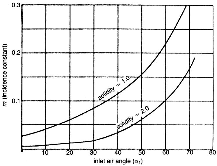
Figure 7-24. Slope of incidence angle variation with air angle.
