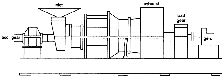
Figure 3-14. Typical industrial gas turbine.
