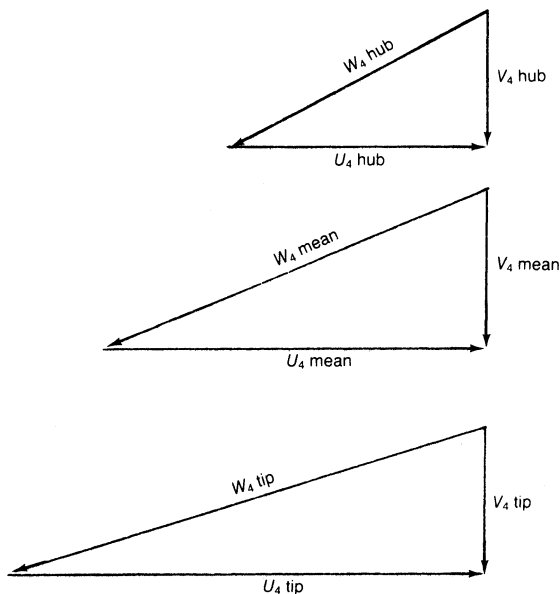
Figure 8-12. Exit velocity diagrams for a radial-inflow turbine.
