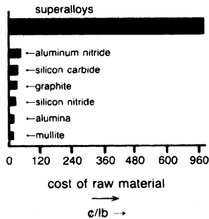
Figure 11-1c. A comparison of raw material costs.
