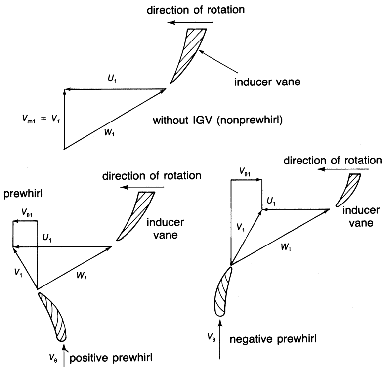
Figure 6-11. Inducer inlet velocity diagrams.
