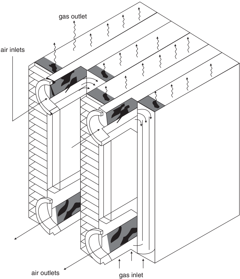
Figure 1-22. A typical plate and fin type regenerator for an industrial gas turbine.
