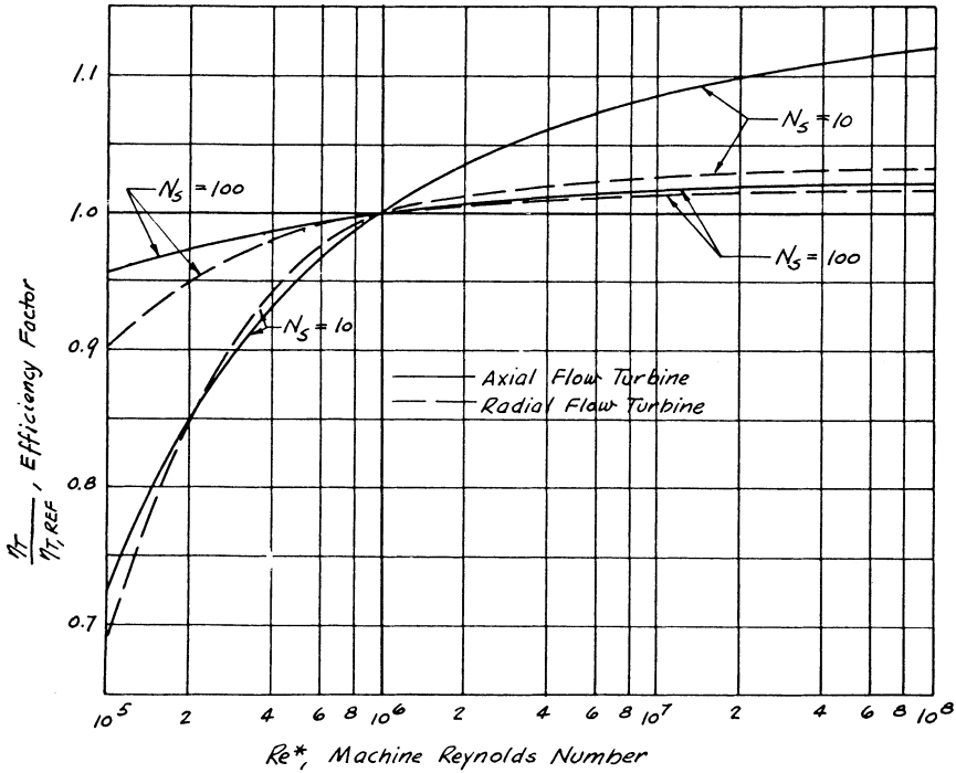
Figure 8-1. Influence of Reynolds number on turbine stage efficiency.
