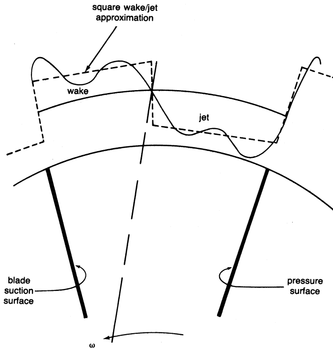
Figure 6-29. Jet-wake flow distribution from an impeller.
