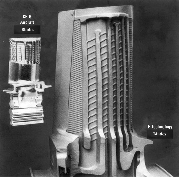
Figure 9-18. Internal of the frame FA blades, showing cooling passages. (Courtesy GE Power Systems.)
