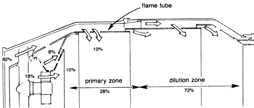
Figure 1-24. Air distribution in a typical combustor.
