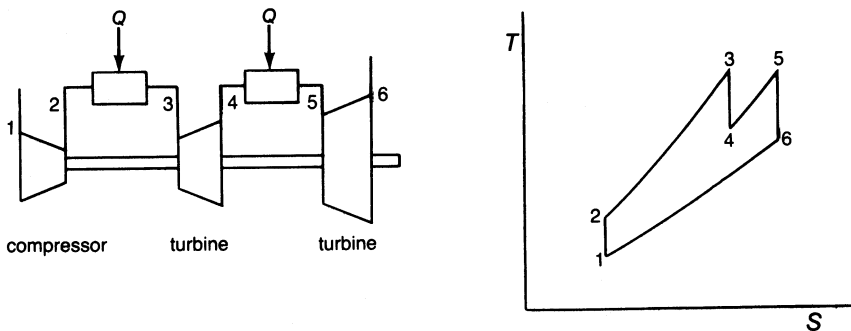
Figure 2-8. Reheat cycle and T-S diagram.
