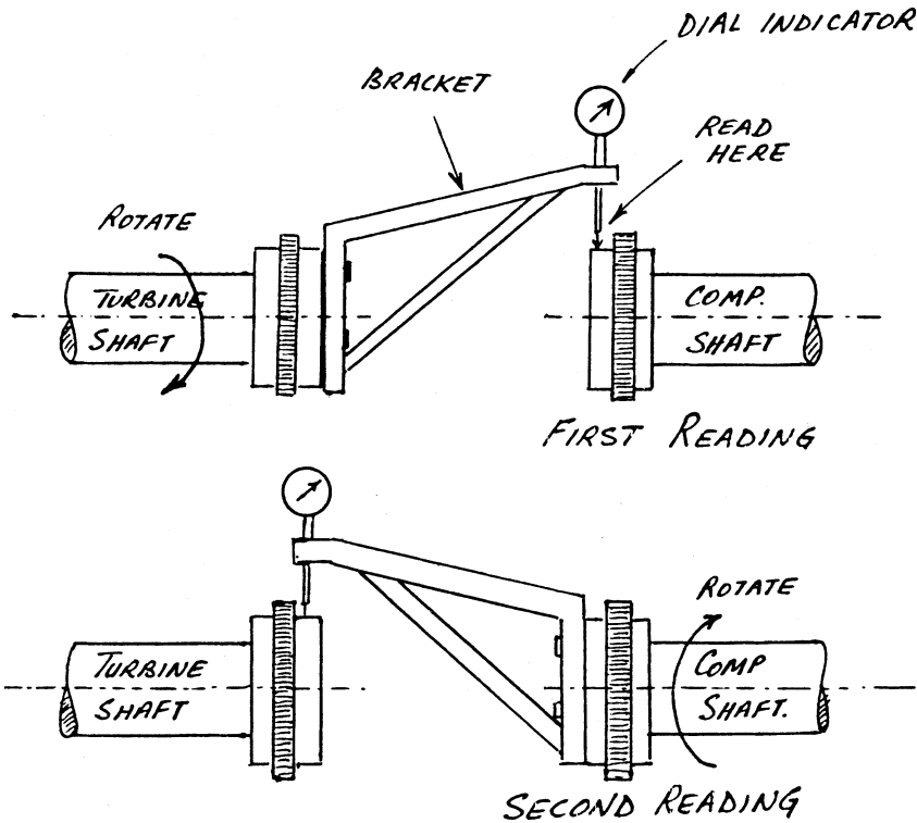
Figure 18-15. Reverse-dial indicator setup.
