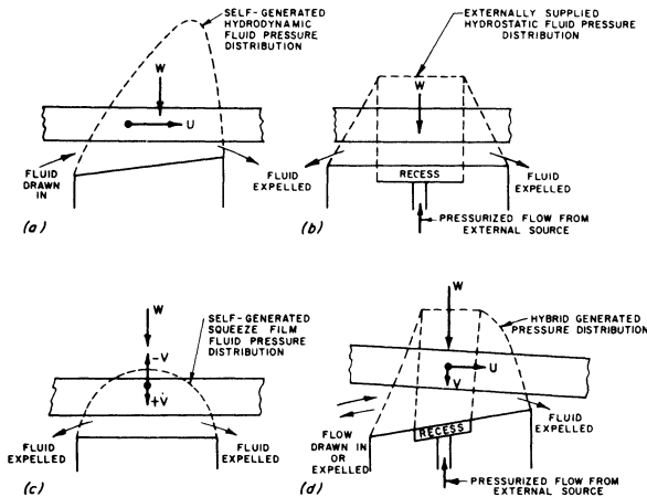
Figure 13-7. Modes of fluid-film lubrication: (a) hydrodynamic, (b) hydrostatic, (c) squeeze film, (d) hybrid.
