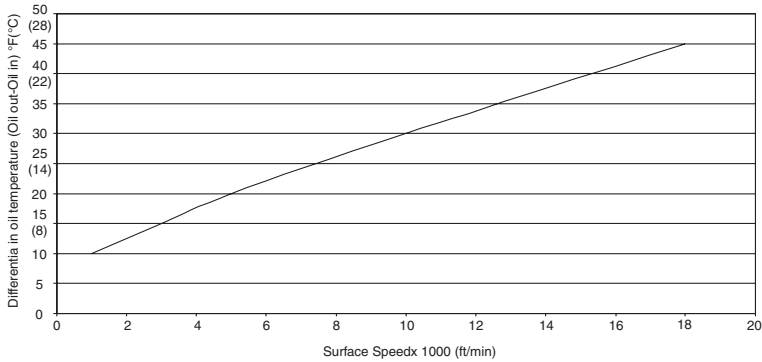
Figure 13-13. Oil discharge characteristics.
