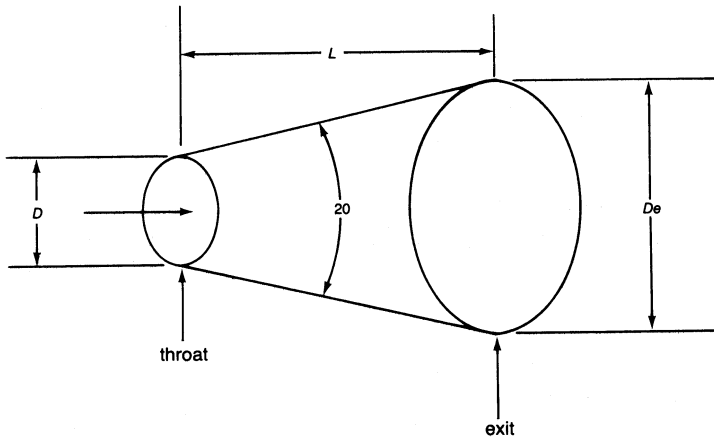
(b) straight-wall conical diffuser
