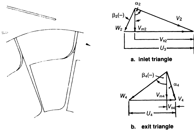
Figure 8-10. Velocity triangles for a radial-inflow turbine.
