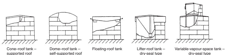
Figure 12-14. Some types of atmospheric storage tanks.
