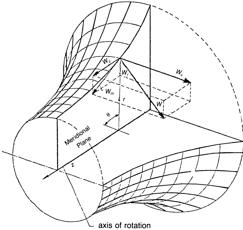
Figure 8-6. Velocity vectors in turbine rotor flow.
