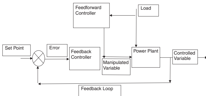
Figure 19-1. Forward and feed back control loop.
