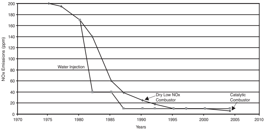
Figure 1-33. Control of gas turbine NO x emissions over the years.
