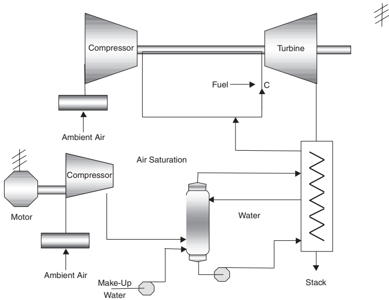
Figure 2-41. Heated and humidified compressed air injection system for power augmentation of a gas turbine.
