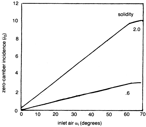
Figure 7-23. Incidence angle for zero-camber airfoil.
