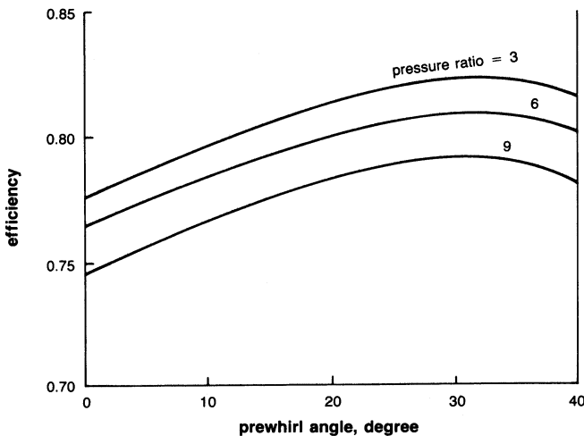
Figure 6-12. Estimated effect of inlet prewhirl. (Rodgers, C. and Shapiro, L., “Design Considerations for High-Pressure-Ratio Centrifugal Compressors,” ASME Paper No.: 73-GT-31.)
