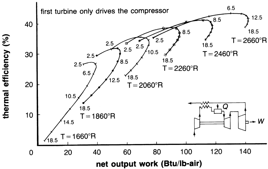
Figure 2-14. Performance map showing the effect of pressure ratio and turbine inlet temperature on a regenerative split shaft cycle.
