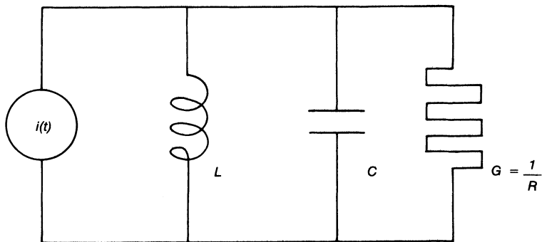
Figure 5-19. Force-current analogy.
