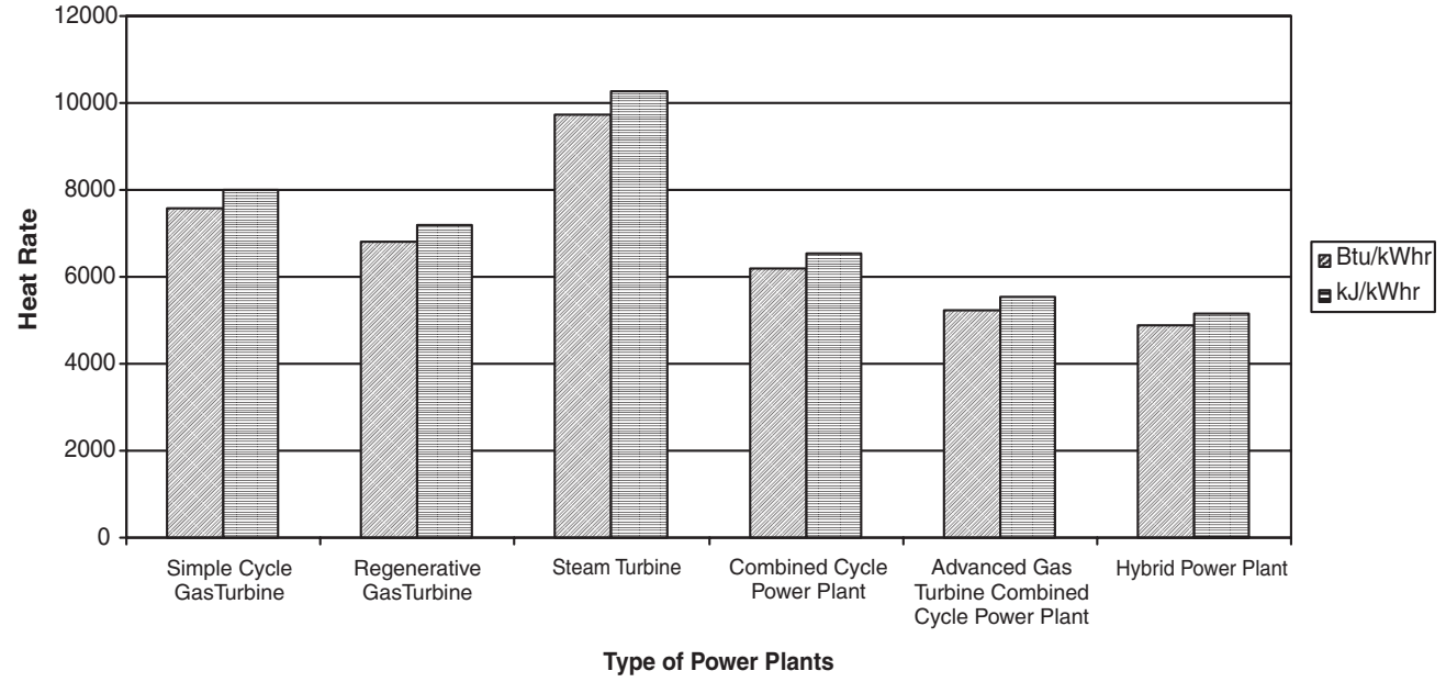
Figure 1-1. Typical heat rates of various types of plants.
