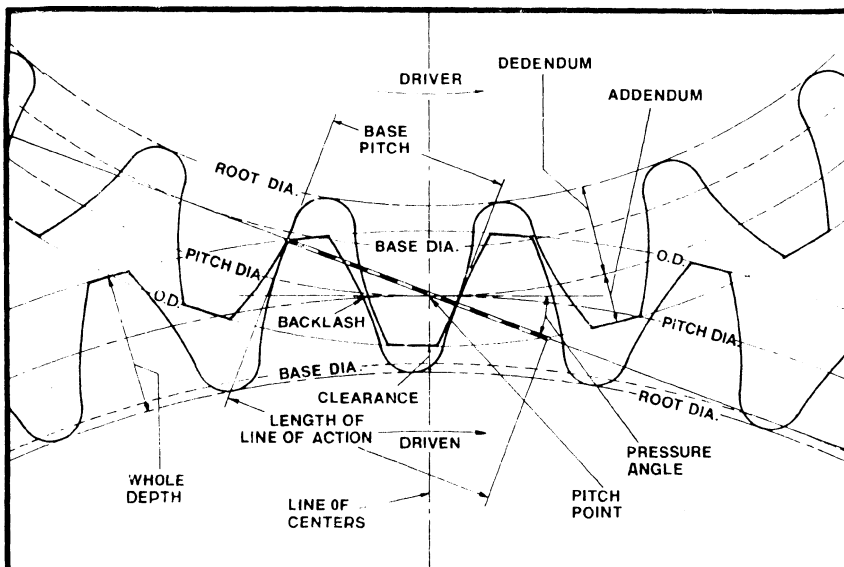
Figure 14-1. Transverse section through gear and pinion mesh.
