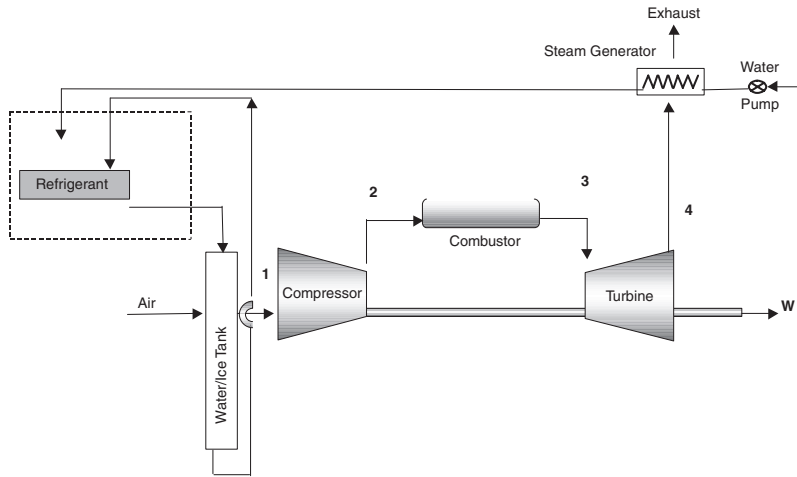
Figure 2-39. Thermal storage inlet system.
