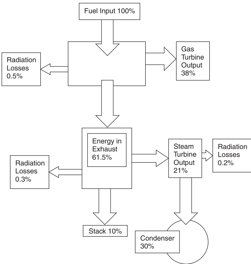
Figure 2-30. Energy distribution in a combined cycle power plant.
