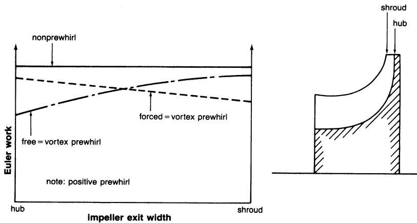
Figure 6-14. Euler work distribution at an impeller exit.
