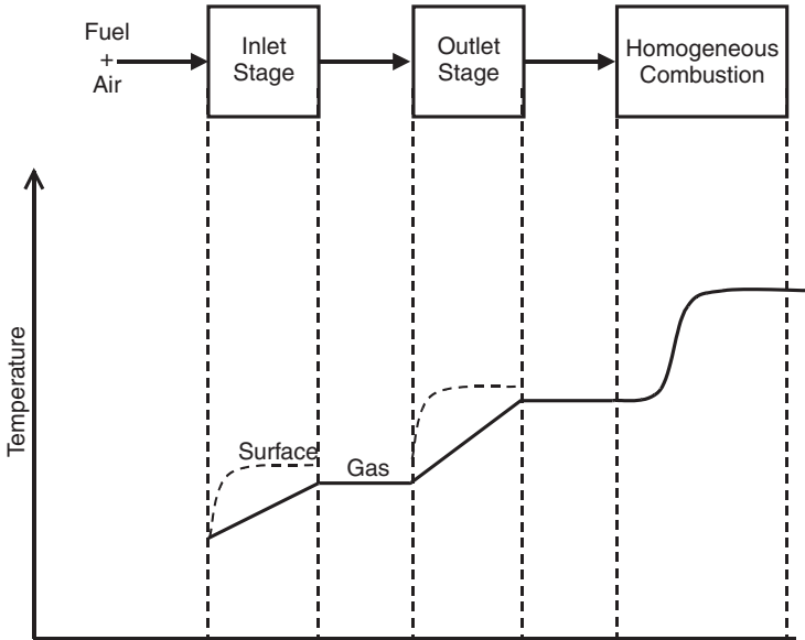
Figure 10-27. Schematic temperature profiles for catalytic combustion system in which the wall temperature is limited and complete combustion occurs after the catalyst.
