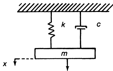
Figure 5-10. Forced vibration system.
