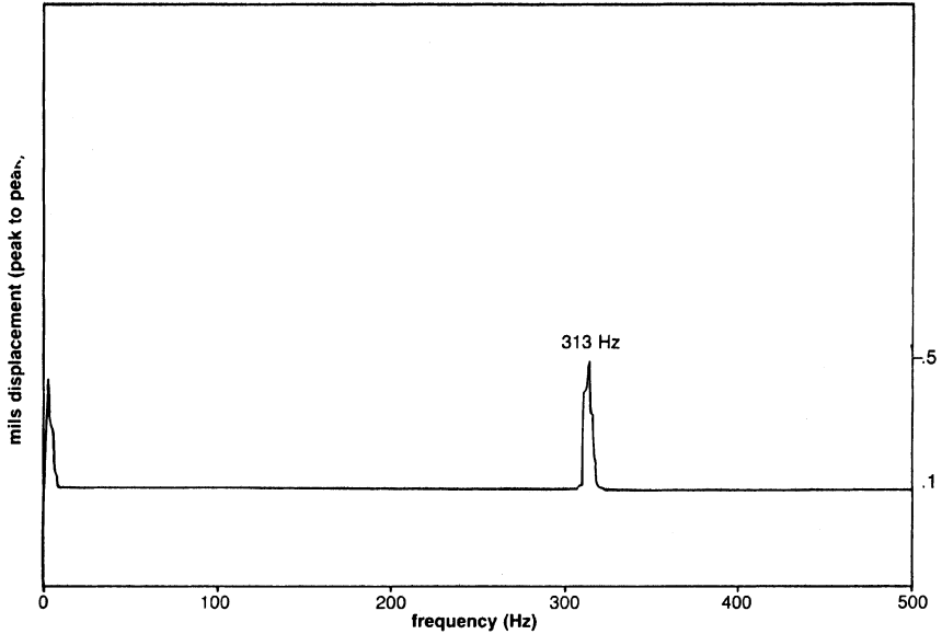
Figure 16-5. Vibration spectrum (rpm = 20,000, P_d = 1200 psig).
