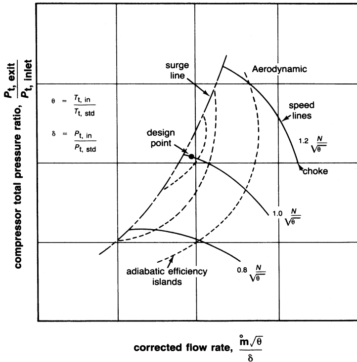
Figure 3-9. Typical centrifugal compressor performance characteristics.
