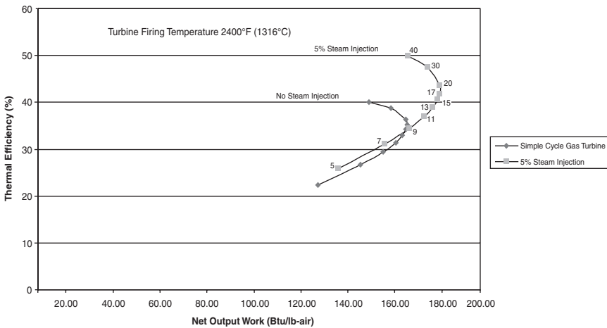
Figure 2-21. Comparison between 5% steam injection and simple cycle gas turbine.
