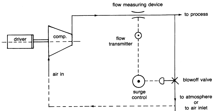
Figure 6-42. Flow-oriented anti-surge control system.
