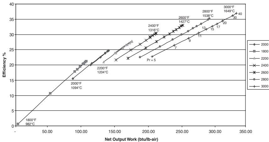
Figure 2-17. The performance of a reheat gas turbine cycle.
