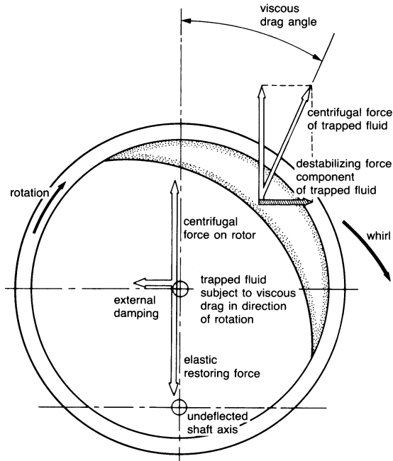
Figure 5-24. Whirl from fluid trapped in the rotor. (Ehrich, F.F., "Identification and Avoidance of Instabilities and Self-Excited Vibrations in Rotating Machinery," Adopted from ASME Paper 72-DE-21, General Electric Co., Aircraft Engine Group, Group Engineering Division, May 11, 1972.)
