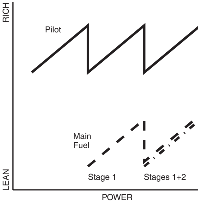
Figure 10-25. Shows the staging of dry low emissions combustor as the turbine is brought to full power.
