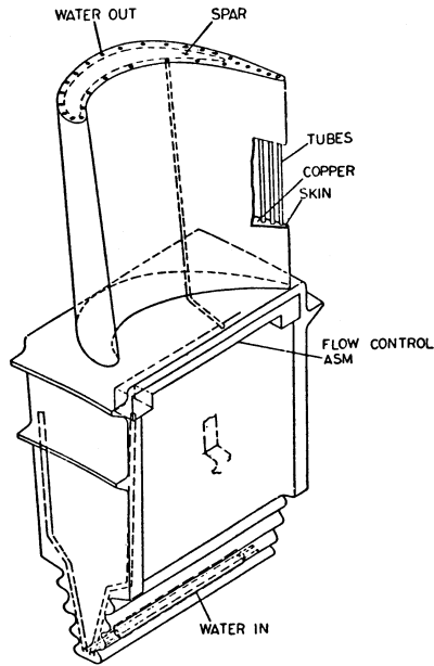
Figure 9-23. Water-cooled turbine blade. (Courtesy General Electric Company.)
