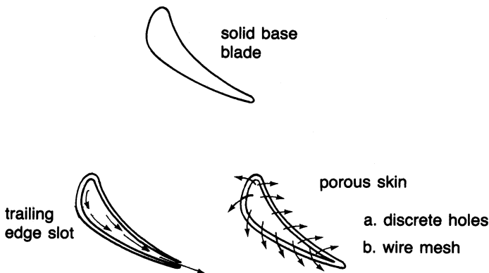
Figure 9-24. Cooled turbine blade types.
