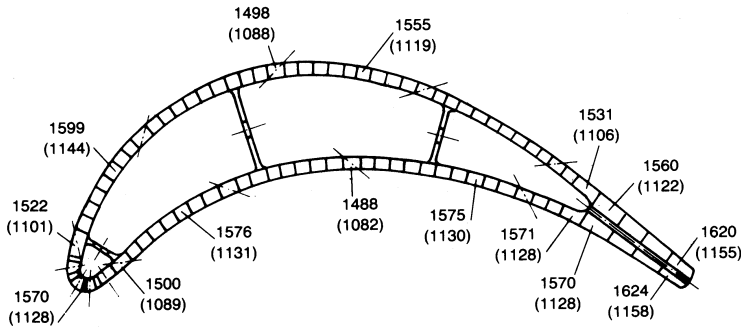
Figure 9-22. Temperature distribution for a multiple small-hole design, °F (cooled).
