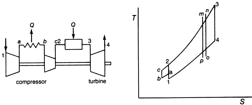
Figure 2-7. The intercooled gas turbine cycle.
