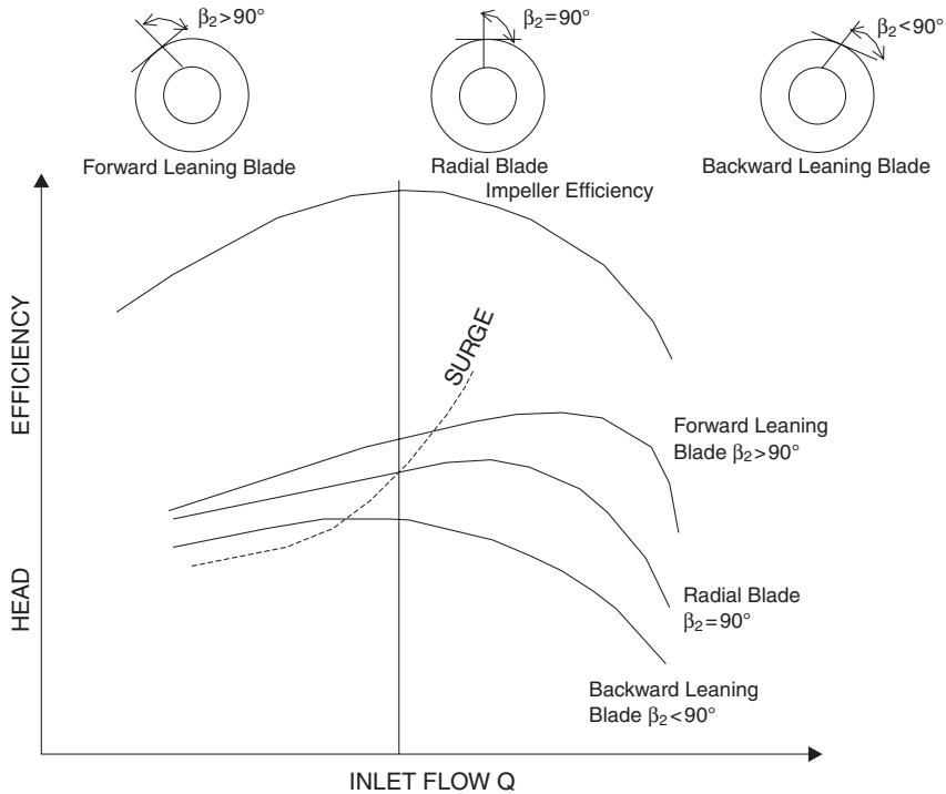
Figure 6-37. Effect of blade angle on stability.
