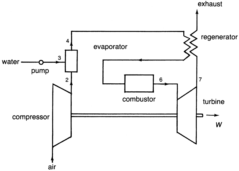
Figure 2-23. The evaporative regenerative cycle.
