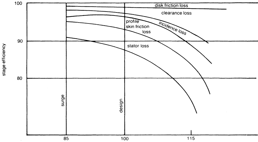
Figure 7-33. Losses in an axial-flow compressor stage.
