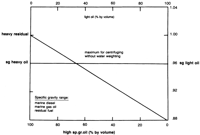
Figure 12-6. Fuel blending for specific gravity reduction. Specific gravity heavy oil = 1.0. Specific gravity light oil = .88.
