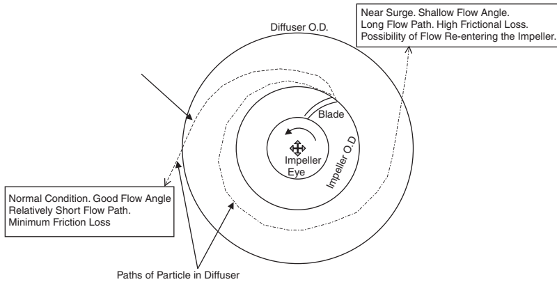
Figure 6-38. Flow trajectory in a vaneless diffuser.
