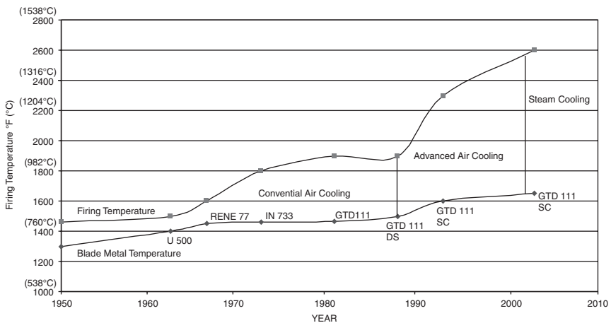
Figure 9-12. Firing temperature increase with blade material improvement.
