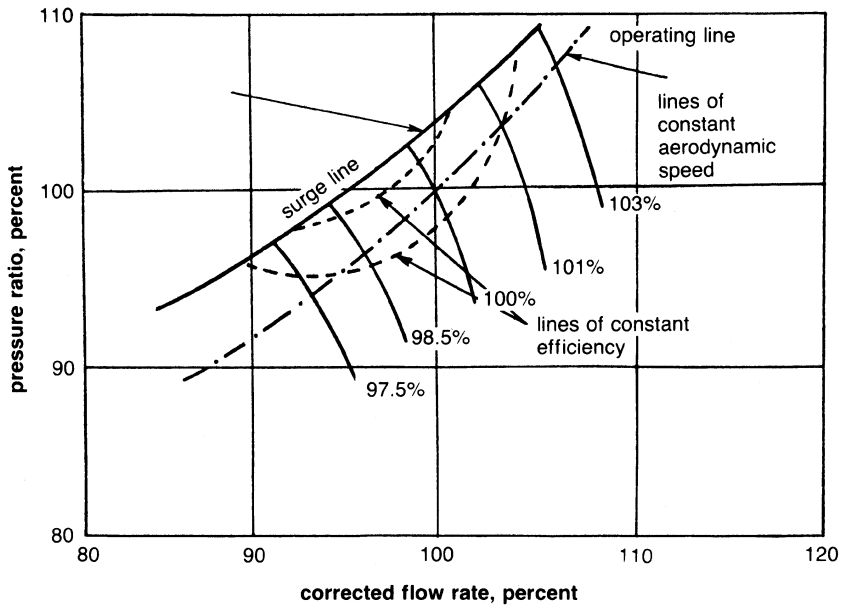
Figure 19-19. Typical compressor map.
