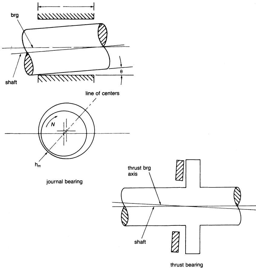
Figure 18-13. Misalignment in both journal and thrust bearings.
