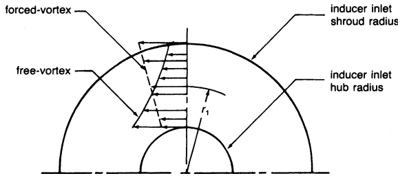
Figure 6-13. Prewhirl distribution patterns.
