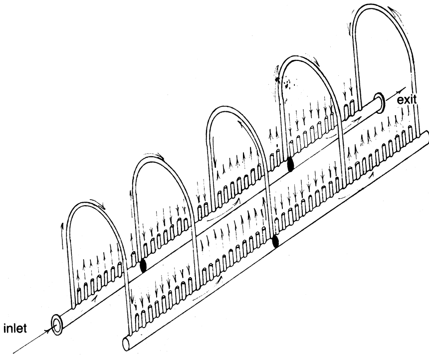
Figure 1-29. An external fired combustor with four passes.
