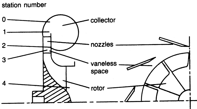
Figure 1-36. Components of a Radial Inflow Turbine.
