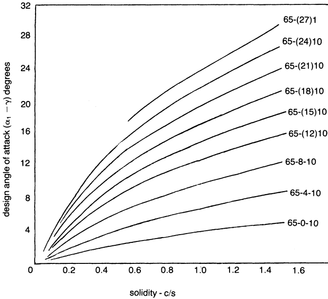
Figure 7-31. Design angles of attack (\alpha_1 - \gamma) for NACA 65 series.
