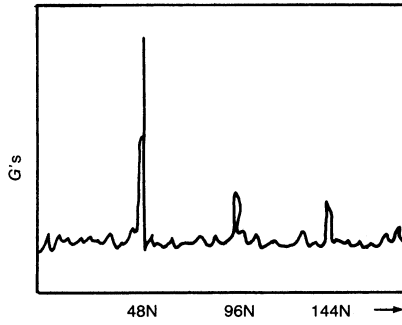
Figure 7-37. High-pressure bleed chamber—8000 rpm.
