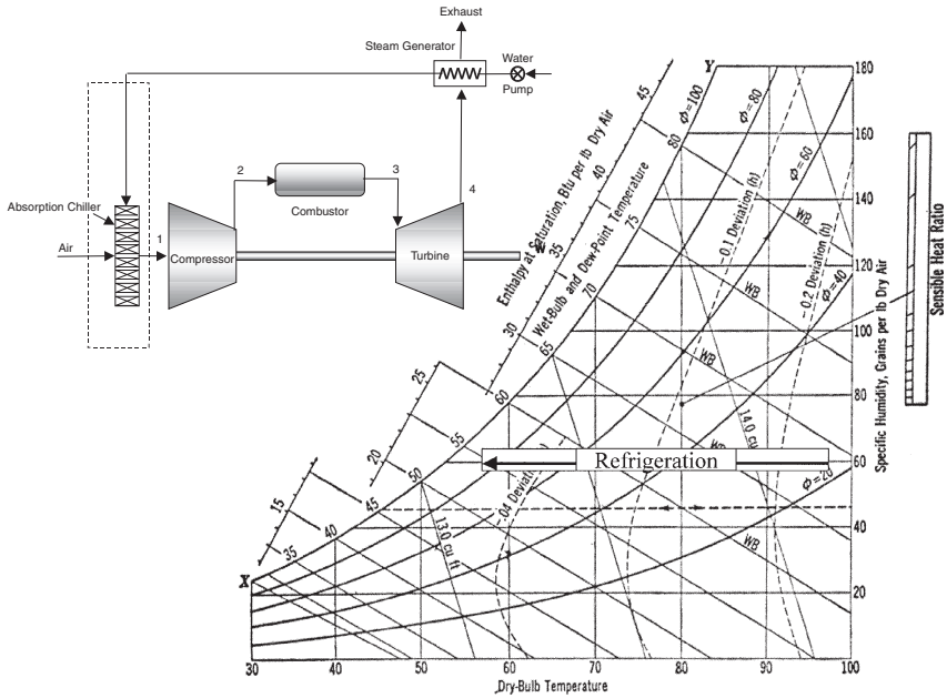
Figure 2-37. Absorption refrigerated inlet cooling system.
