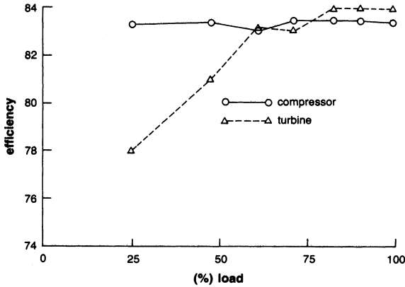
Figure 3-16. Compressor and turbine efficiency as a function of load.
