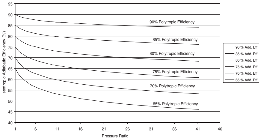
Figure 3-6. Relationship between adiabatic and polytropic efficiency.
