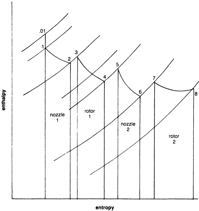
Figure 8-9. Enthalpy-entropy diagram for a multistage turbine.
