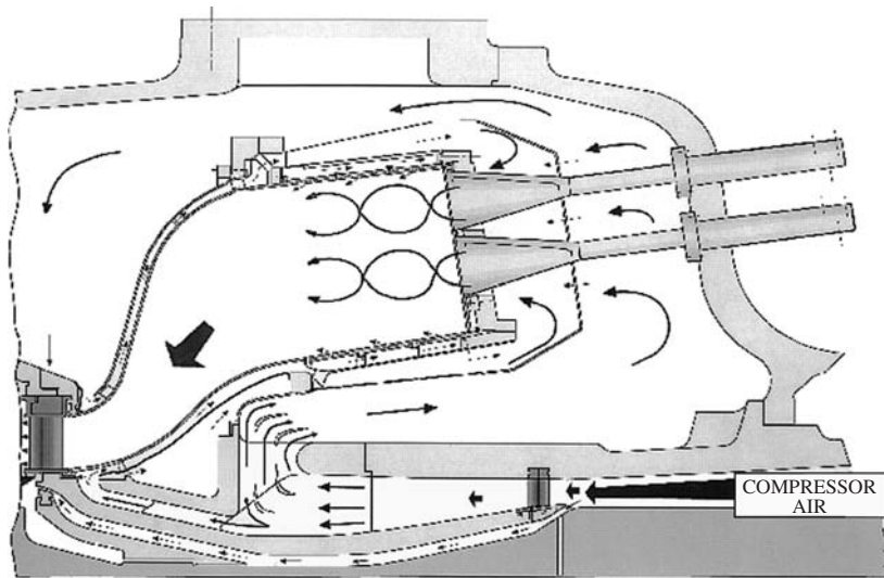
Figure 10-24. Schematic of a dry low emission \text{NO}_x combustor (Courtesy ALSTOM.)
