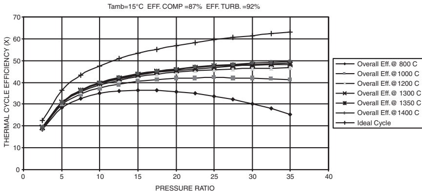
Figure 1-5. Overall cycle efficiency.
