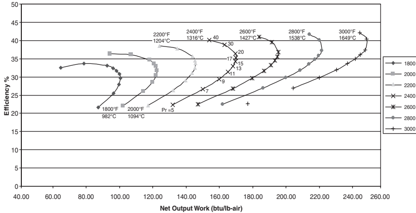
Figure 2-10. The performance map of a simple cycle gas turbine.
