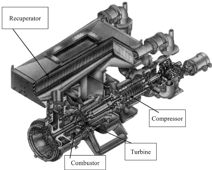
Figure 1-12. A recuperative medium-sized industrial gas turbine. (Courtesy Solar Turbines Incorporated.)
