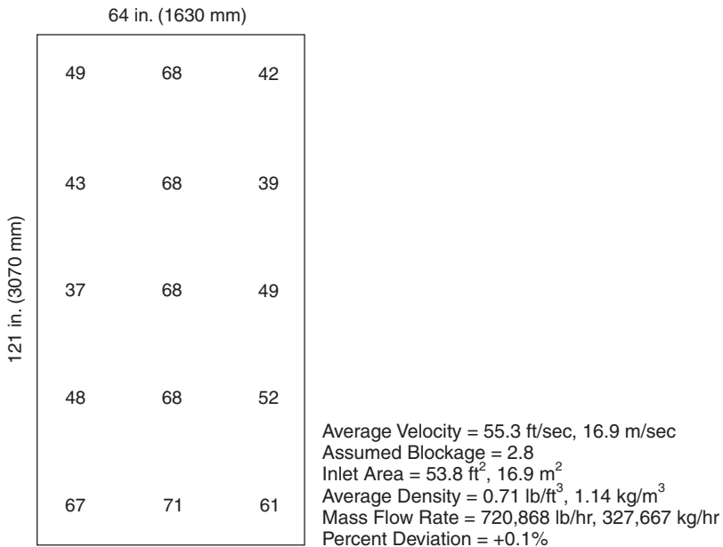
Figure 3-18. Typical inlet velocity profile for an industrial gas turbine.
