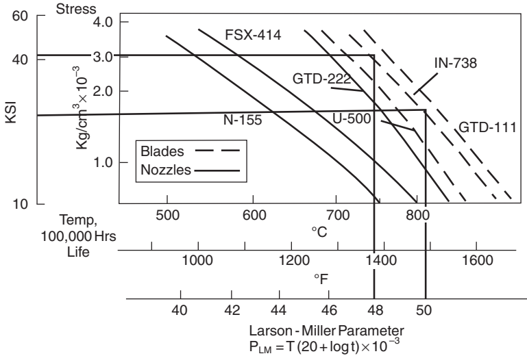
Figure 11-4. Larson-Miller parameter for various types of blades.
