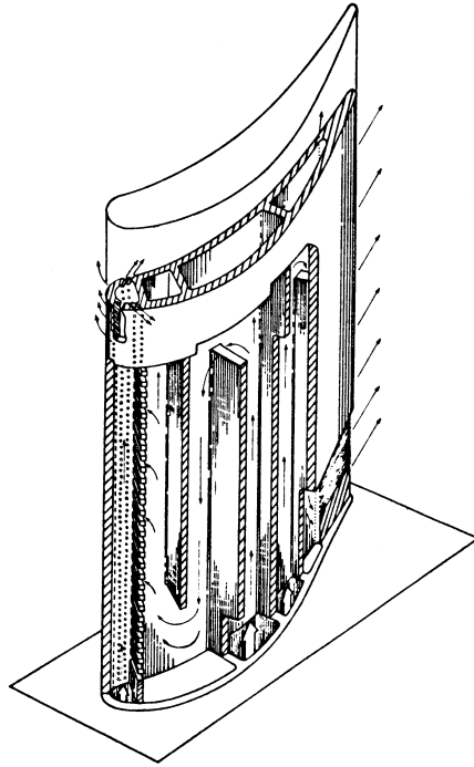
Figure 9-16. Film and convection-cooled blade.
