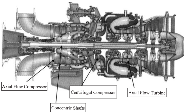
Figure 1-14. A small aeroderivative gas turbine. (Courtesy Pratt & Whitney Canada Corp.)
