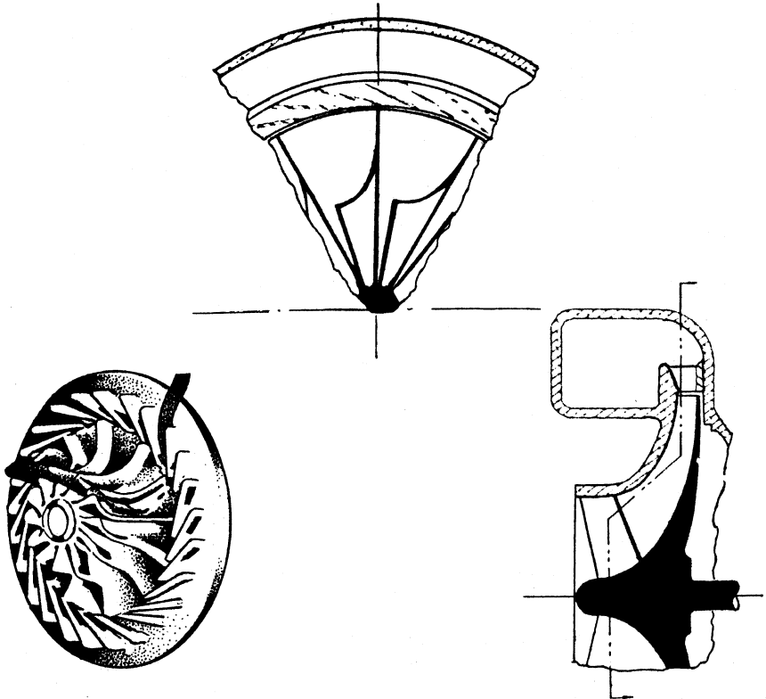
Figure 1-35. Mixed flow type radial inflow turbine.
