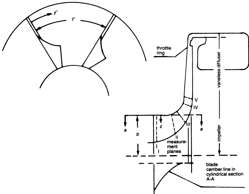
Figure 6-18. Velocity profiles through a centrifugal compressor.
