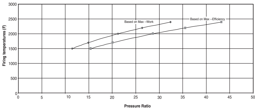
Figure 2-3. Pressure ratio based on maximum efficiency or work at various firing temperatures. Based on a compressor efficiency of 87% and a turbine efficiency of 92%.
