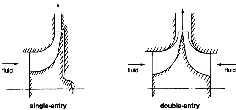
Figure 6-7. Types of entry-inducer systems.
