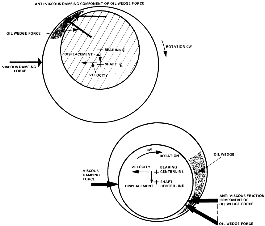
Figure 13-15. Oil whirl.
