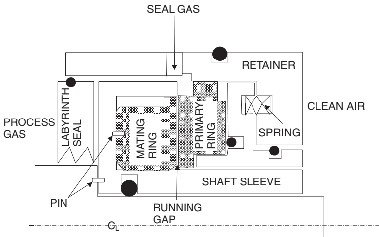
Figure 13-35. Single dry gas seal.
