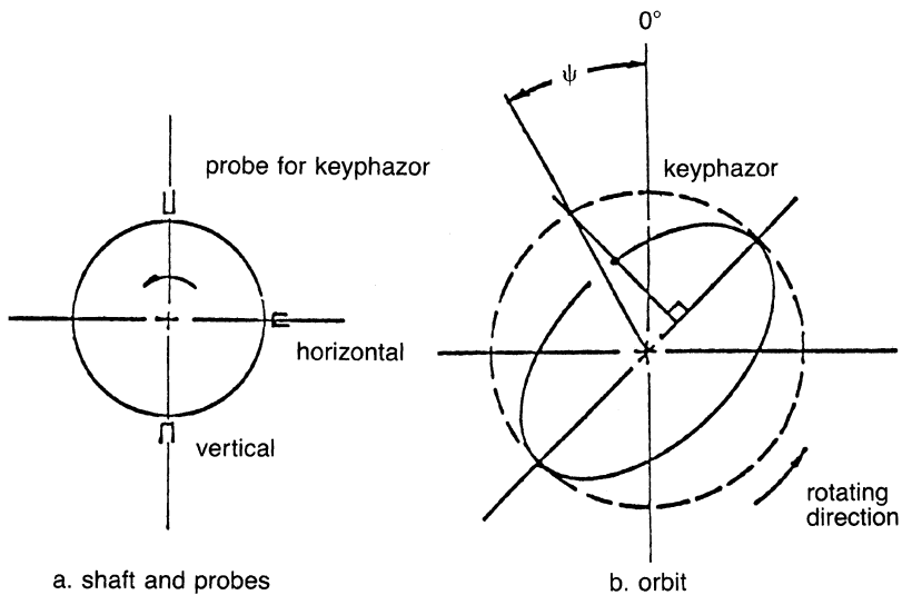
Figure 17-7. Typical probe positions and the phase angle in an elliptic orbit.
