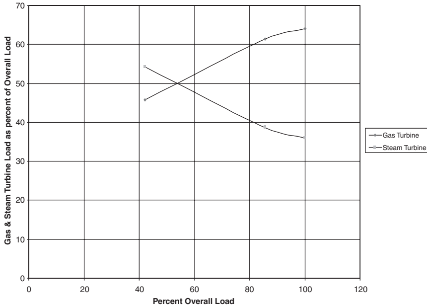
Figure 2-31. Load sharing between prime movers over the entire operating range of a combine cycle power plant.
