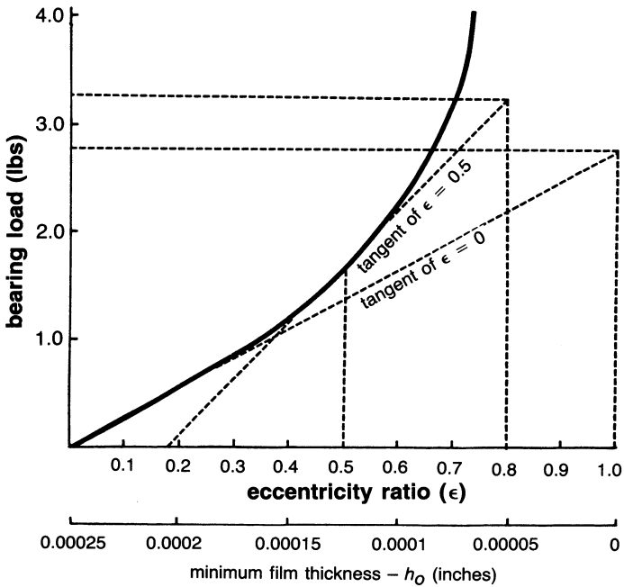
Figure 13-11. Journal bearing load capacity versus minimum film thickness and eccentricity ratio.
