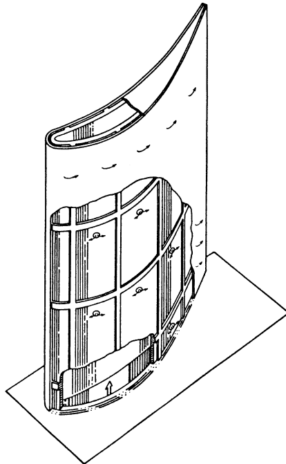
Figure 9-19. Transpiration-cooled blade.
