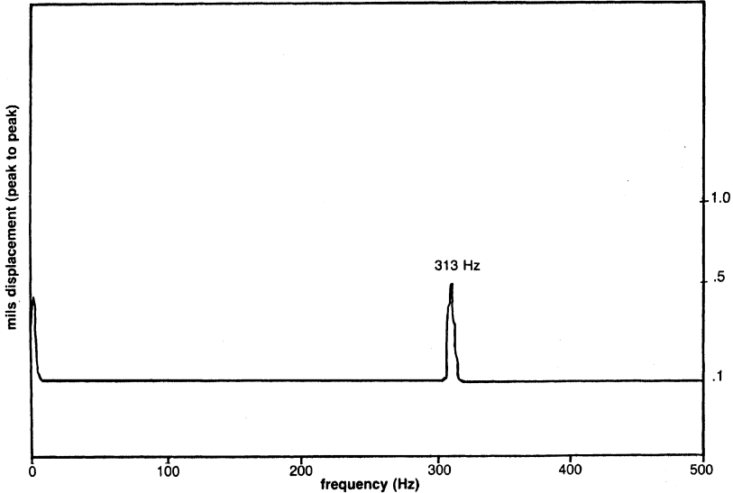
Figure 16-8. Vibration spectrum (rpm = 20,000, P_d = 1320 psig).
