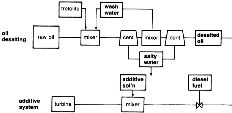
Figure 12-5. A typical residual fuel treatment system.
