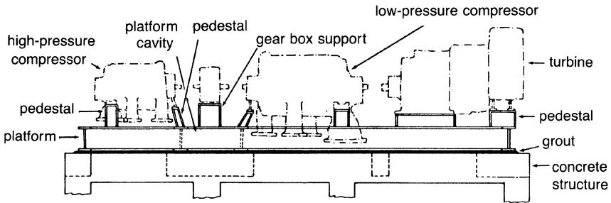
Figure 21-14. A typical compressor train containing a turbine and two compressor stages.
