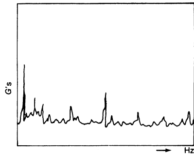
Figure 7-39. Fifth-stage bleed pressure—5800 rpm.
