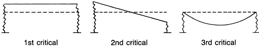
Figure 5-16b. Flexible supports and rigid rotors.
