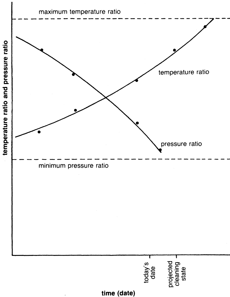
Figure 19-17. Data trending to predict maintenance schedules.
