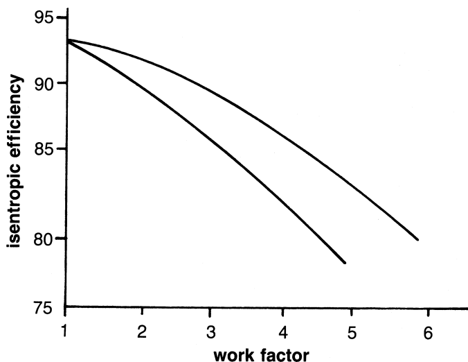
Figure 9-3. Effect of stage work on efficiency.
