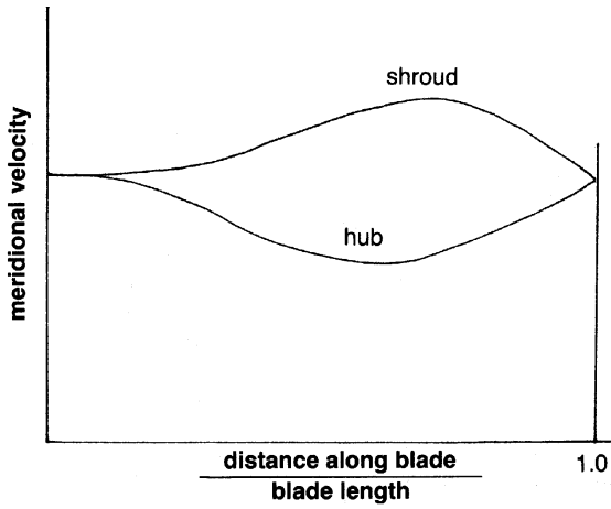
Figure 8-14. Meridional velocity distribution from hub to shroud along the blade length.
