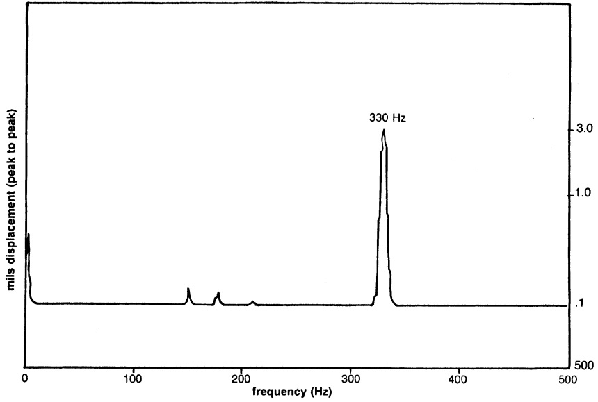
Figure 16-6. Vibration spectrum (rpm = 20,000, P_d = 1250 psig).
