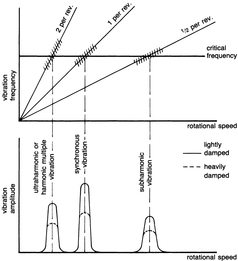
Figure 5-20. Characteristic of forced vibration or resonance in rotating machinery. (Ehrich, F.F., "Identification and Avoidance of Instabilities and Self-Excited Vibrations in Rotating Machinery," Adopted from ASME Paper 72-DE-21, General Electric Co., Aircraft Engine Group, Group Engineering Division, May 11, 1972.)
