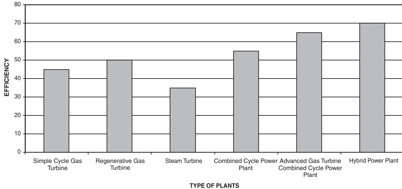
Figure 1-2. Typical efficiencies of various types of plants.
