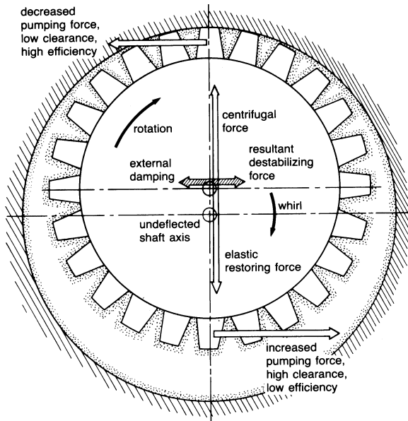
Figure 5-23b. Aerodynamic cross-coupling. (Ehrich, F.F., "Identification and Avoidance of Instabilities and Self-Excited Vibrations in Rotating Machinery," Adopted from ASME Paper 72-DE-21, General Electric Co., Aircraft Engine Group, Group Engineering Division, May 11, 1972.)
