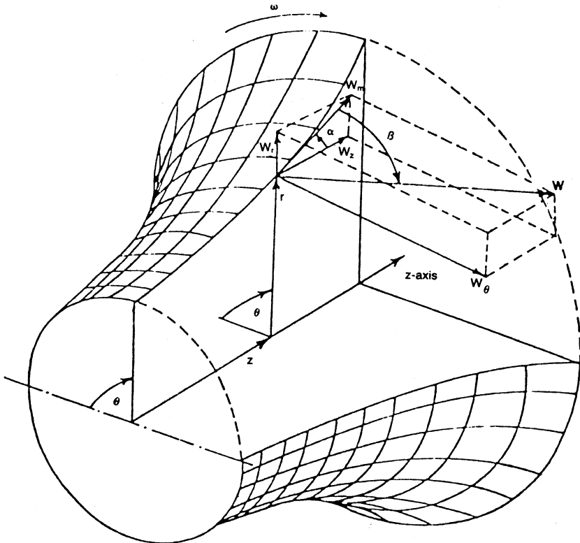
Figure 3-2. Velocity vectors in compressor rotor flow.
