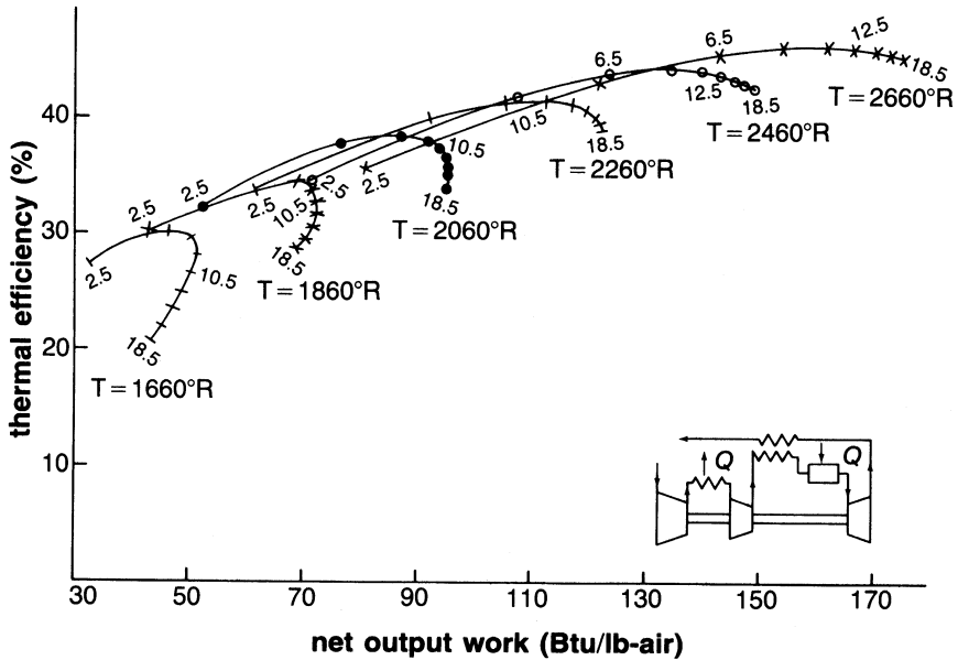
Figure 2-16. Performance map showing the effect of pressure ratio and turbine inlet temperature on an intercooled regenerative cycle.
