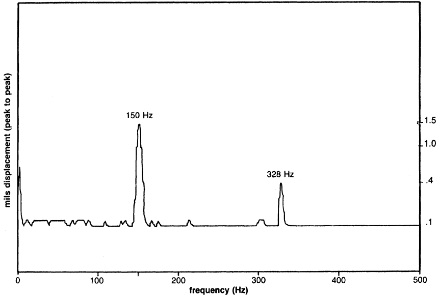
Figure 16-7. Vibration spectrum (rpm = 20,000, P_d = 1270 psig).
