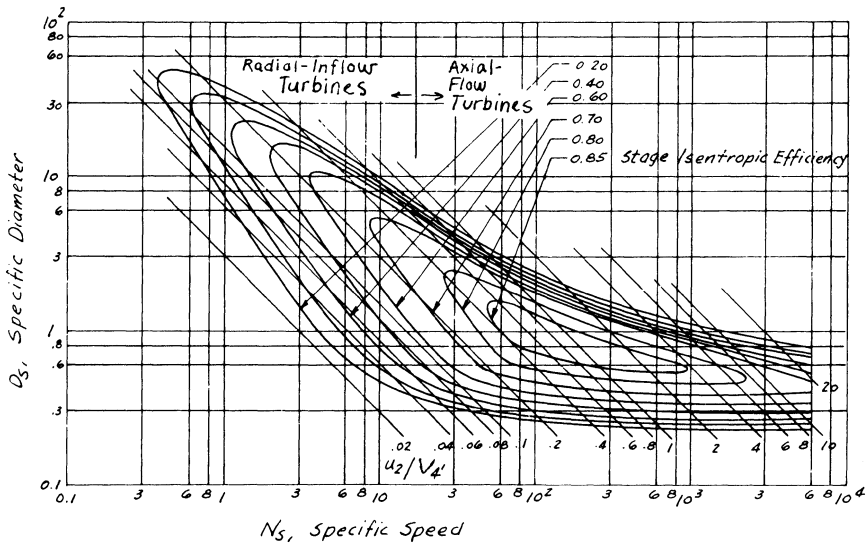
Figure 8-2. N_s D_s diagram for a turbine stage. Efficiency is on a total-to-total basis; that is, it is related to inlet and exit stagnation conditions. Diagram values are suitable for machine Reynolds number Re \geq 10^6 . (Balje, O.E., "A Study of Reynolds Number Effects in Turbomachinery," Journal of Engineering for Power, ASME Trans., Vol. 86, Series A, p. 227.)
