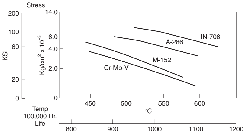
Figure 11-6. Turbine Wheel Alloys stress rupture comparison.
