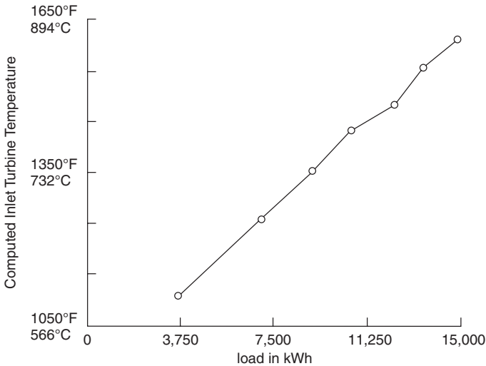
Figure 3-17. Turbine inlet temperature as a function of turbine load.
