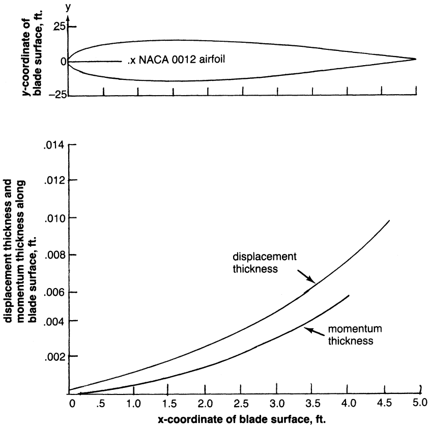
Figure 9-26. Growth of displacement and momentum thickness on an airfoil.
