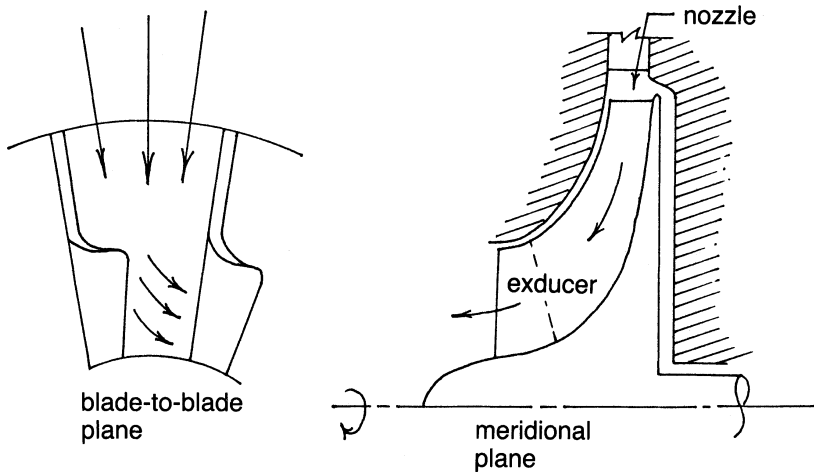
Figure 8-13. The two major flow planes in a radial-inflow turbine.
