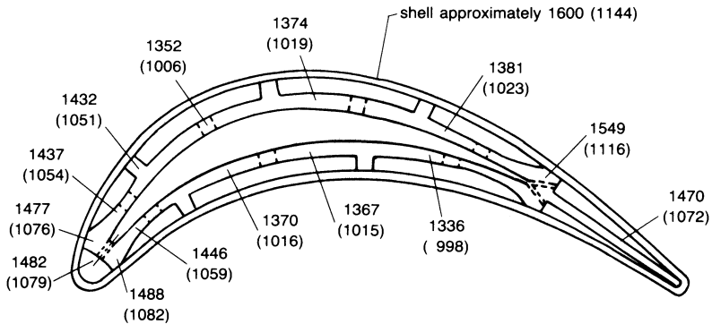
Figure 9-20. Temperature distribution for transpiration-cooled design, °F (cooled).
