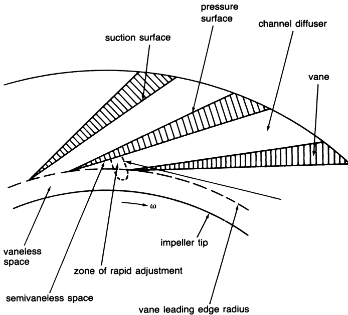
Figure 6-28. Flow regions of the vane diffuser.
