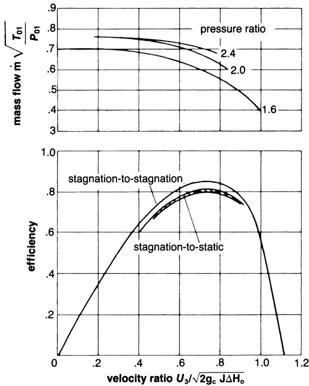
Figure 8-11. An example of a radial-inflow turbine characteristic. (Courtesy Institution of Mechanical Engineers.)
