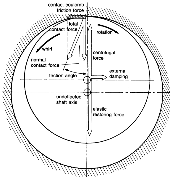
Figure 5-22b. Dry friction whirl. (Ehrich, F.F., "Identification and Avoidance of Instabilities and Self-Excited Vibrations in Rotating Machinery," Adopted from ASME Paper 72-DE-21, General Electric Co., Aircraft Engine Group, Group Engineering Division, May 11, 1972.)
