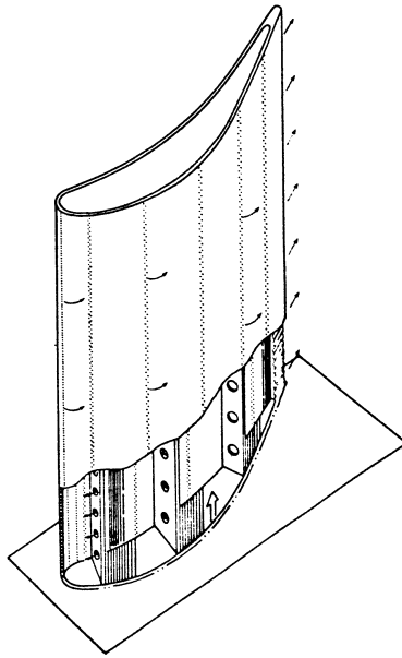
Figure 9-21. Multiple small hole transpiration-cooled blade.
