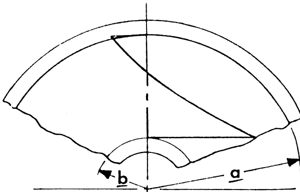
Figure 18-9. Stress distribution under axial deflection.
