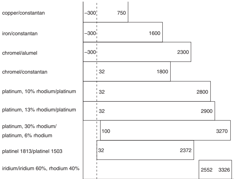
Figure 19-12. Ranges of various thermocouples.
