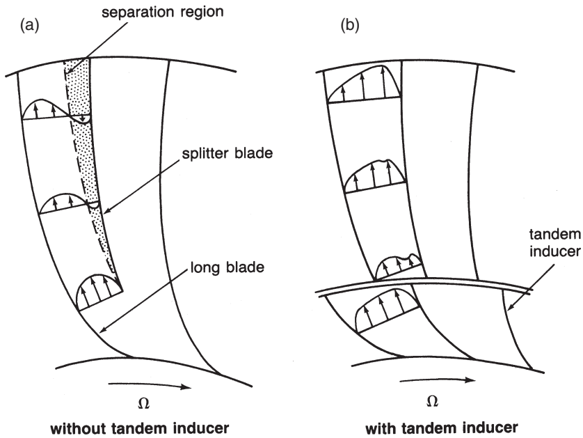
Figure 6-20. Impeller channel flow.
