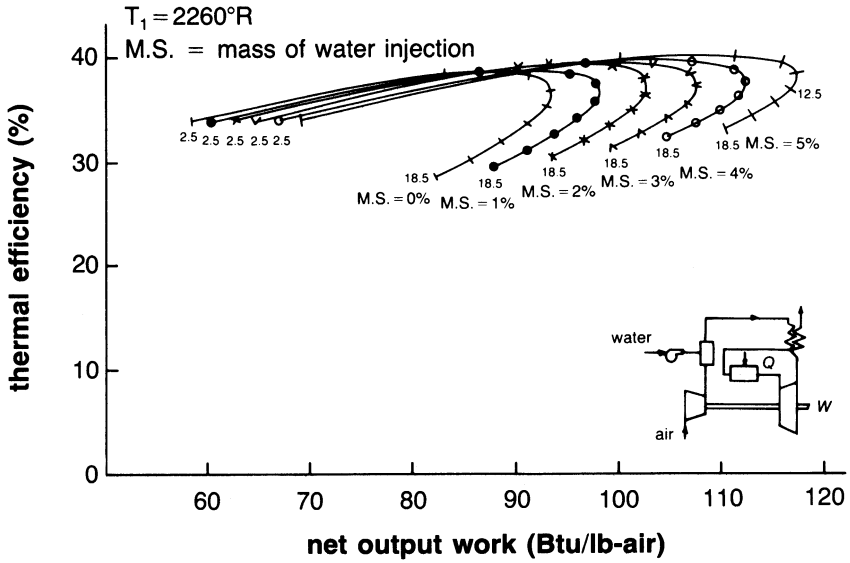
Figure 2-24. Performance map showing the effect of pressure ratio and steam flow rate on an evaporative regenerative cycle.
