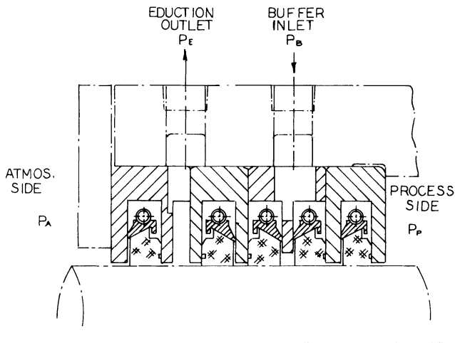
Figure 13-31. Restrictive ring seal system with both buffer and eduction cavities.
