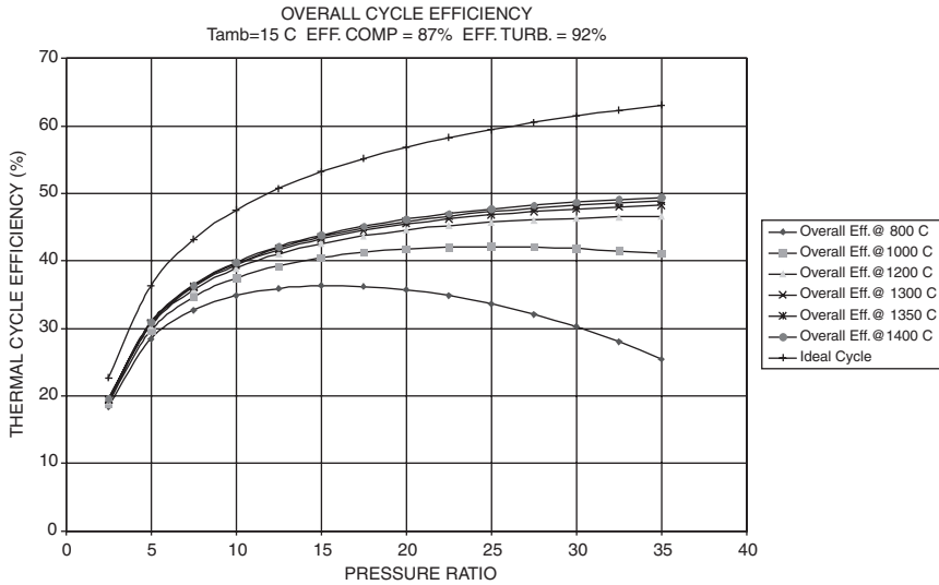
Figure 20-9. Effect of pressure ratio and firing temperature on the performance of a gas turbine.
