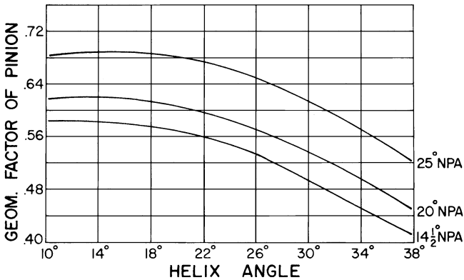
Figure 14-5. Variation of gear tooth geometry with pressure angle and helix angle. (Courtesy of Lufkin Industries, Inc.)
