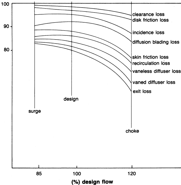
Figure 6-35. Losses in a centrifugal compressor.
