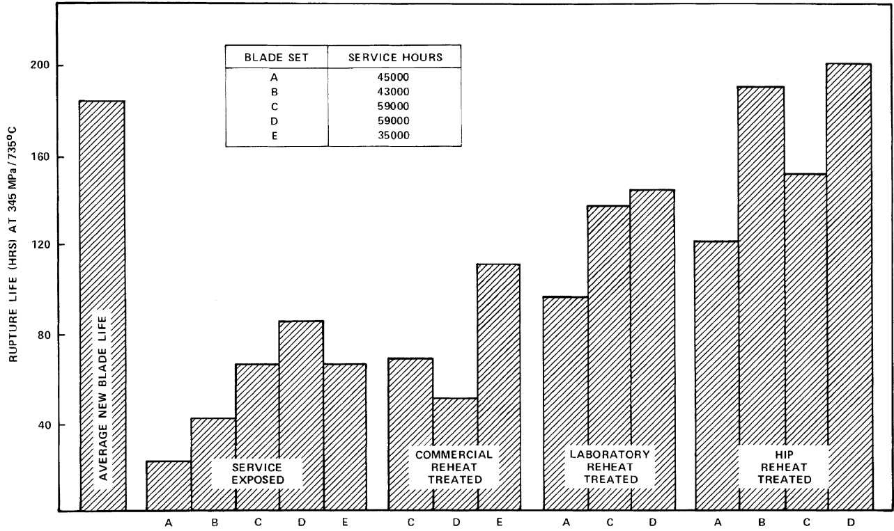
Figure 21-13. Comparison of stress rupture life at 50 ksi/1350°F (345 MPa/735°C) in service exposed, commercially reheat-treated, laboratory reheat-treated, and HIP reheat-treated used Inconel X-750 turbine blades. (Courtesy of Westinghouse Electric Corp., Gas Turbine Div.)
