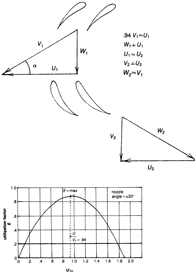
Figure 9-11. The effect of exit velocity and air angle on the utilization factor.
