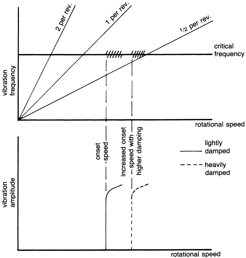
Figure 5-21. Characteristics of instabilities or self-excited vibration in rotating machinery. (Ehrich, F.F., "Identification and Avoidance of Instabilities and Self-Excited Vibrations in Rotating Machinery," Adopted from ASME Paper 72-DE-21, General Electric Co., Aircraft Engine Group, Group Engineering Division, May 11, 1972.)
