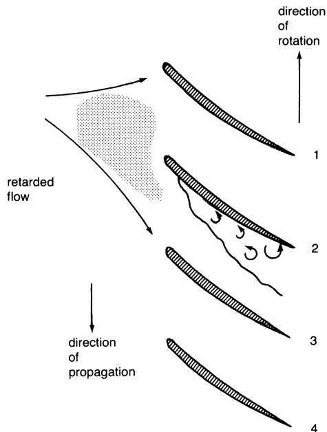
Figure 7-32. Propagating stall in a cascade.
