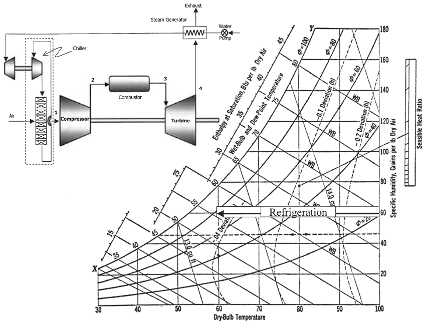
Figure 2-36. Mechanical refrigerated inlet system used to cool the inlet air of the gas turbine.
