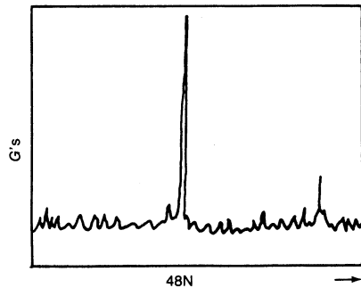
Figure 7-36. High-pressure bleed chamber—5400 rpm.
