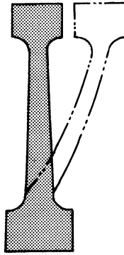
Figure 18-8. Axial deflection in a disc.
