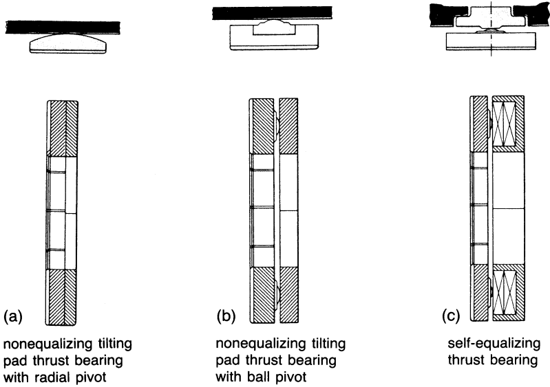
Figure 13-18. Various types of thrust bearings.
