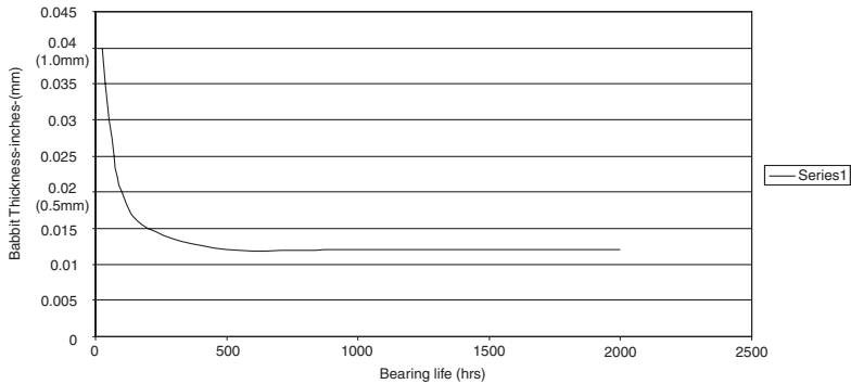
Figure 13-14. Babbitt fatigue characteristics.
