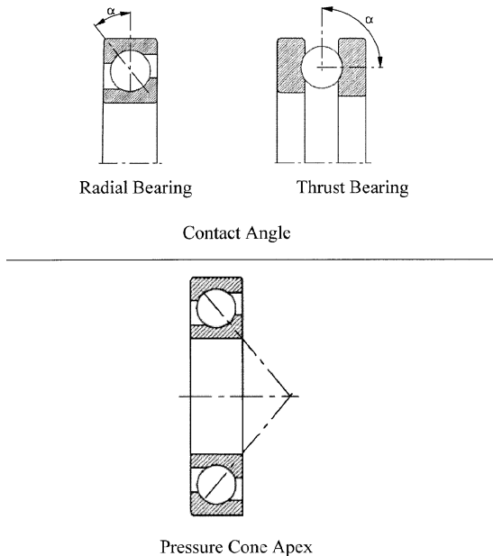
Figure 13-2. Rolling bearing terminology. (Courtesy FAG bearings.)
