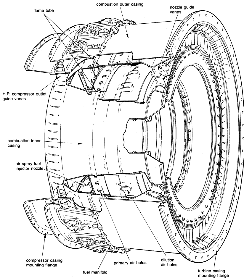
Figure 1-27. Annular combustion chamber.
