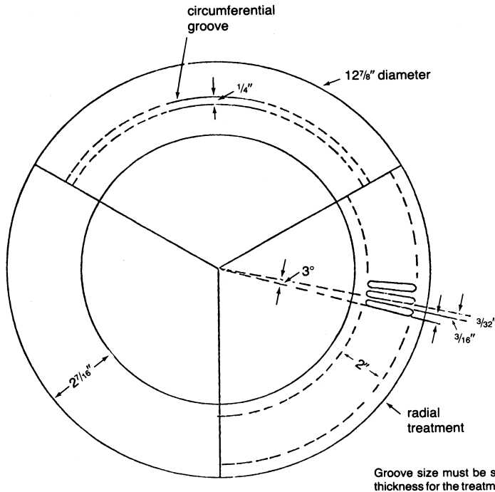
Figure 7-13. Details of the various casing treatments. Each treatment was on a separate disc.
