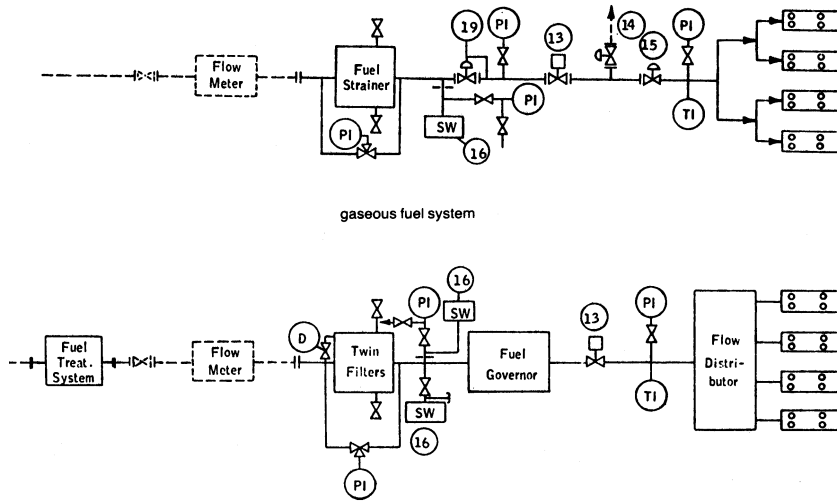
Figure 4-7. Fuel systems for gas turbines.
