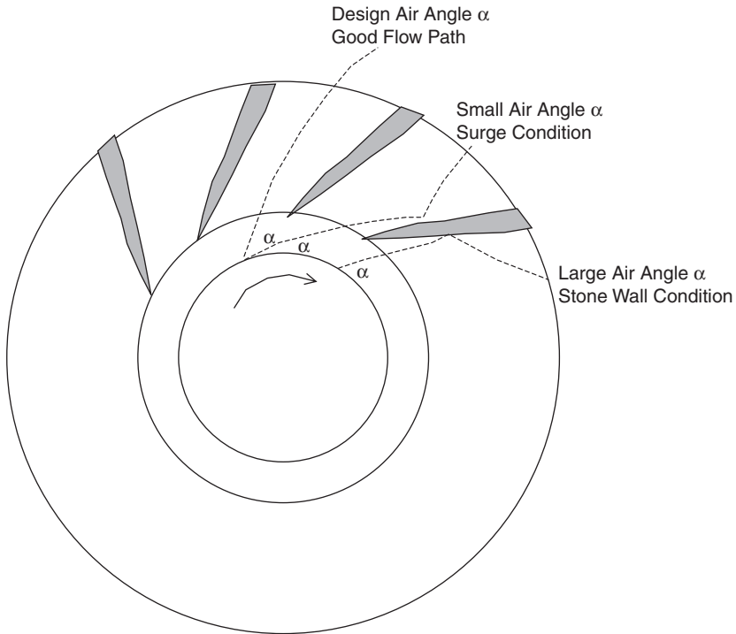
Figure 6-39. Vaned diffuser.
