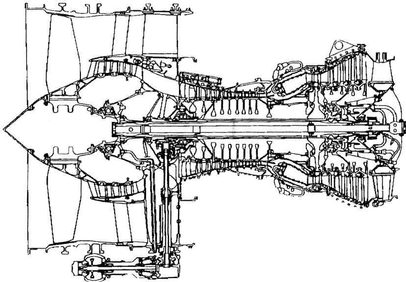
Figure 4-1. A schematic of a fan jet engine with a by-pass fan.
