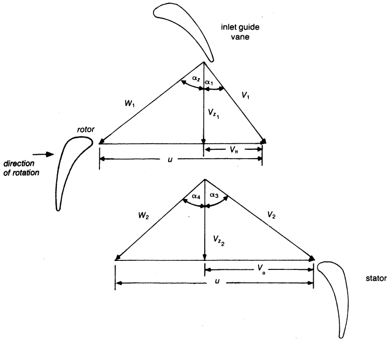
Figure 7-17. Typical velocity triangles for an axial-flow compressor.
