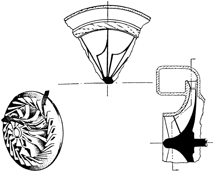
Figure 8-4. Mixed-flow-type radial-inflow turbine.
