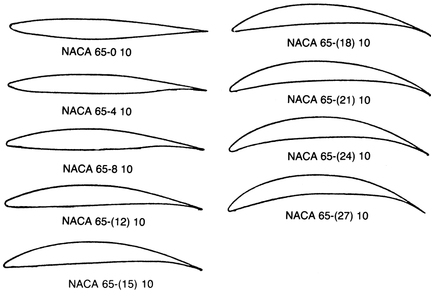
Figure 7-28. The NACA 65 series of cascade airfoils.
