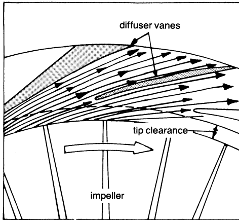
Figure 6-2. Flow entering a vaned diffuser.
