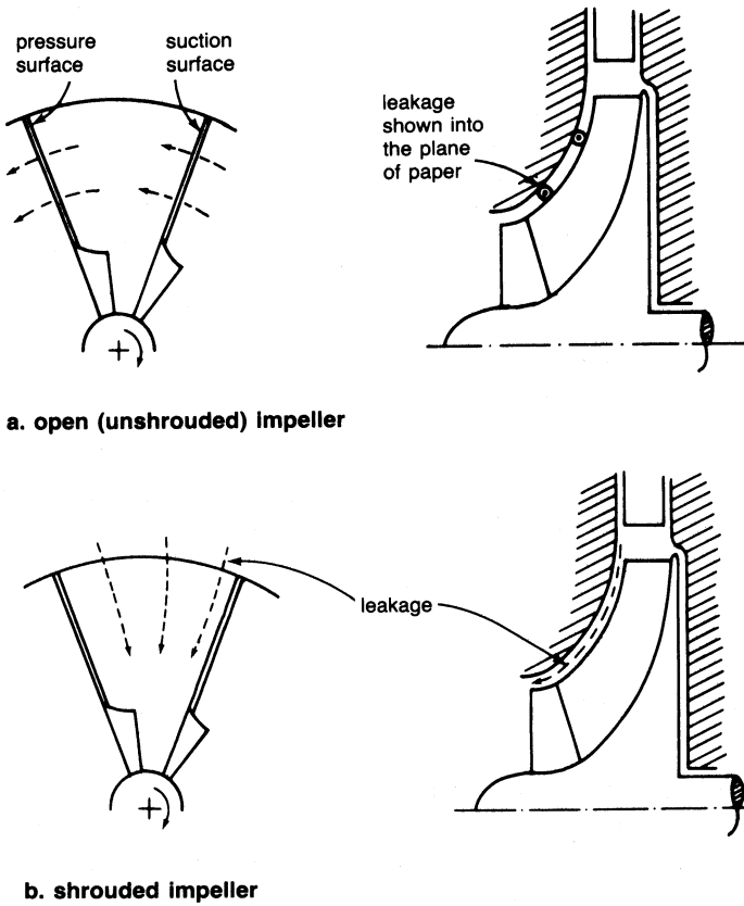
Figure 6-33. Leakage affecting clearance loss.
