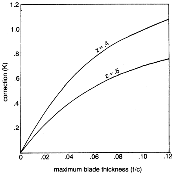
Figure 7-25. Correction factor for blade thickness and incidence angle calculation.
