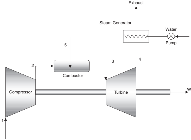
Figure 2-43. Steam injection in the gas turbine combustor.
