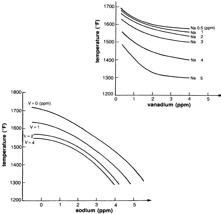
Figure 12-3. The effect of temperature on IN 718 corrosion by sodium and vanadium.
