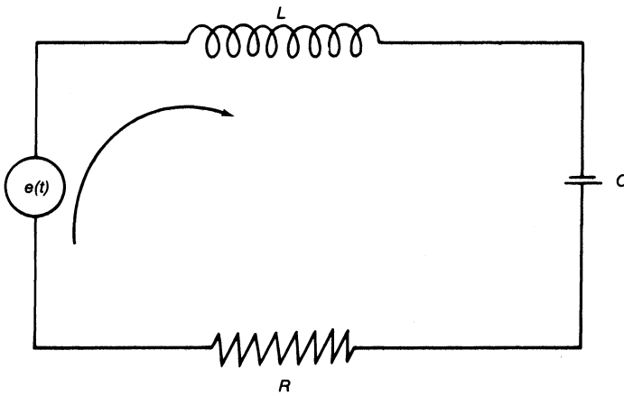
Figure 5-18. A force-voltage system.
