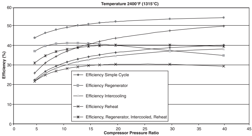
Figure 2-29. Comparison of thermal efficiency of various cycles temperature.
