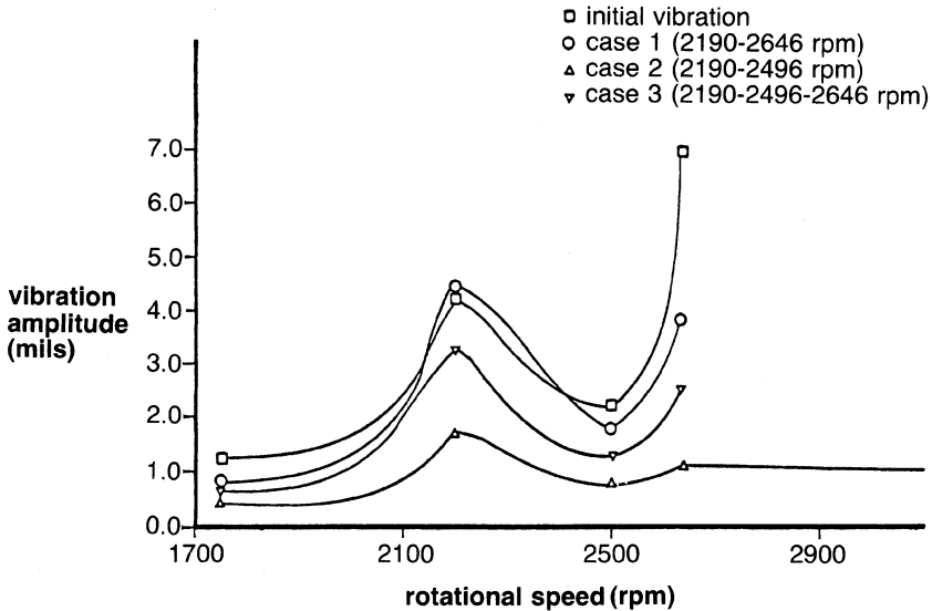
Figure 17-9. Rotor amplitudes for least-square balance.
