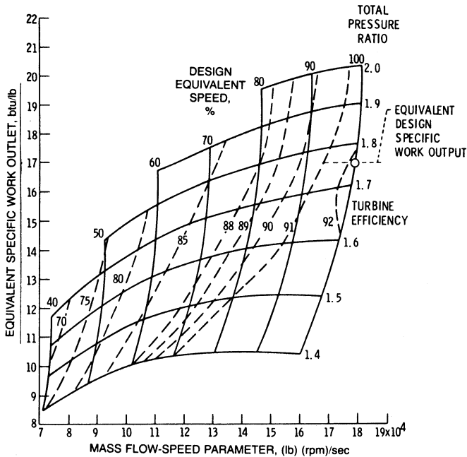
Figure 9-29. Turbine performance map.
