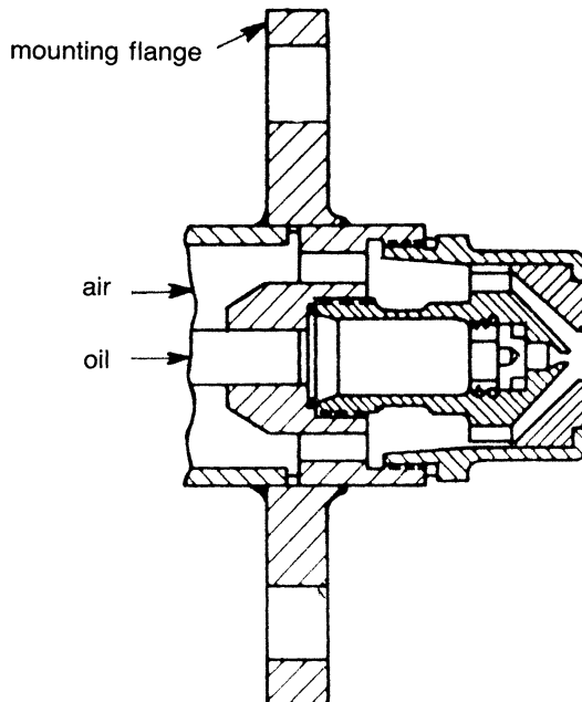
Figure 10-10. Low-pressure air atomizer. (Courtesy of General Electric Company.)
