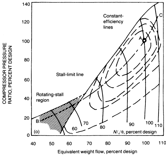
Figure 7-34. Performance map of an axial-flow compressor.
