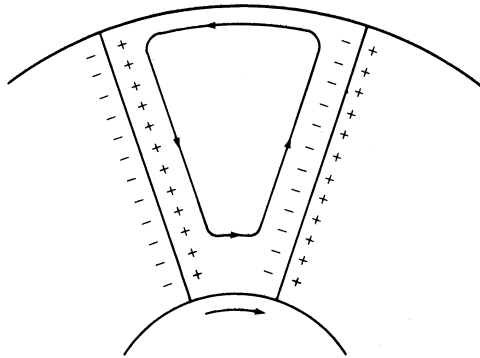
Figure 6-22. Coriolis circulation.
