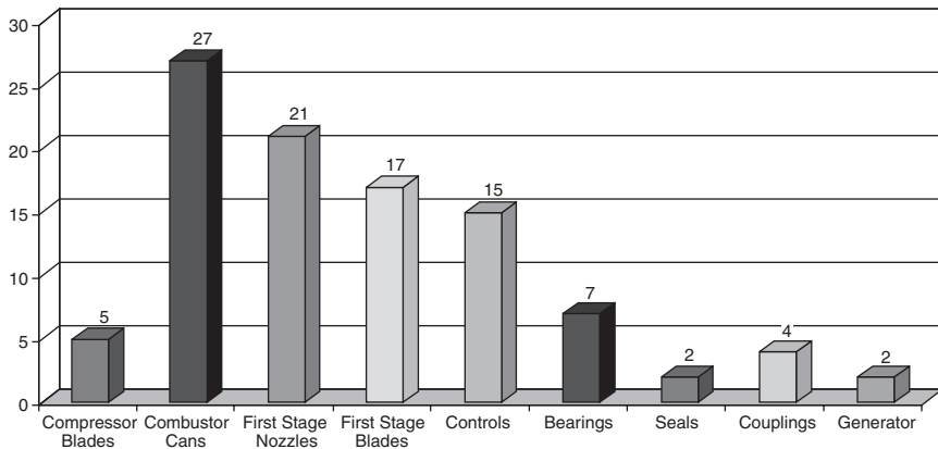
Figure 21-6. Contributions of various major components to gas turbine down time.
