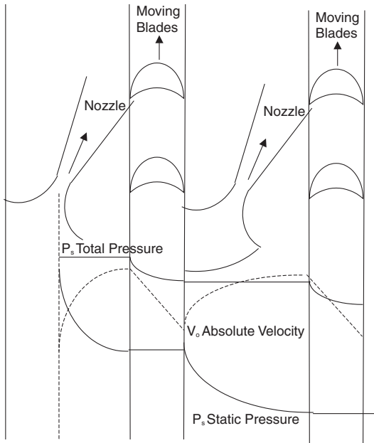
Figure 9-8. Pressure and velocity distributions in a Rateau-type impulse turbine.
