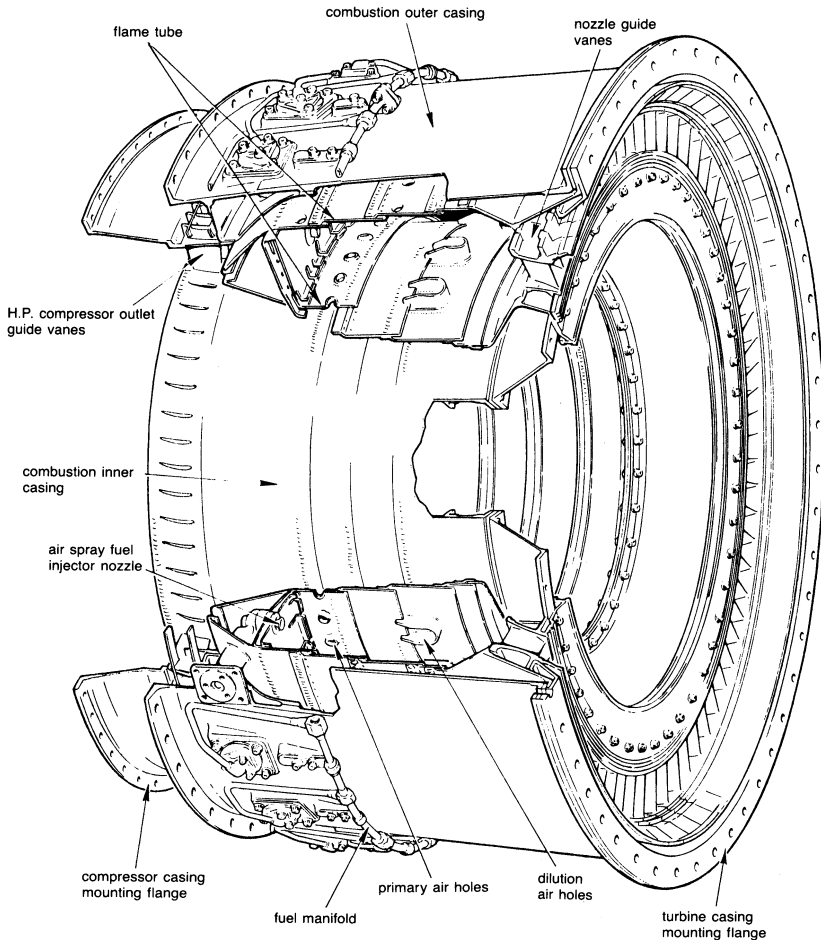
Figure 10-16. Aircraft-type annular combustion chamber. (© Rolls-Royce Limited.)
