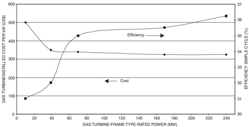
Figure 4-5. Installed cost and efficiency of frame type turbines.
