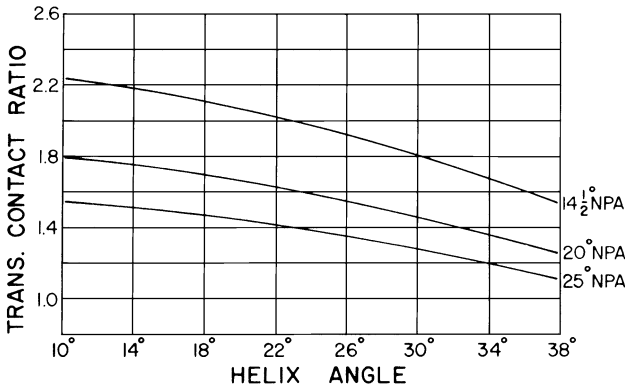
Figure 14-3. Variation of transverse contact ratio with pressure angle and helix angle. (Courtesy of Lufkin Industries, Inc.)
