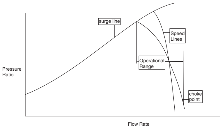
Figure 19-18. Performance map of an axial flow compressor used in most gas turbines.
