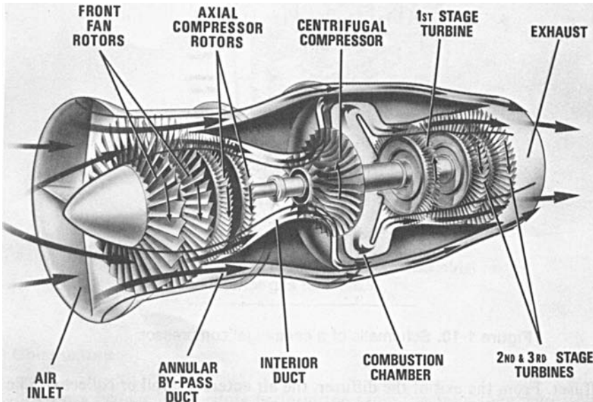
Figure 1-19. A schematic of a cutaway of a small gas turbine used in helicopter or vehicular applications.
