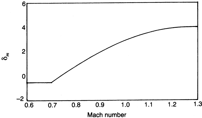
Figure 7-26. Mach-number correction for incidence angle.
