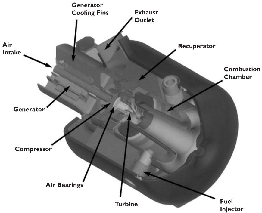
Figure 1-15. A compact micro-turbine schematic. (Courtesy Capstone Corporation.)
