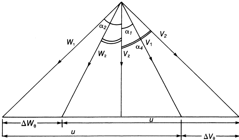
Figure 7-19. Symmetrical velocity triangle for 50% reaction stage.
