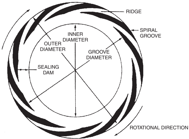
Figure 13-36. Spiral grooved mating ring. (Courtesy Proceedings Seventeenth Turbomachinery Symposium, Dry Gas Compressor Seals by Piyush Shah, John Crane Inc.)
