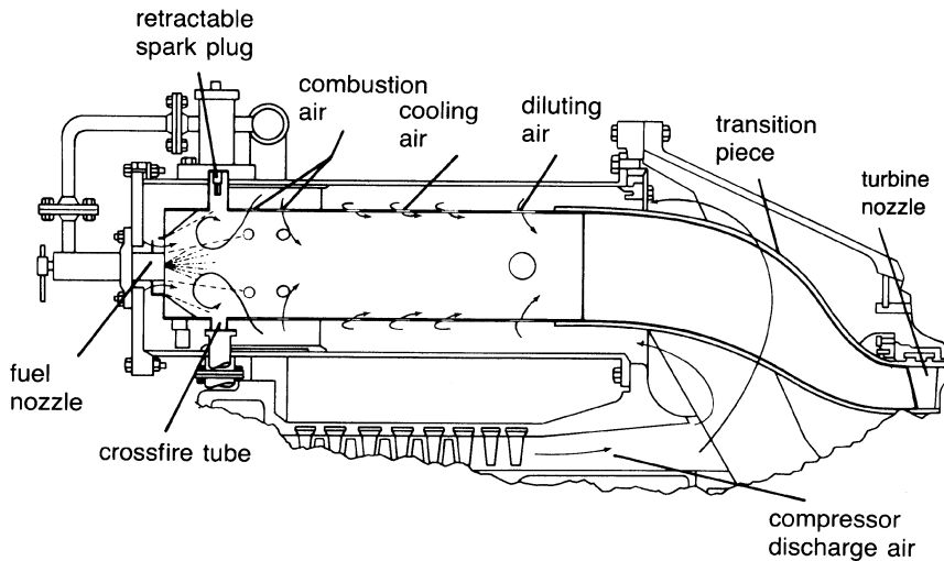
Figure 10-14. Turbo-annular or can-annular combustor for a heavy-duty gas turbine. (Courtesy of General Electric Company.)
