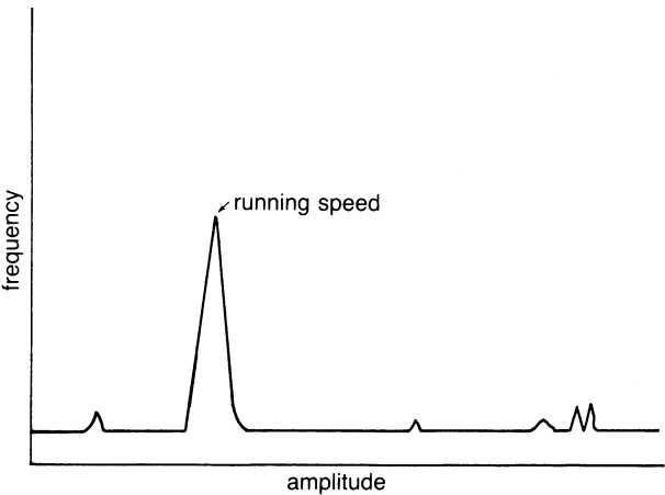
Figure 16-9. A typical unbalance signature plot.
