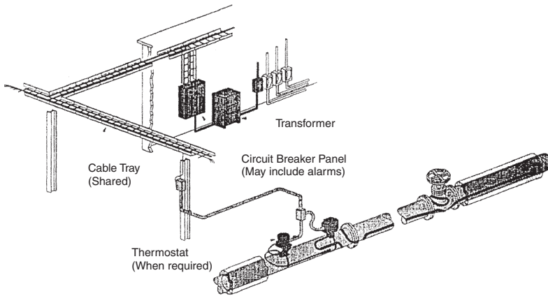
Figure 12-13. Electric heat tracing system.
