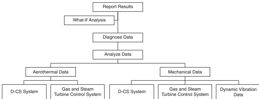
Figure 21-1. Total performance-based condition monitoring system.
