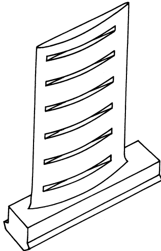
Figure 7-9. Perspective of compressor blade with treatment.
