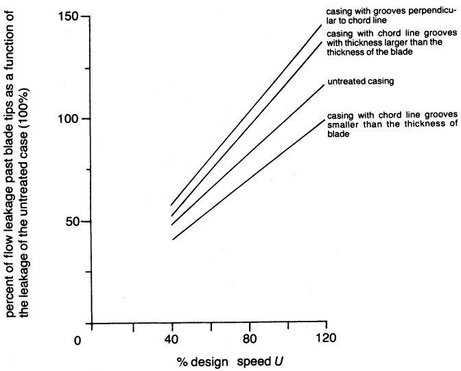
Figure 7-15. Mass flow leakage at tips for various casing treatments.
