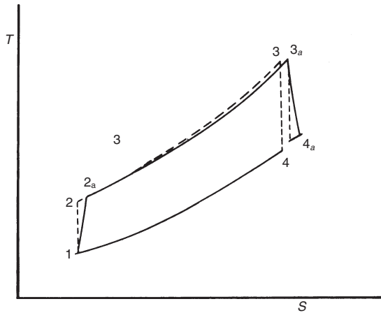
Figure 2-9. T-S diagram of the actual open simple cycle.
