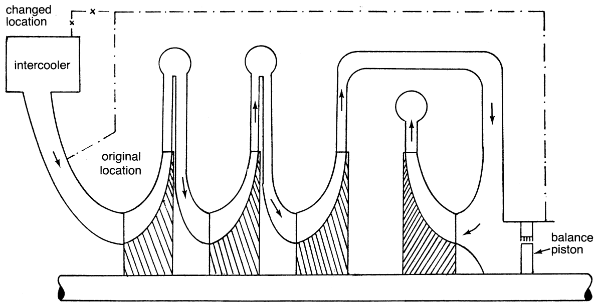
Figure 21-23. Thrust forces in a centrifugal compressor.
