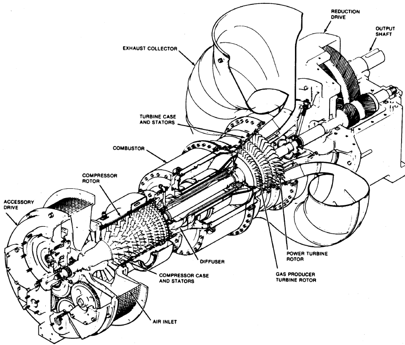
Figure 1-11. A medium size industrial gas turbine. (Courtesy Solar Turbines Incorporated.)
