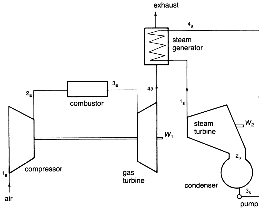
Figure 2-26. The Brayton-Rankine combined cycle.
