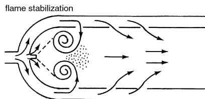
Figure 10-8. Flow pattern by swirl vanes and radial jets.
