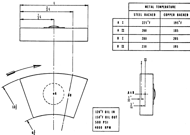
Figure 21-10. Temperature distribution in bearing surfaces.
