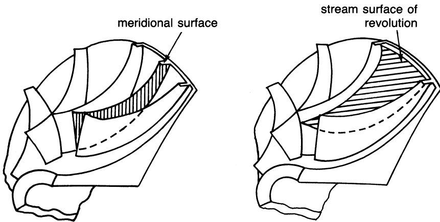
Figure 6-15. Two-dimensional surface for a flow analysis.
