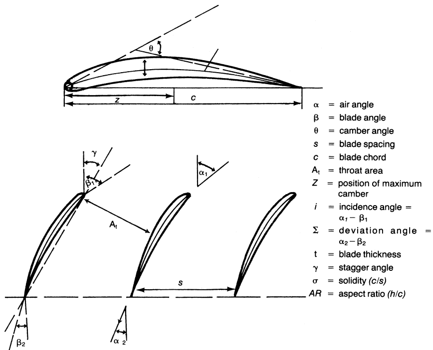
Figure 7-4. Blade profile nomenclature.
