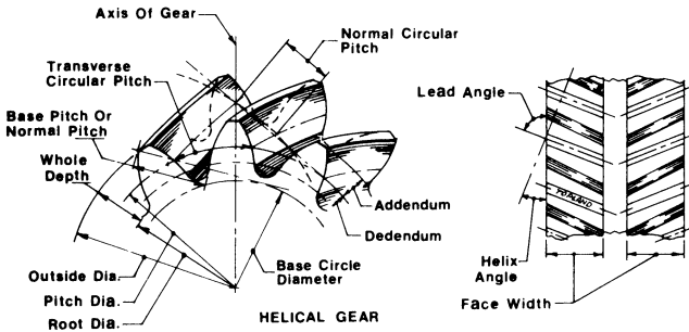
Figure 14-2. Helical gear terminology.
