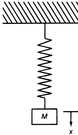
Figure 5-1. System with single degree of freedom.
