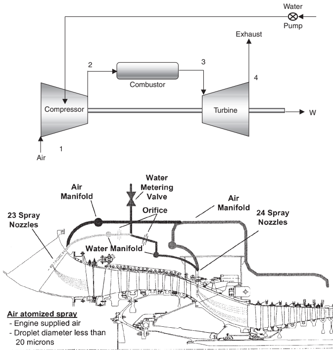
Figure 2-40. Mid-compressor cooling showing a schematic as well as an actual application in a GE LM 6000 Engine. (Courtesy GE Power Systems.)
