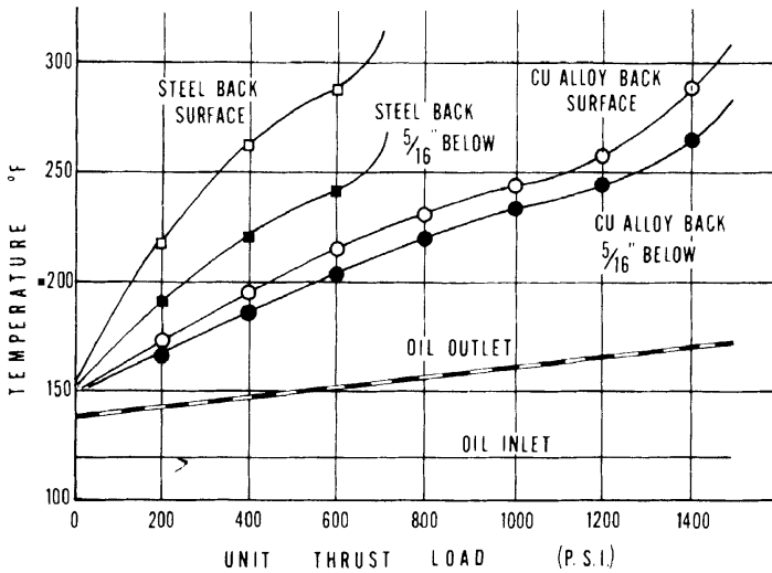
Figure 13-19. Thrust-bearing temperature characteristics.
