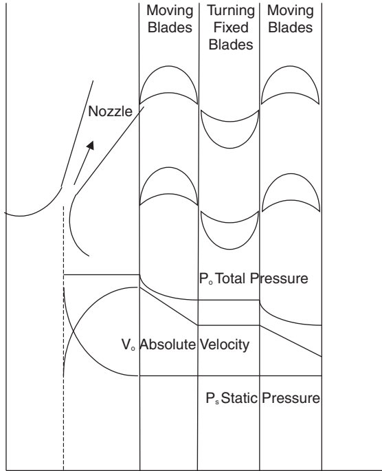
Figure 9-7. Pressure and velocity distributions in a Curtis-type impulse turbine.
