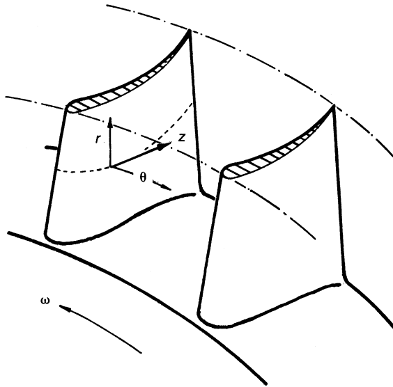
Figure 7-2. Coordinate system for axial-flow compressor.
