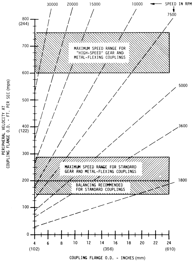
Figure 18-1. Flexible coupling operating spectrum.
