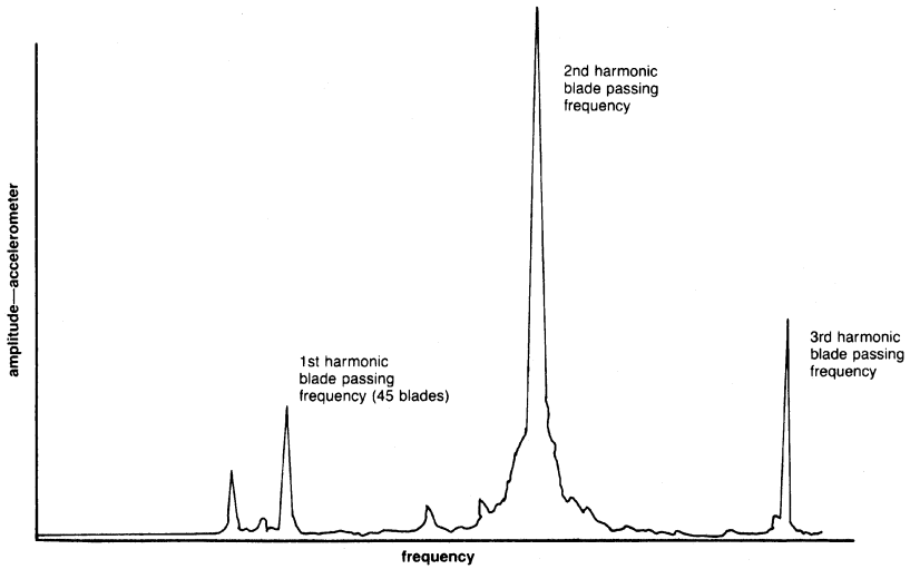
Figure 16-14. Axial-flow compressor spectrum showing blade passing frequency.
