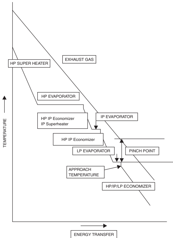
Figure 2-33. Energy/temperature diagram of the triple pressure HRSG.
