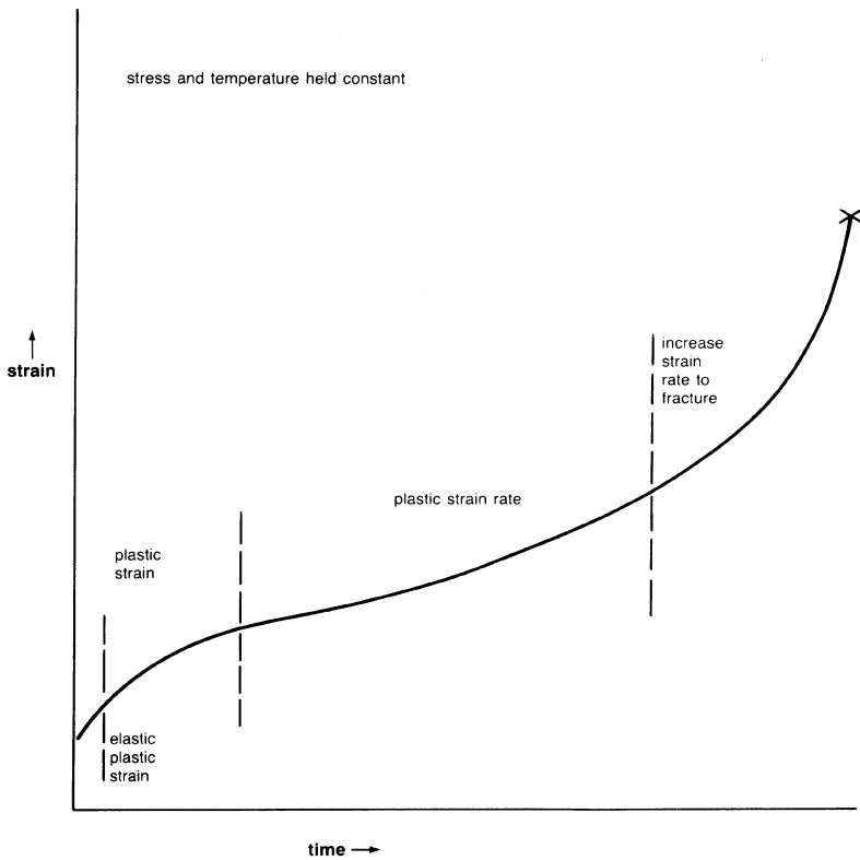
Figure 11-3. Time dependent strain curve under constant load.
