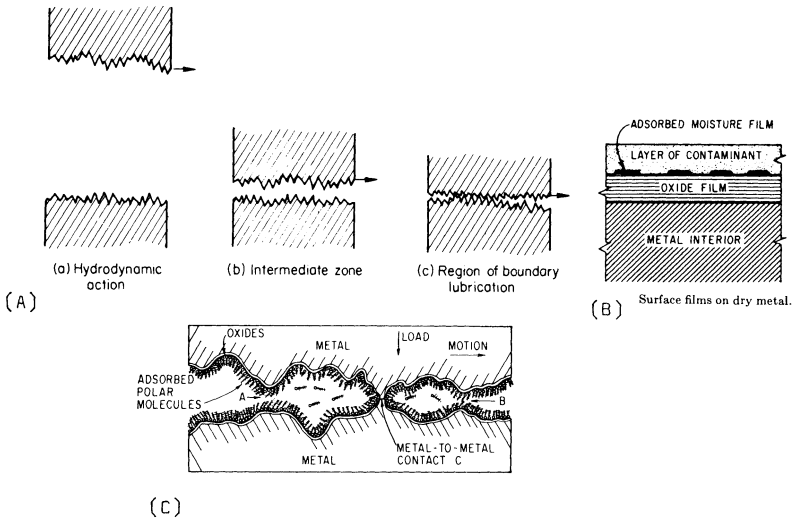
Figure 13-9. Enlarged views of bearing surfaces.
