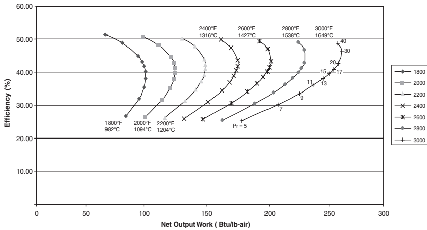
Figure 2-22. The performance map of a steam injected gas turbine.
