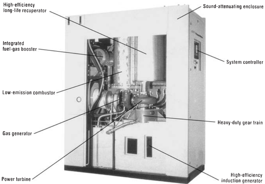
Figure 1-16. A cogeneration micro-turbine system package. (Courtesy Ingersoll Rand Corporation.)
