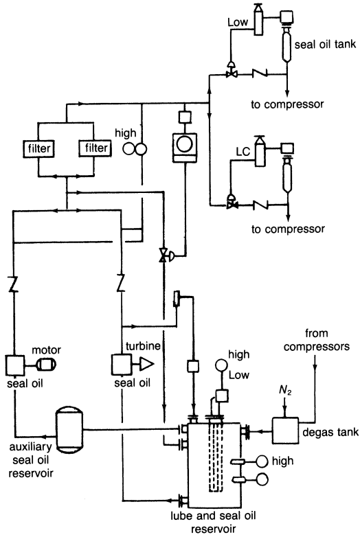
Figure 15-4. Seal oil system.
