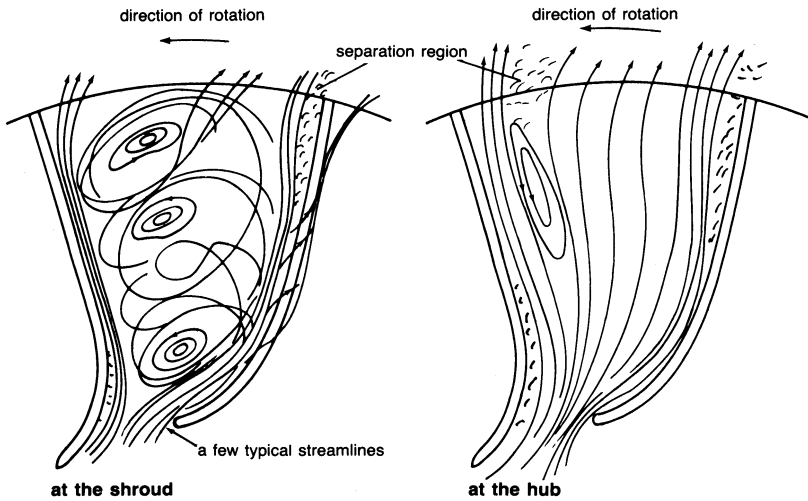
Figure 6-16. Flow map of impeller plane.
