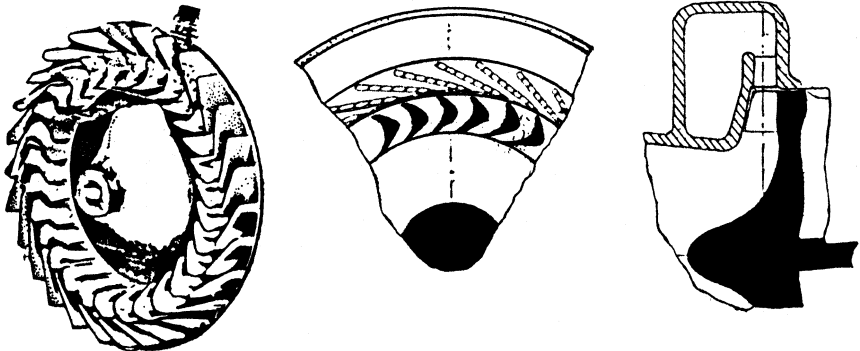
Figure 1-34. Cantilever-type radial inflow turbine.
