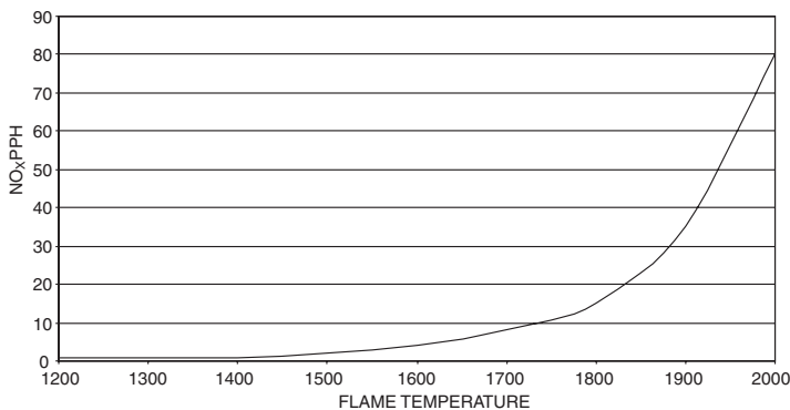
Figure 10-21. Correlation of adiabatic flame temperature with \text{NO}_x emissions.
