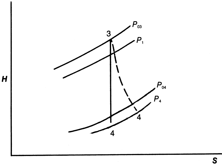
Figure 3-5. Entropy-enthalpy diagram of a turbine.
