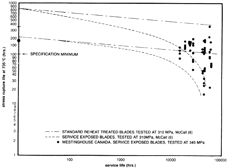
Figure 21-12. The variation of remaining stress rupture life at 1350°F (735°C) with service time in forged Inconel alloy X-750 turbine blades. (Courtesy of Westinghouse Electric Corp., Gas Turbine Div.).
