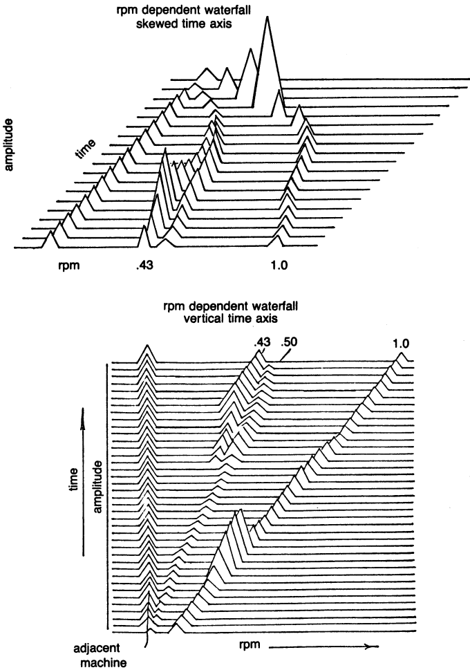
Figure 16-4b. Waterfall graph of increasing rpm.
