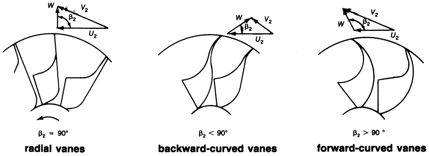
Figure 6-8. Various types of impeller blading.
