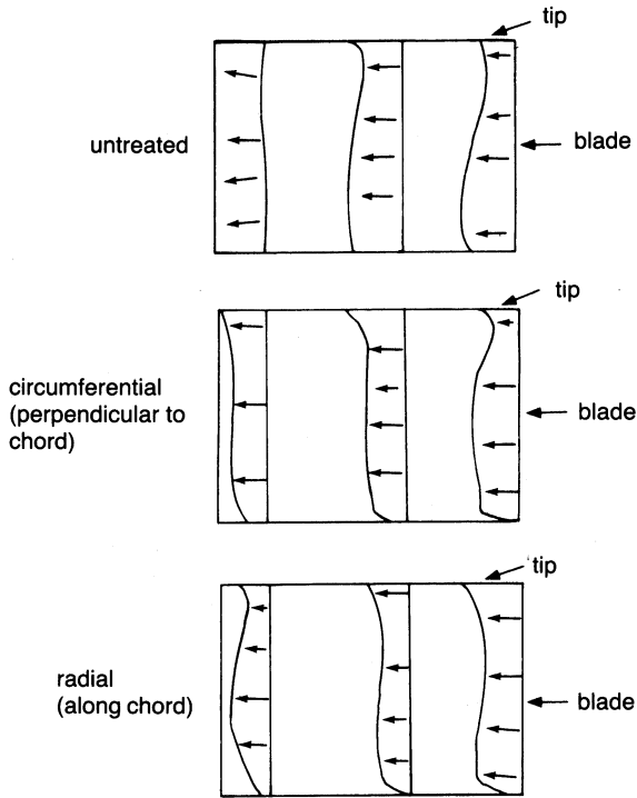
Figure 7-16. Velocity patterns observed in the side view of the blade passage for various casing treatments.
