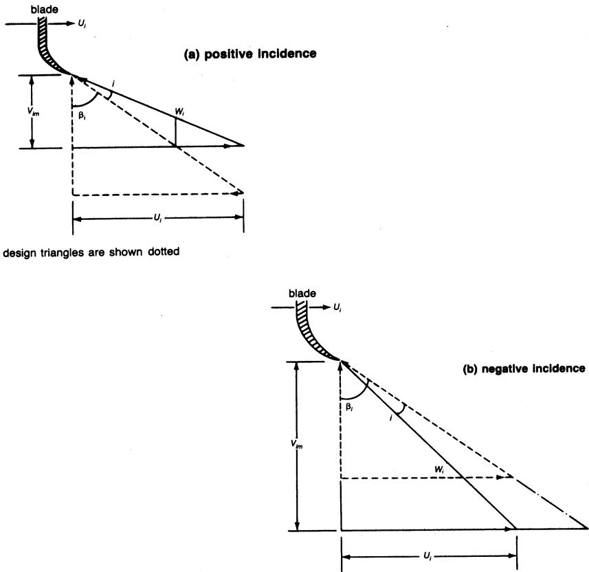
Figure 6-31. Inlet velocity triangles at nonzero incidents.
