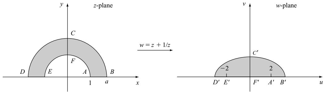
Figure 30.6. The mapping w = z + 1/z .
