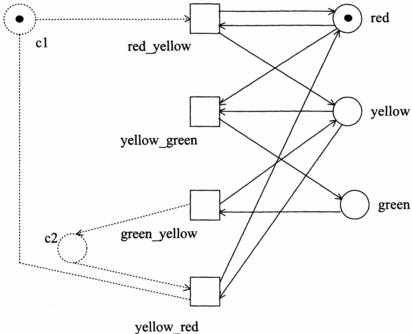
Figure S2.2 German traffic light model
