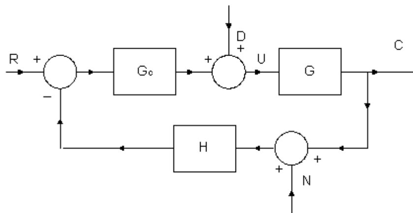
Figure 5.1 Basic Block Diagram of Feedback Control System.
