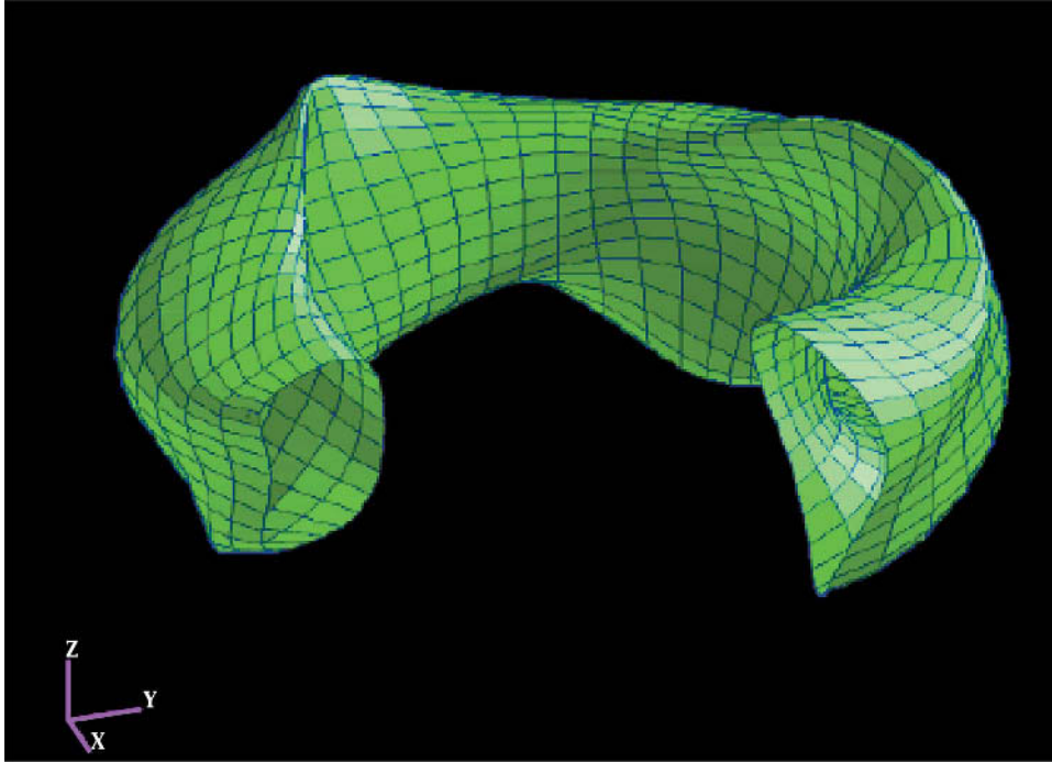
FIGURE 2.1 Pressure surface of a three-dimensional stellarator equilibrium illustrates the complex equilibria that can be studied and manipulated to maximize confinement and other properties. Courtesy of M. Zarnstorff, Princeton Plasma Physics Laboratory (PPPL).
