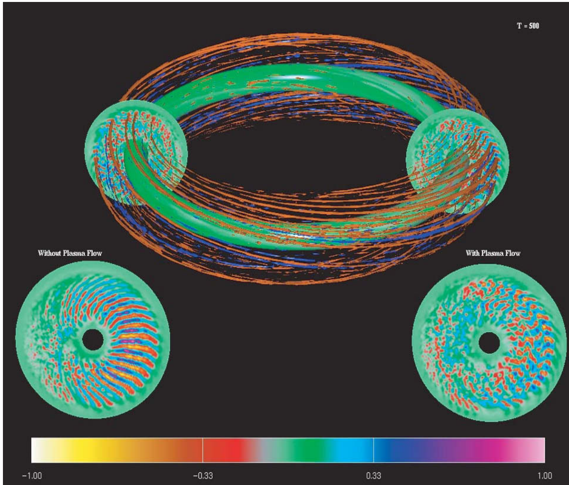
FIGURE 2.5 Simulation of ion energy transport in a tokamak plasma. Surfaces show the vortices that develop both with and without large-scale poloidal rotation, which acts to break up the flow patterns, reducing transport in magnetic confinement systems. Courtesy of W.M. Tang (PPPL). A similar image first appeared in Science , 1998, vol. 281, pp. 1835-1837.
