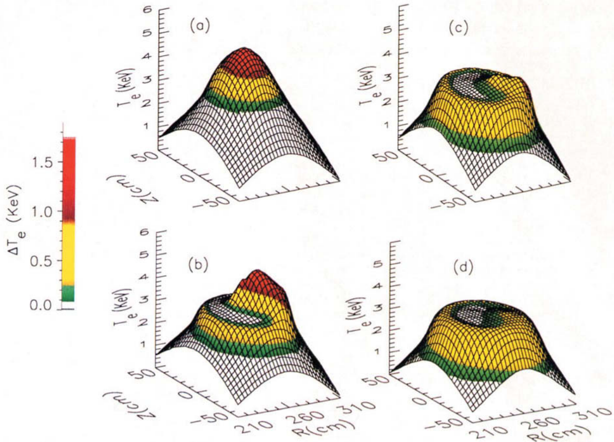
FIGURE 2.4 Measurements of the electron temperature at the core of the TFTR tokamak during a sawtooth crash. The measurements are taken with a high-resolution grating polychrometer, which measures the cyclotron emission from electrons as they spiral around the magnetic field lines. Courtesy of M. Yamada (PPPL). Reprinted by permission from Physics of Plasmas , 1994, vol. 1, pp. 3269-3276.
