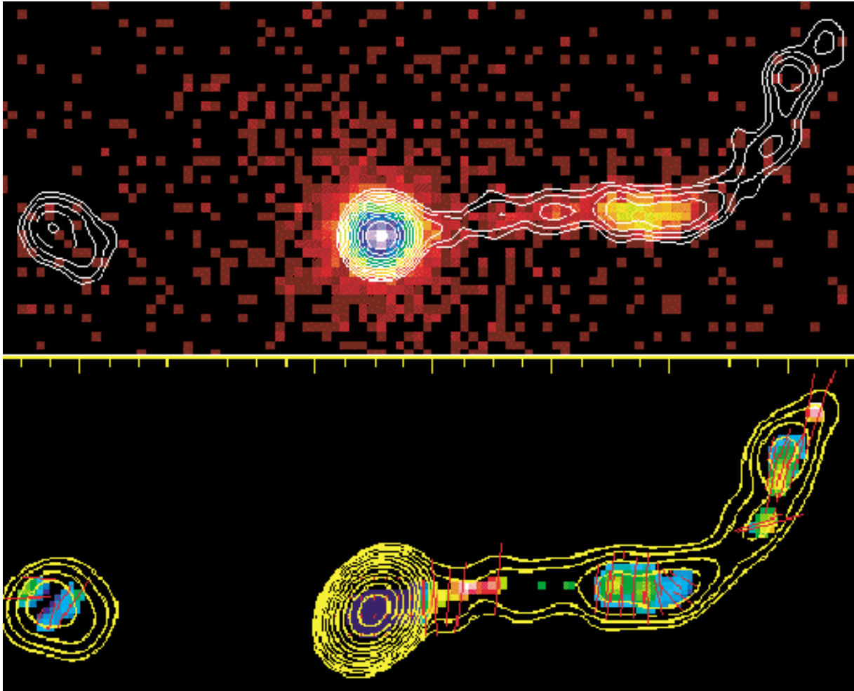
FIGURE 4.2 A Chandra X-ray Observatory (ACIS-S) image (top) of x rays from the quasar PKS 0637-752. The contours show an overlay of the 8.6-GHz emission measured with the ATCA. One tic mark is 1 arcsec, which corresponds to 9.2 kpc in the plane of the sky for the redshift 0.652 of this object. The x-ray jet, which closely correlates with the radio emission from 4 to 10 arcsec west of the nucleus, is the largest and most luminous detected to date. The radio polarization fraction and E-vector direction are shown in the bottom panel. Clearly, major events are taking place 11 arcsec west of the quasar, where the radio jets bend, the x-ray emission drops, and the radio emission becomes unpolarized, followed by realignment of the magnetic field direction. Courtesy of NASA, SAO, D. Schwartz (SAO), and the PKS 0637-752 Consortium.
