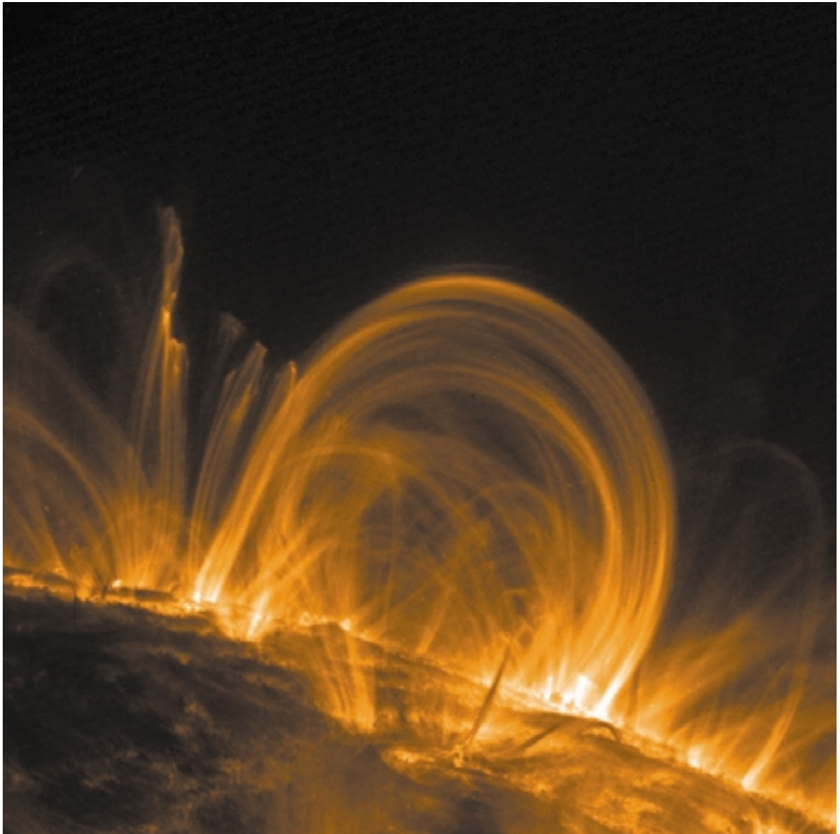
FIGURE 4.3 This solar image was taken with the TRACE telescope, using a normal incidence soft x-ray mirror whose band pass is centered on an emission line of Fe IX; the image clearly shows the highly complex structuring caused by solar surface magnetic fields and the remarkable “plasma loops,” which indicate million-degree solar gases trapped by these magnetic fields. Courtesy of NASA and the Stanford-Lockheed Institute for Space Research.
