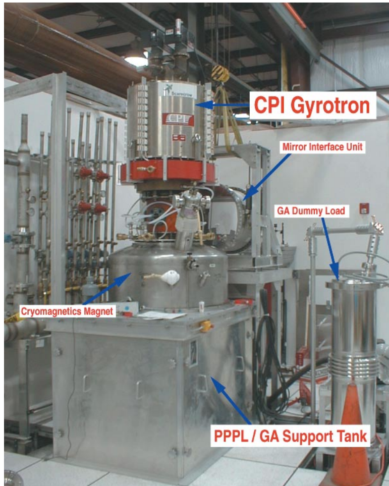
FIGURE 2.2 A gyrotron from the DIII-D tokamak experiment at General Atomics (GA) in San Diego. A gyrotron is a source of high-frequency radio waves for heating electrons. Courtesy of General Atomics.
