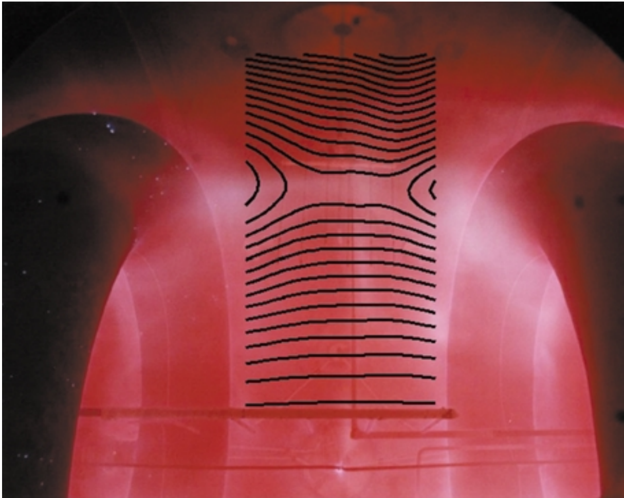
FIGURE 4.4 This image shows the interior of the MRX reconnection experiment. The pair of large coils produce oppositely directed magnetic field lines. The bright area between the coils (in an X-shaped pattern) is the region where magnetic energy is being released into the plasma through the reconnection process. Superimposed is a snapshot of the measured magnetic field. Courtesy of M. Yamada (PPPL). Reprinted by permission from Journal of Geophysical Research , 1999, vol. 104, p. 14529.
