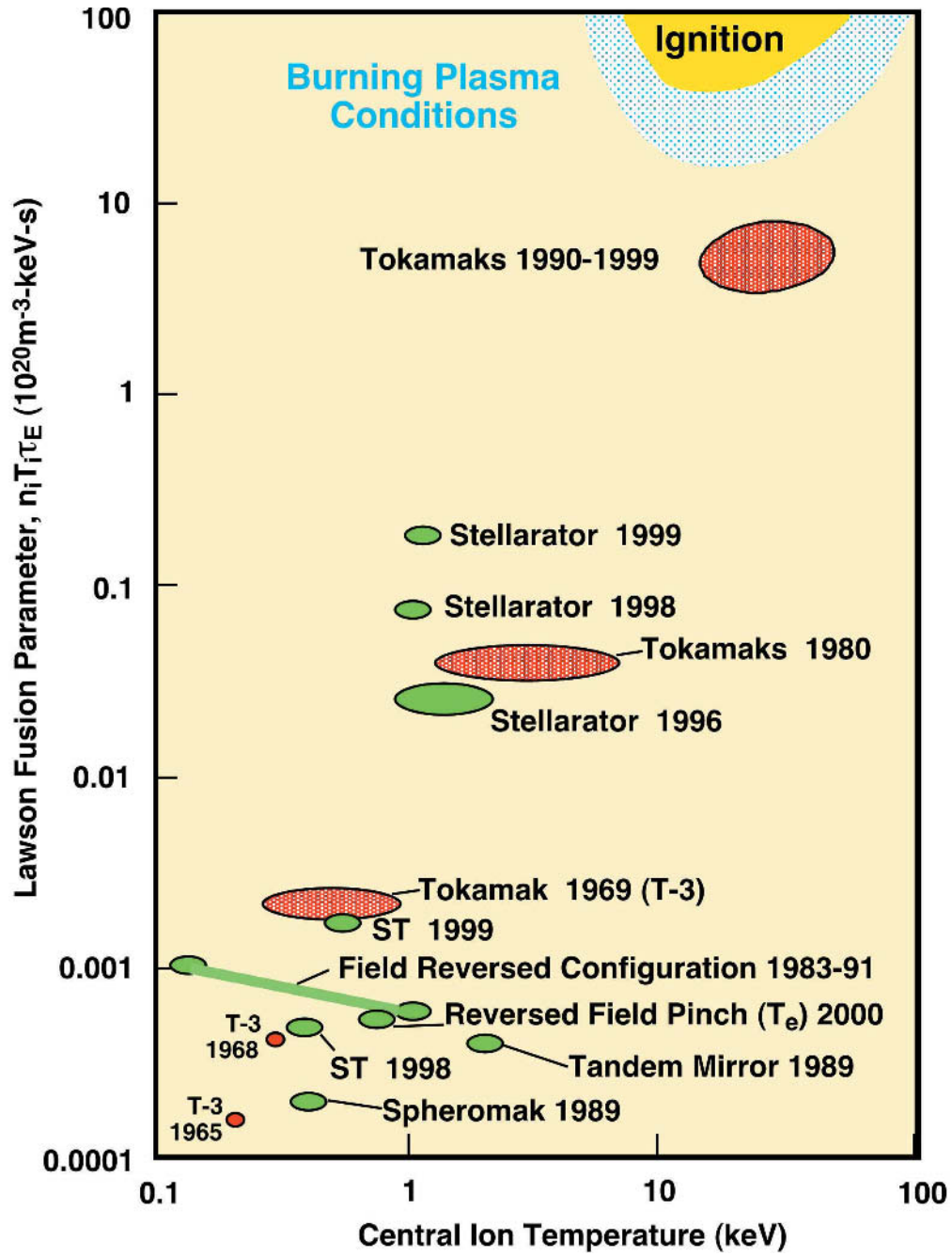
FIGURE 3.5 Improvements in plasma stability and confinement obtained in magnetic confinement configurations should allow the study of burning fusion plasmas in the near future. The Lawson fusion parameter is the product of the plasma density, ion temperature, and average confinement time and represents a simple figure of merit for proximity to conditions for fusion ignition. Courtesy of PPPL.
