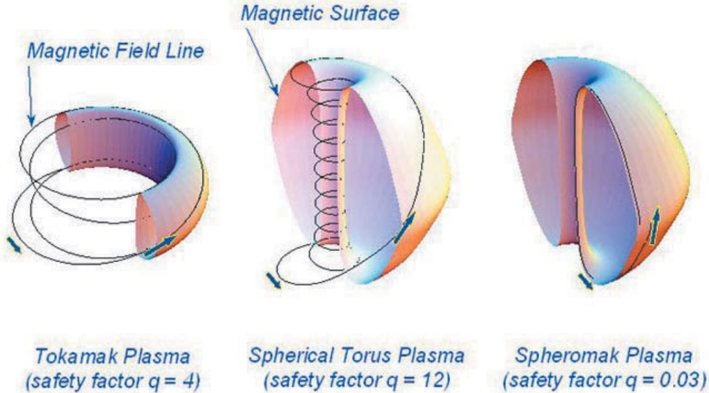
FIGURE 3.2 Examples of the magnetic topologies of several related toroidal configurations with increasing curvature and varying stability characteristics. The tokamak (left) uses a strong external toroidal field to provide robust stability against pressure- and current-driven instabilities. The spherical torus uses a weak toroidal field in a compact configuration to allow access to higher \beta values than obtained in the tokamak. The spheromak (right) uses internal plasma currents only to provide the confining poloidal field plus a weak toroidal field. A larger safety factor indicates a higher level of protection from current-driven instabilities. Courtesy of M. Peng (PPPL). Reprinted by permission from Physics of Plasmas , 2000, vol. 7, pp. 1681-1692.
