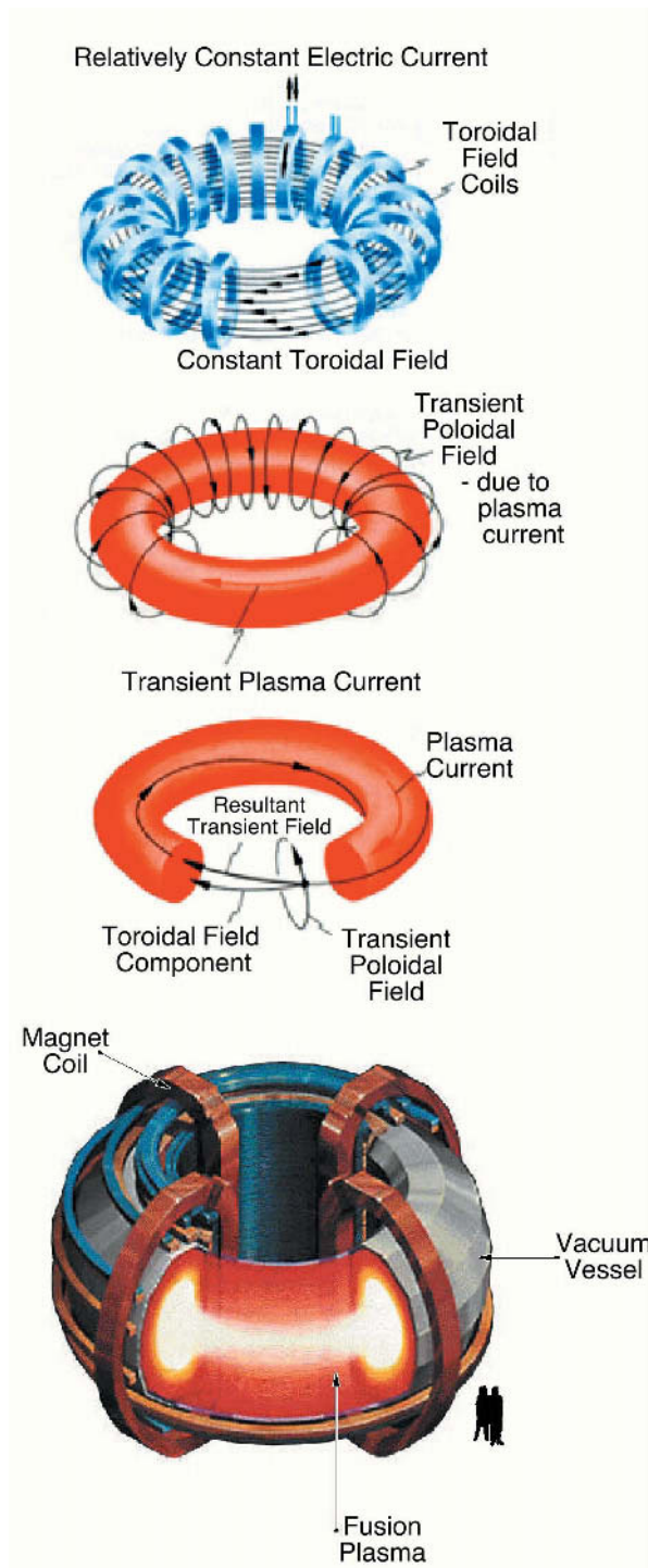
FIGURE 3.1 Components of the tokamak confinement configuration, one of the more advanced plasma confinement concepts. It uses a strong toroidal field created by external field coils (top) to stabilize the plasma while using a poloidal field created by a toroidal plasma current to confine the particles. The final configuration includes a large vacuum vessel to isolate the hot plasma from the surrounding environment (bottom). Courtesy of General Atomics and PPPL.
