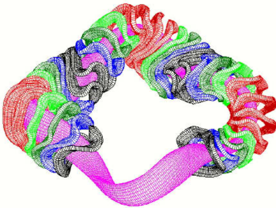
(c) Quasi-Symmetric Stellarator
