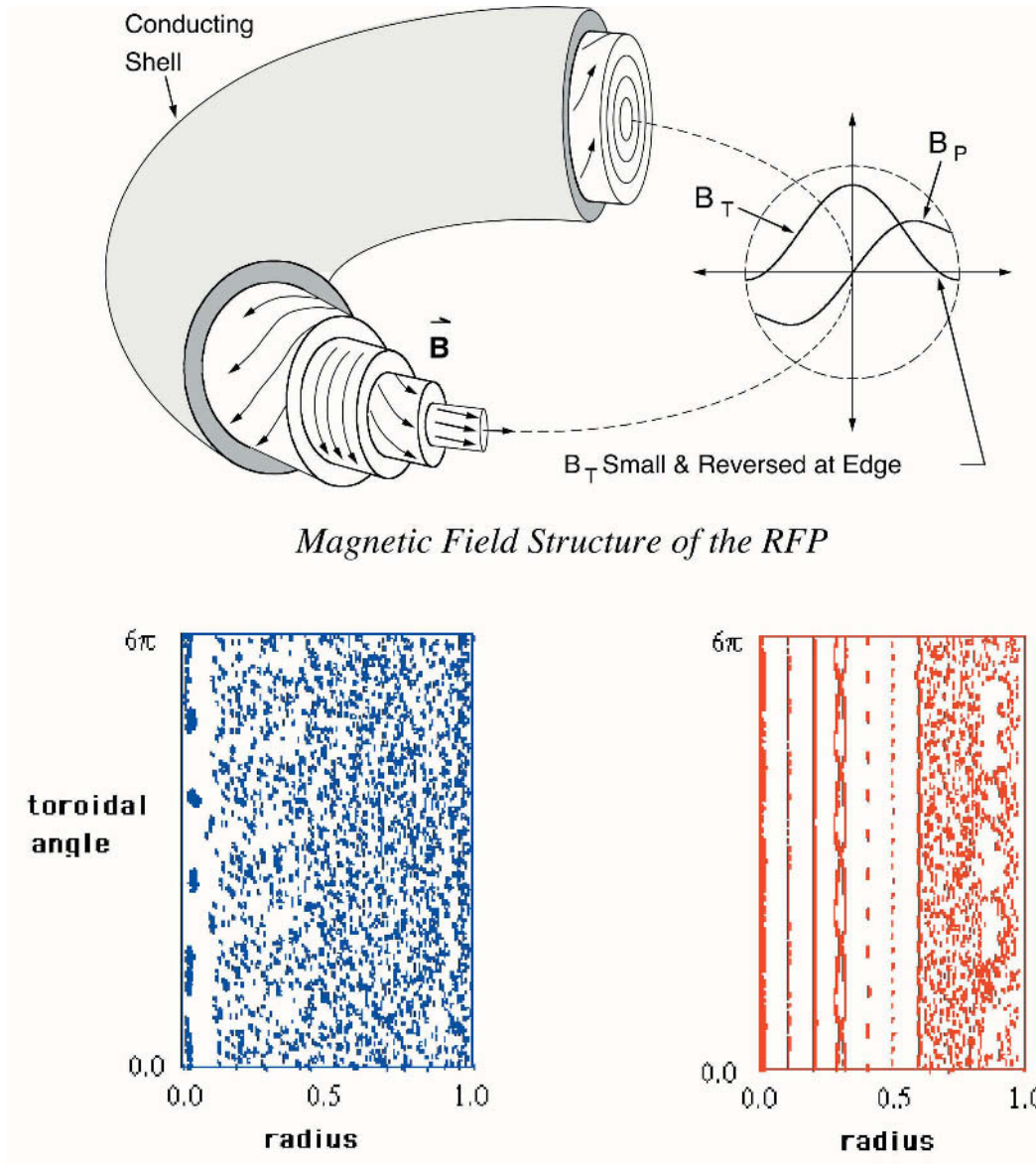
FIGURE 3.3 A magnetic confinement concept such as the reversed-field pinch (top) is a relatively self-organizing configuration that is subject to turbulent magnetic field structures. The magnetic topology includes a reversal of the toroidal field inside the plasma owing to plasma currents. Under normal inductive current drive, the magnetic field lines can readily become chaotic, as indicated by a puncture plot of the field lines as they traverse a poloidal plane (bottom left). With finer control of the plasma currents, well-defined flux surfaces are restored (bottom right). Courtesy of S. Prager (University of Wisconsin at Madison).
