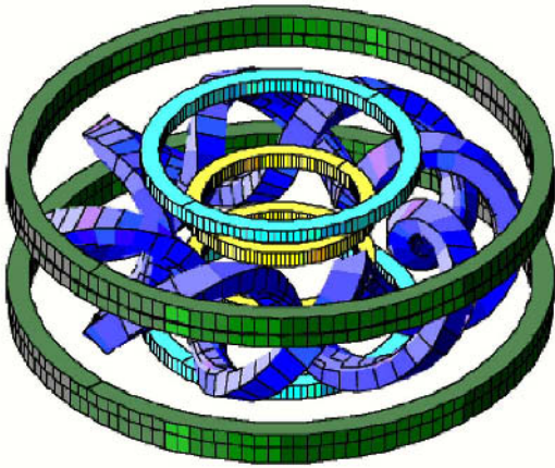
(a) Conventional Stellarator
