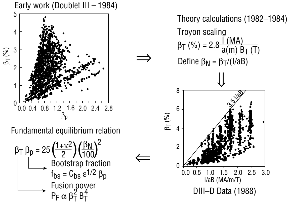
FIGURE 2.3 Pressure limits as measured by the plasma \beta (ratio of plasma to magnetic pressure) in the DIII-D tokamak. The convergence of the data when normalized to the theoretically based pressure limit was one of the early successes of the theory program. Courtesy of General Atomics.
