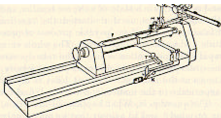
FIG. 22.—Bowditch's Reaction-timer. F , tuning-fork carrying a little plate which holds the paper on which the electric pen M makes the tracing, and sliding in grooves on the base-board. P , a plug which spreads the prongs of the fork apart when it is pushed forward to its extreme limit, and releases them when it is drawn back to a certain point. The fork then vibrates, and the pen, at T is a tongue fixed to the carriage of the fork, and at K an electric key which the tongue opens and with which the electric pen is connected. At the instant of opening, the pen changes its place and the undulating line is drawn at a different level on the paper. The opening can be made to serve as a signal to the reactor in a variety of ways, and his reaction can be made to close the pen again, when the line returns to its first level. The reaction time = the number of undulations traced at the second level.
