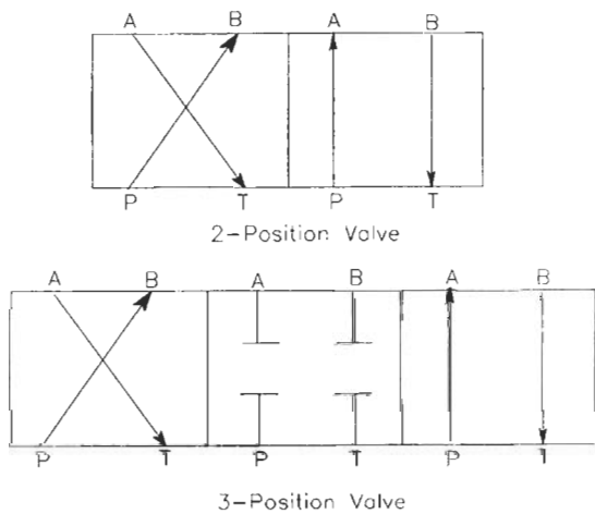
Figure 17-14 Schematic of two-position and three-position valves.
