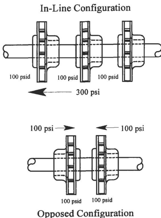
Figure 7-1 Impeller orientation of multistage centrifugal pumps.
