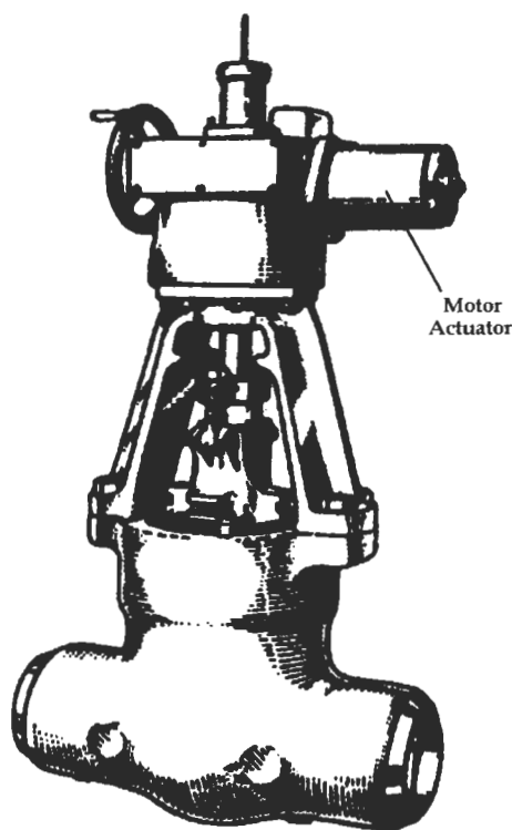
Figure 17-8 High-torque electric motors can be used as actuators (Higgins and Mobley 1995).
