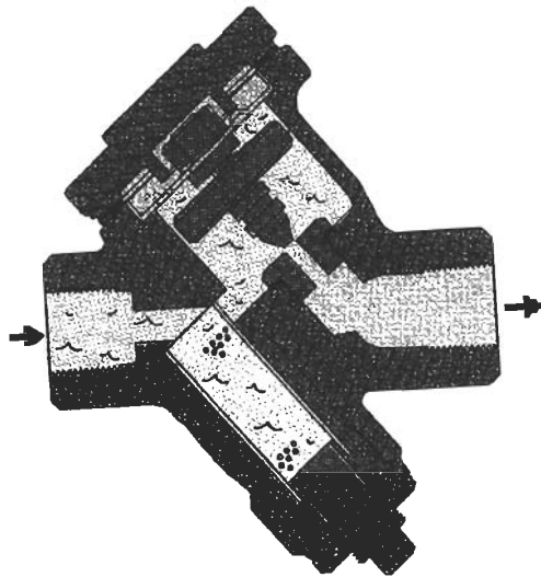
Figure 15-5 Thermostatic trap.
