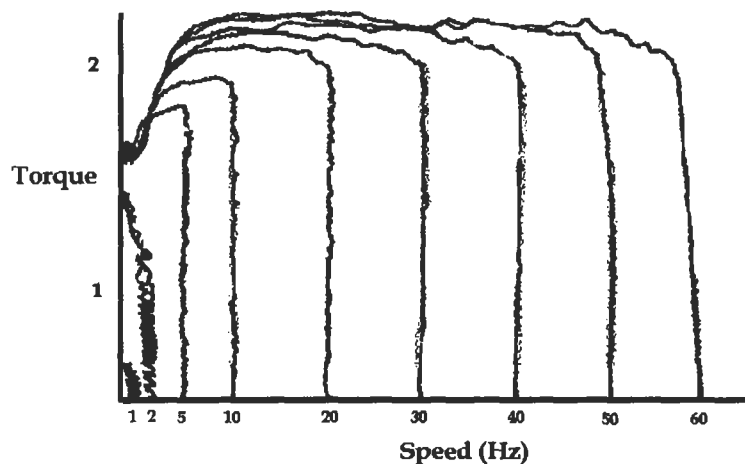
Figure 16-4 Flux vector has limited ability to supply full torque at low speeds.
