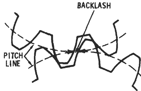
Figure 14-17 Backlash (Neale 1993).
