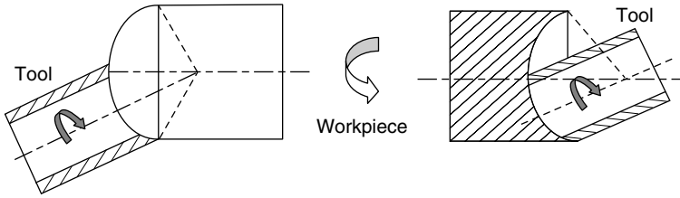
Figure 5.18 Rotary EDM.
