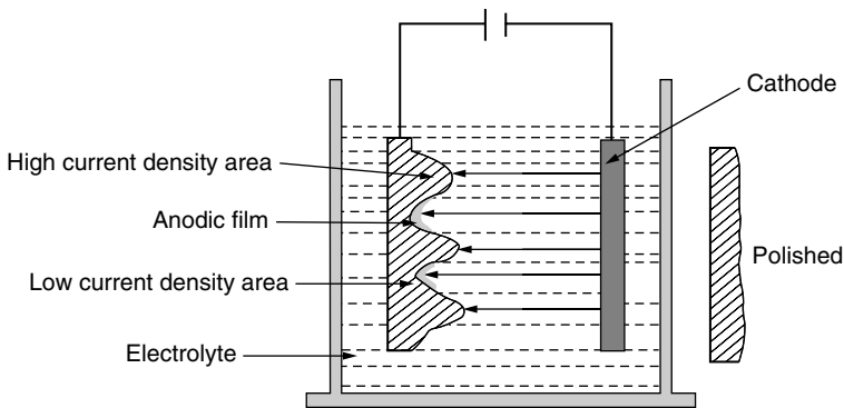
Figure 3.16 Electropolishing process.
