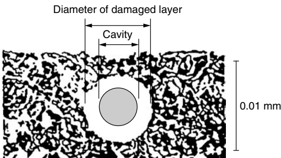
Figure 5.47 Cross section of cavity by single EBM pulse in chromium molybdenum steel (Kaczmarek, 1976).
