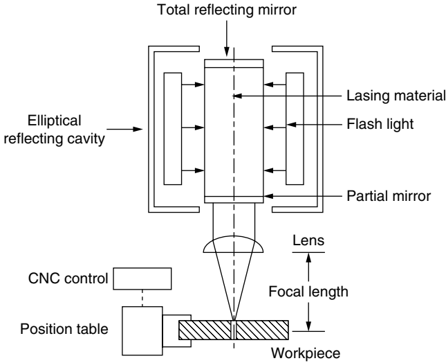
Figure 5.32 LBM schematic.
