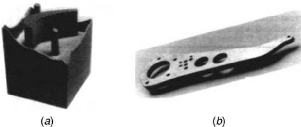
Figure 2.14 (a) Silicon nitride turbine blades (sinking), and (b) CFC acceleration lever and holes (contour USM) (Benkirane et al., 1995).
