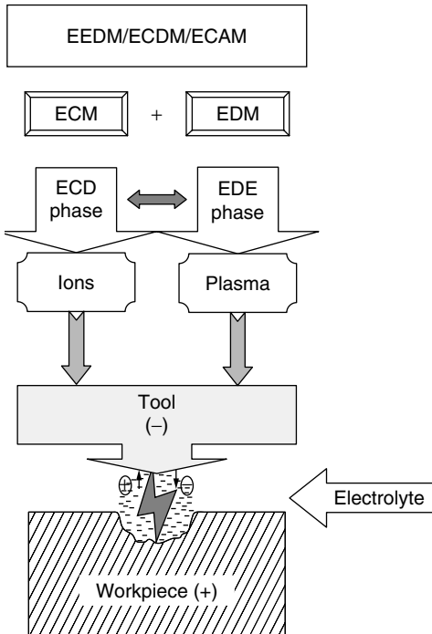
Figure 7.6 EEDM process components.
