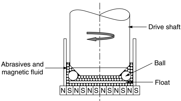
Figure 2.31 Magnetic finishing of balls (Kalpakjian, 1997).
