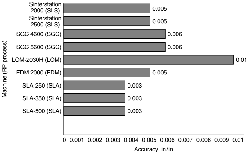
Figure 8.14 Accuracy levels for RP techniques (Wright, 2001).
