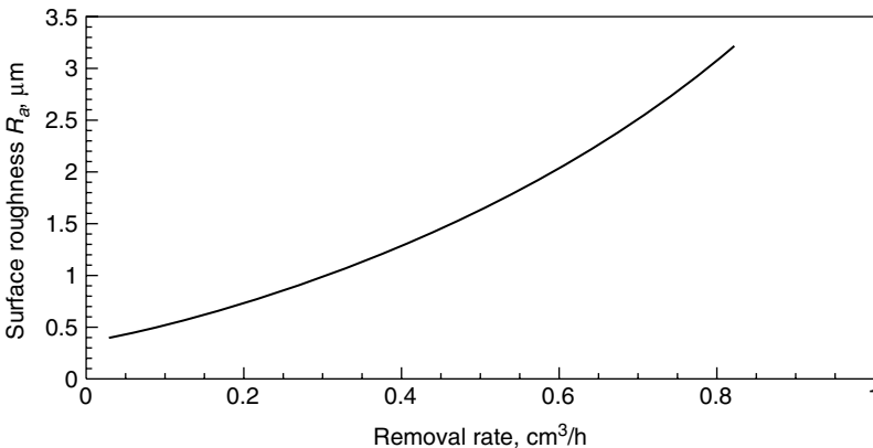
Figure 7.13 Removal rate and surface roughness in EDM (El-Hofy, 1995).
