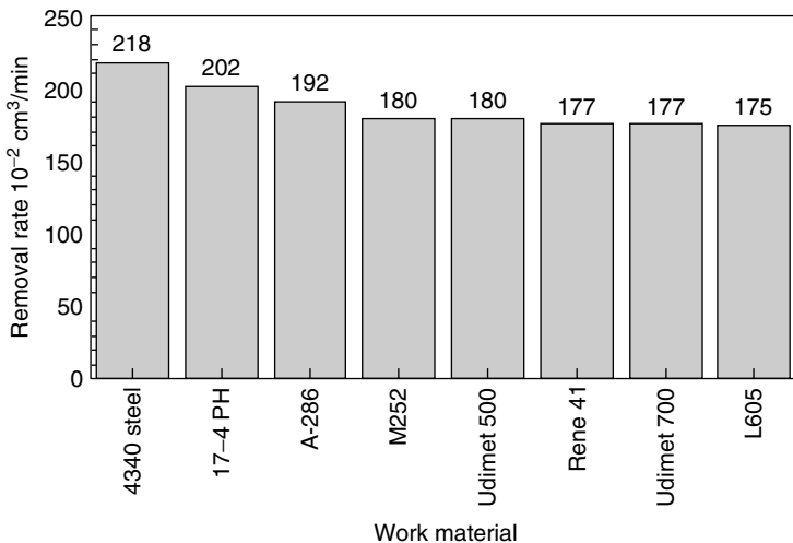
Figure 4.10 Theoretical removal rates for ECM of alloys assuming 100 percent current efficiency and a current density of 1.53 \text{ A/mm}^2 (El-Hofy, 1995).
