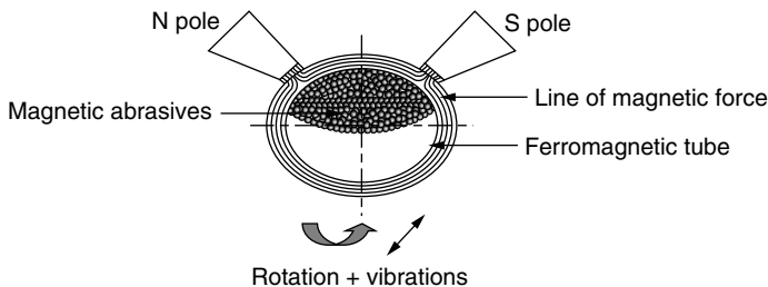
Figure 2.33 Magnetic finishing of magnetic tubes.
