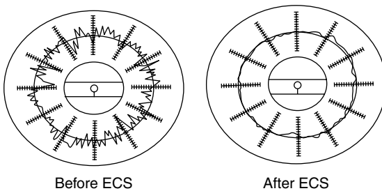
Figure 6.15 Effect of ECS on out-of-roundness profiles.
