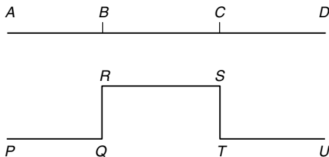
Figure 4.13 Dimensional control in ECM.
