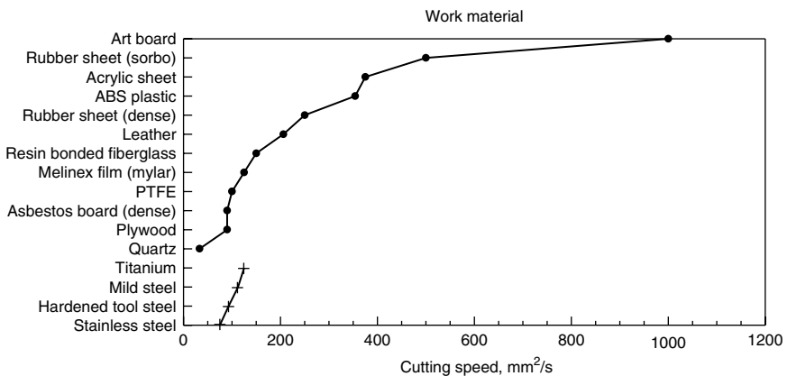
Figure 5.34 Cutting speeds in \text{CO}_2 LBM (El-Hofy, 1995).
