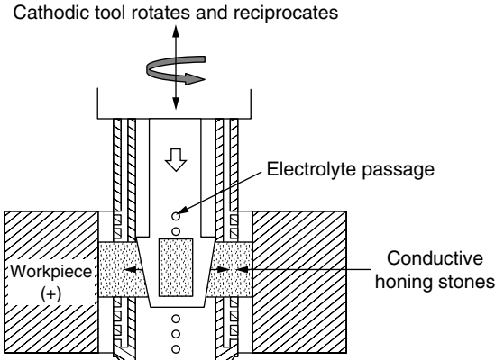
Figure 6.7 ECH schematic.
