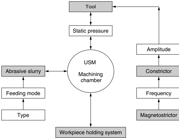
Figure 2.3 USM system components.
