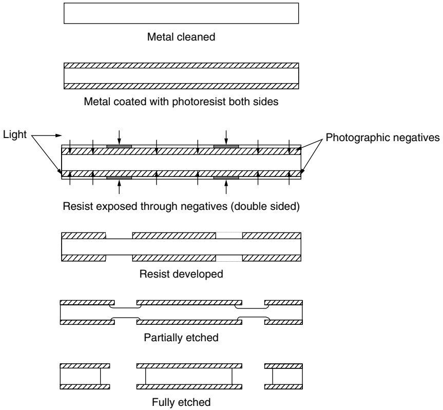
Figure 3.10 PCM steps (Thusty, 1999).
