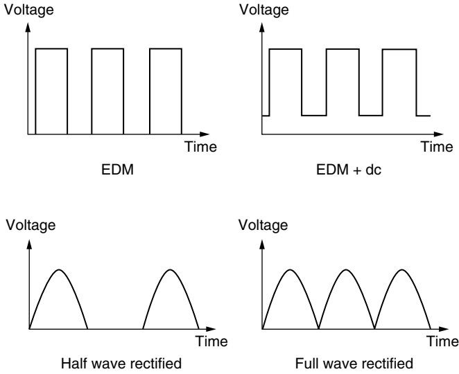
Figure 7.5 Voltage waveforms.
