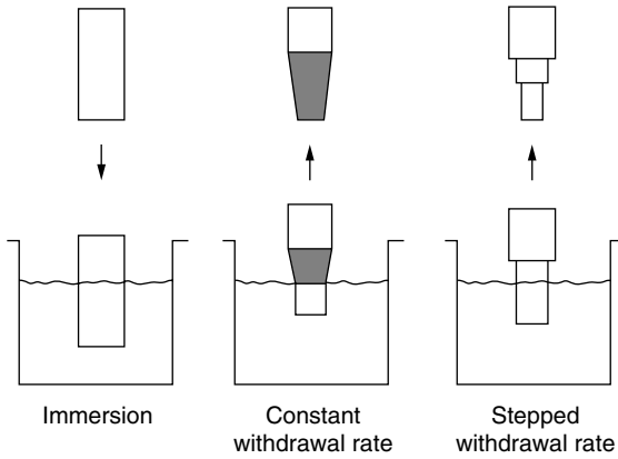
Figure 3.4 Machining tapers and steps by CHM.
