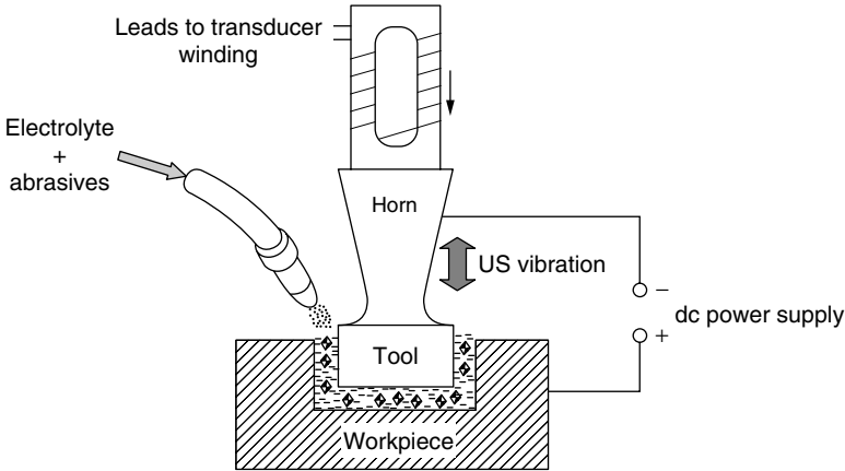
Figure 6.18 USMEC schematic.
