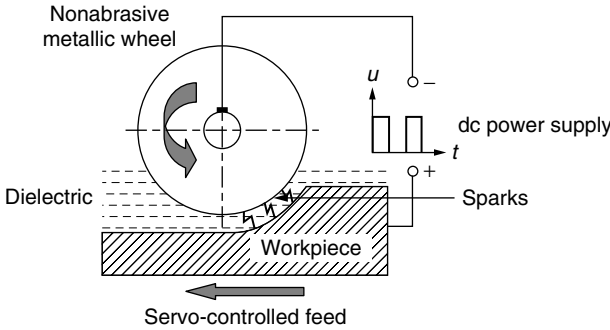
Figure 7.12 EDG schematic.
