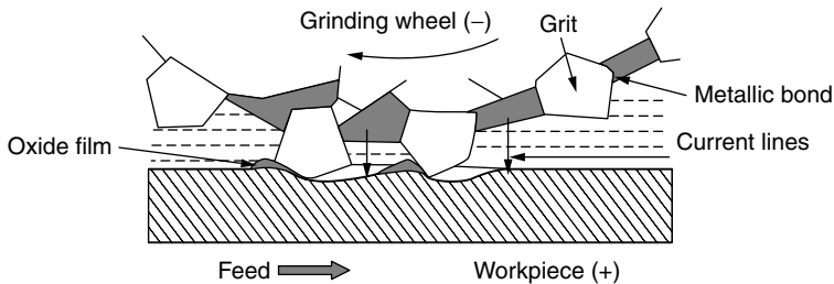
Figure 6.5 ECD and MA in the machining gap during ECG.
