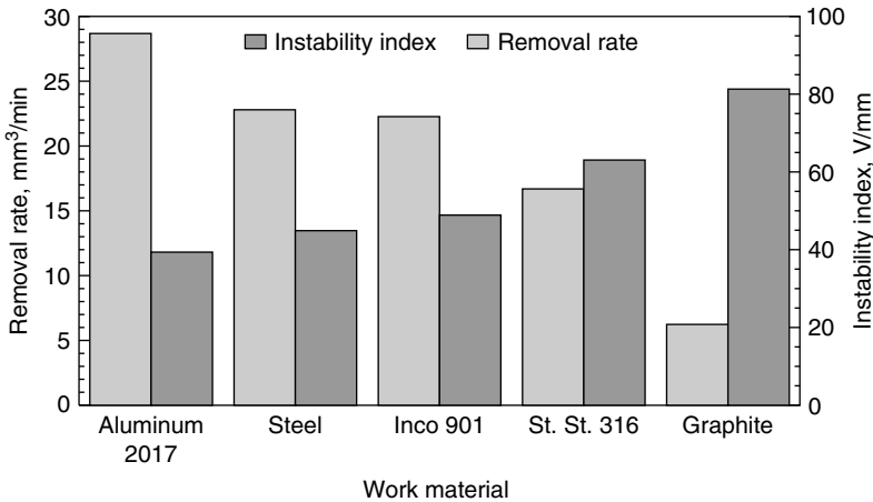
Figure 7.10 Machinability and stability in EEDM (El-Hofy, 1995).
