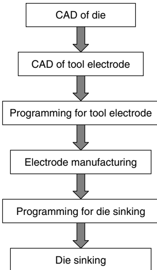
Figure 5.21 EDM die sinking flowchart.
