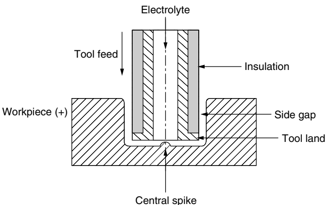
Figure 4.21 ECDR configuration.
