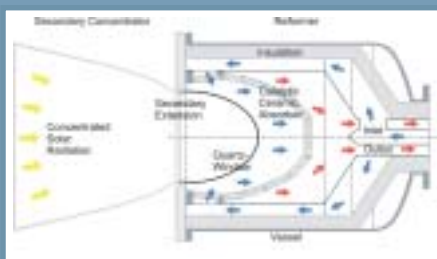
Diagram of the state-of-the-art reformer.
