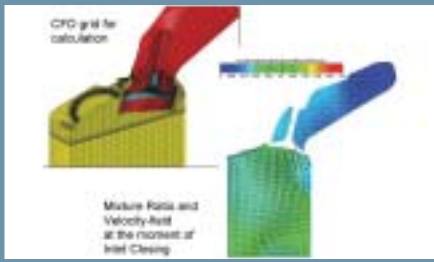
CFD calculation of mixture formation
