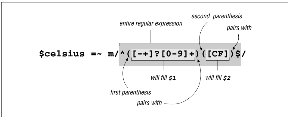
Figure 2-1: Capturing parentheses
