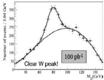
Figure 6: Two jet mass distribution. The fit to the W signal (gaussian) and to the background (Chebyshev polynomial) are indicated.
