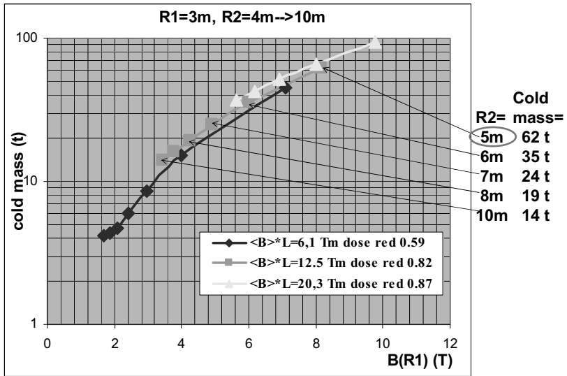
Current density in MgB 2 cable 1kA/mm 2 @ B(R 1 ) ≤ 2T, 1kA/mm 2 × 2/B(R 1 ) @ B(R 1 ) > 2T
