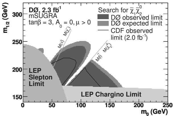
Figure 4: Region excluded by DØ in m_0 - m_{1/2} plane in comparison with the limits from the searches at LEP and CDF.
