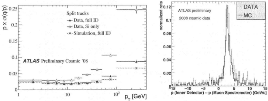
Figure 6: The momentum resolution derived by the cosmic ray split-track method (left), and the evaluation of energy deposited in the calorimeter by comparing the momentum measured in the ID and muon spectrometer (right).
