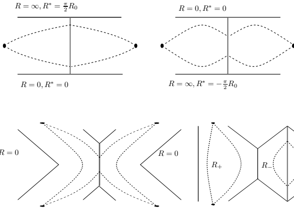
Figure 3: a) \Lambda > 0, k = -1, S_0^0 > 0 b) \Lambda > 0, k = -1, S_0^0 < 0 c) \Lambda < 0, k = +1, S_0^0 > 0 d) \Lambda < 0, k = +1, S_0^0 < 0
