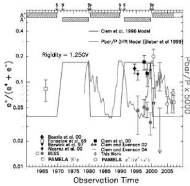
Figure 4: Phenomenological calculations for the positron-electron and antiproton-proton ratios along with the PAMELA and other experimental results.
