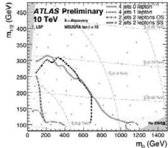
Figure 8: SUSY discovery reach in the plan of universal scalar mass m_0 and universal gaugino mass m_{1/2} .
