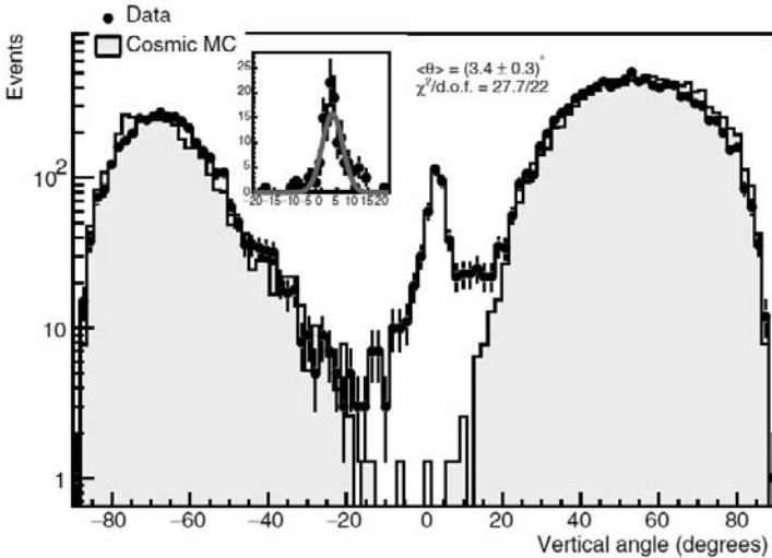
Figure 1: Distribution of the vertical angle of the reconstructed three dimensional tracks using the 2006 data sample. More details are given in the text.
