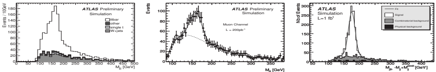
Figure 1: Left: Expected distribution of the three-jet invariant mass in the electron channel mass, normalised to 200 \text{ pb}^{-1} . Middle: The likelihood fit in the three-jet invariant mass for the muon channel. The statistical uncertainties correspond to an integrated luminosity of 200 \text{ pb}^{-1} . Right: Hadronic top mass for semileptonic events after purification cuts.
