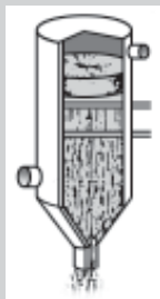
Gambar 11.12 Filter basah
