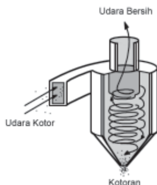
Gambar 11.8 Filter udara
