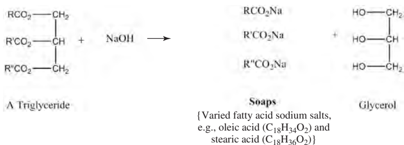
FIGURE 5.2.1.2 Saponification of a Triglyceride. Treating a fat with a strong base frees fatty acids that can be isolated as sodium salts that can be used as soaps.
