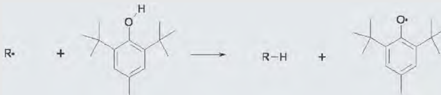
FIGURE 5.3.2.3 BHT Radical Reaction. BHT scavenges alkyl radicals, and the BHT radical is very stable and unreactive.
