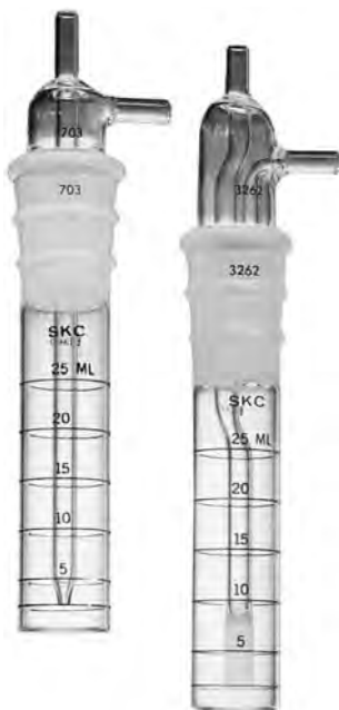
FIGURE 6.3.1.2 An Impinger for Air Sampling. The bottom portion of the impinger is filled with a measured quantity of a liquid. The air sample is drawn into the liquid from the opening at the top by using reduced pressure at the side port. The impinger on the right has a sintered glass attachment at the bottom, which creates many small bubbles in the air and optimizes the air-liquid interface. (Courtesy of SKC, Inc., Eighty Four, PA.)
