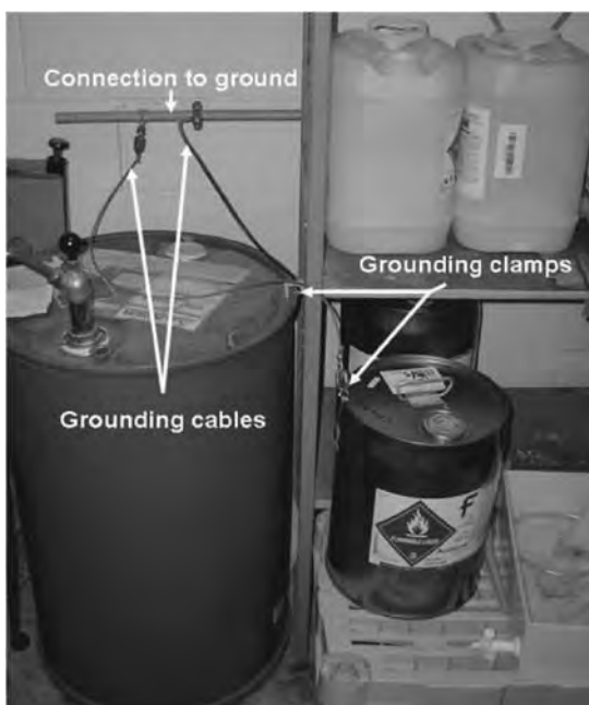
FIGURE 5.1.2.3 Proper Grounding for Metal Solvent Drum. Spring-loaded clips make it easy to connect a metal container to a grounded metal pipe.
